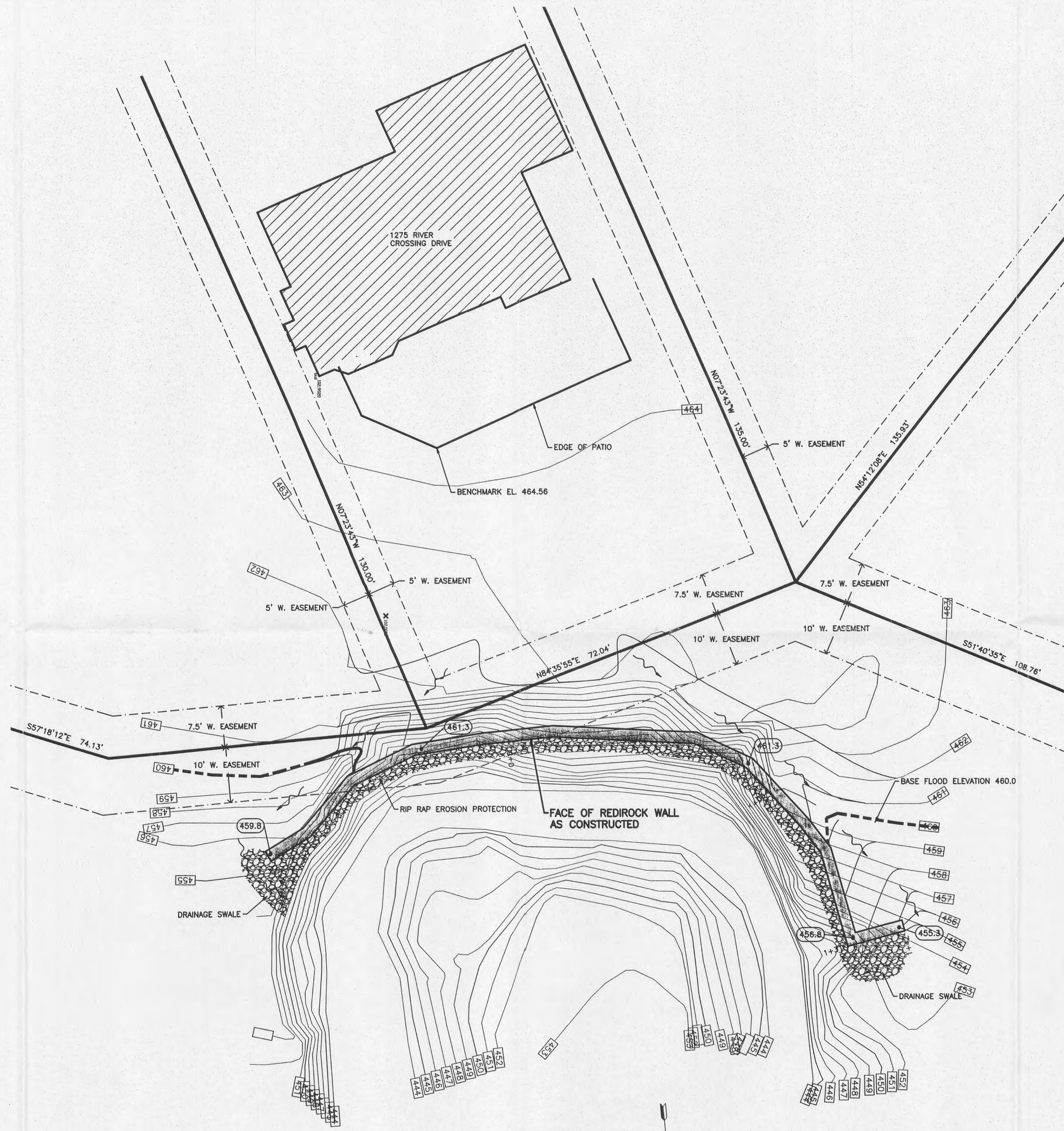
AS-BUILT PLAN VIEW SCALE 1"=10'
