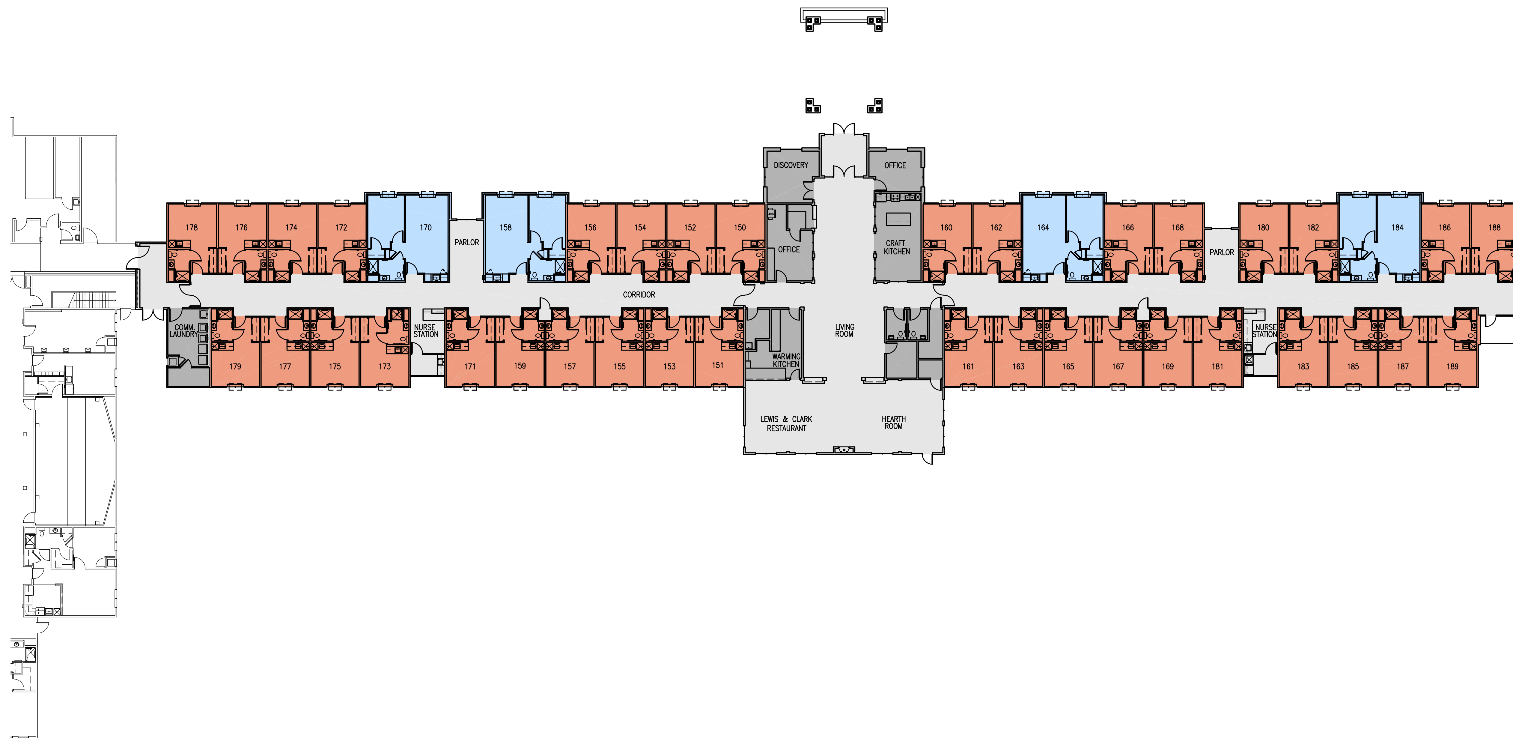
FIRST FLOOR OVERALL PLAN SCALE 1/16" = 1' - 0"
