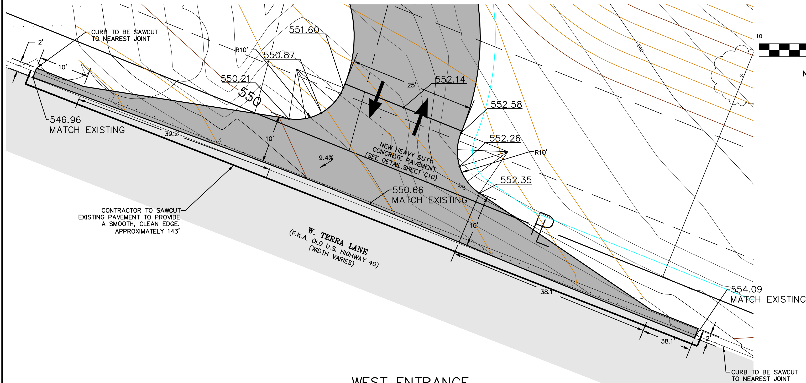
WEST ENTRANCE WARPING DETAIL
