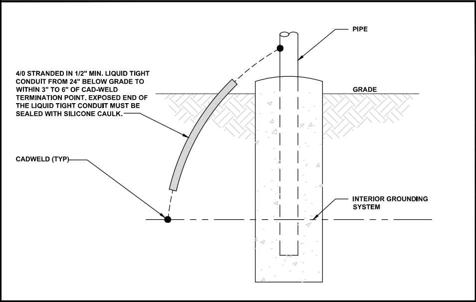
TRANSITIONING GROUND DETAIL NO SCALE 4
