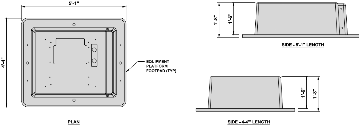
PLATFORM DETAIL
