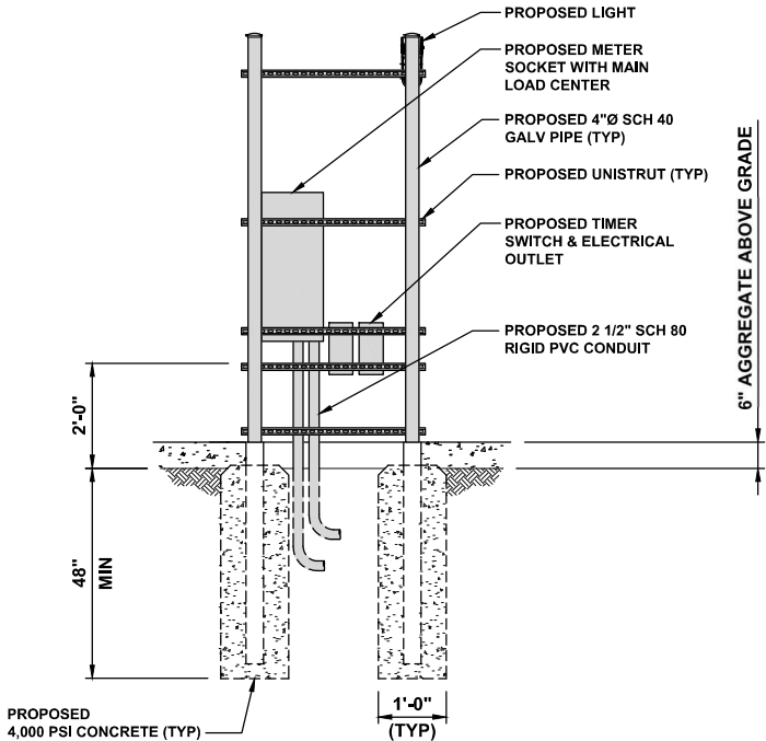
BACK ELEVATION
