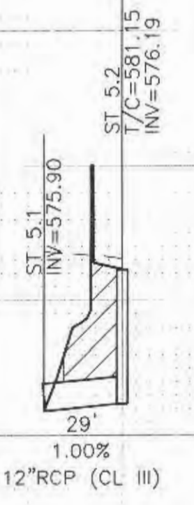
STORM SEWER 5 (PRIVATE)
