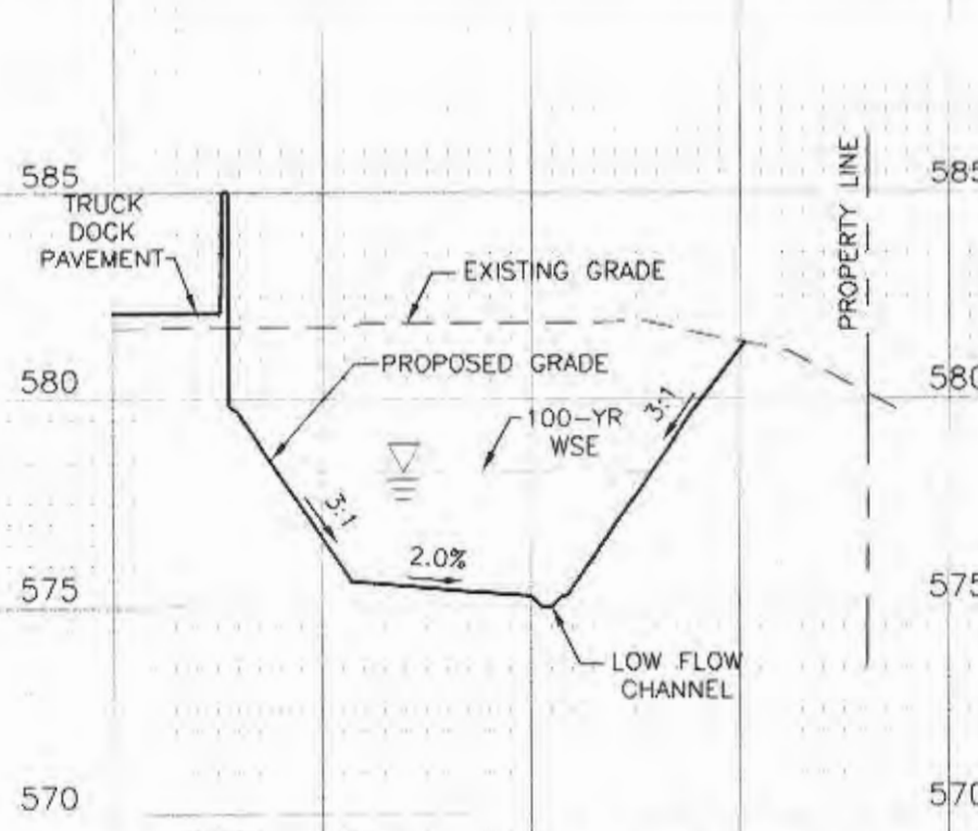
BASIN CROSS SECTION A-A
