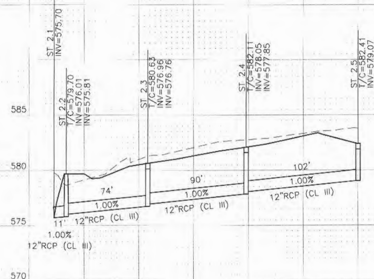
STORM SEWER 2 (PRIVATE)
