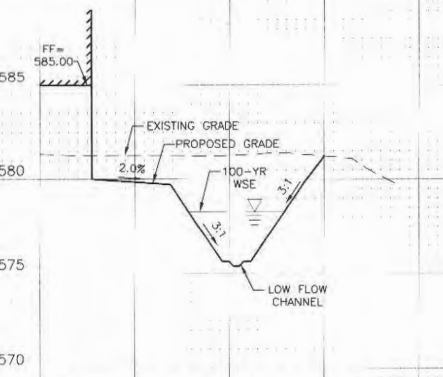
BASIN CROSS SECTION B-B
