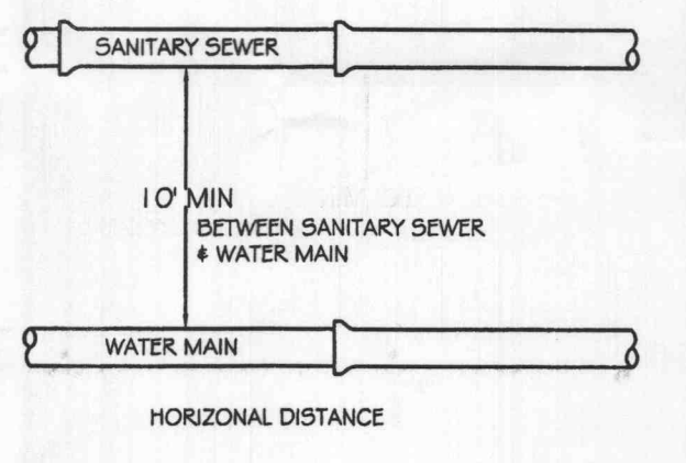
TYPICAL WATER & SEWER SEPARATION N.T.S.
