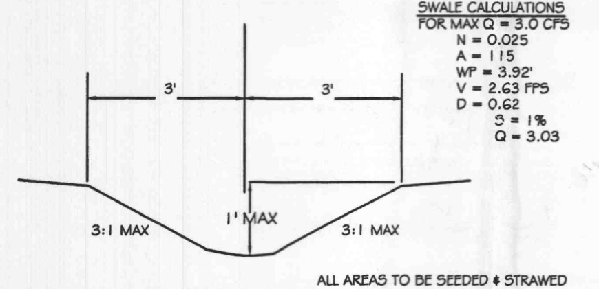
TYPICAL GRASS SWALE N.T.S.
