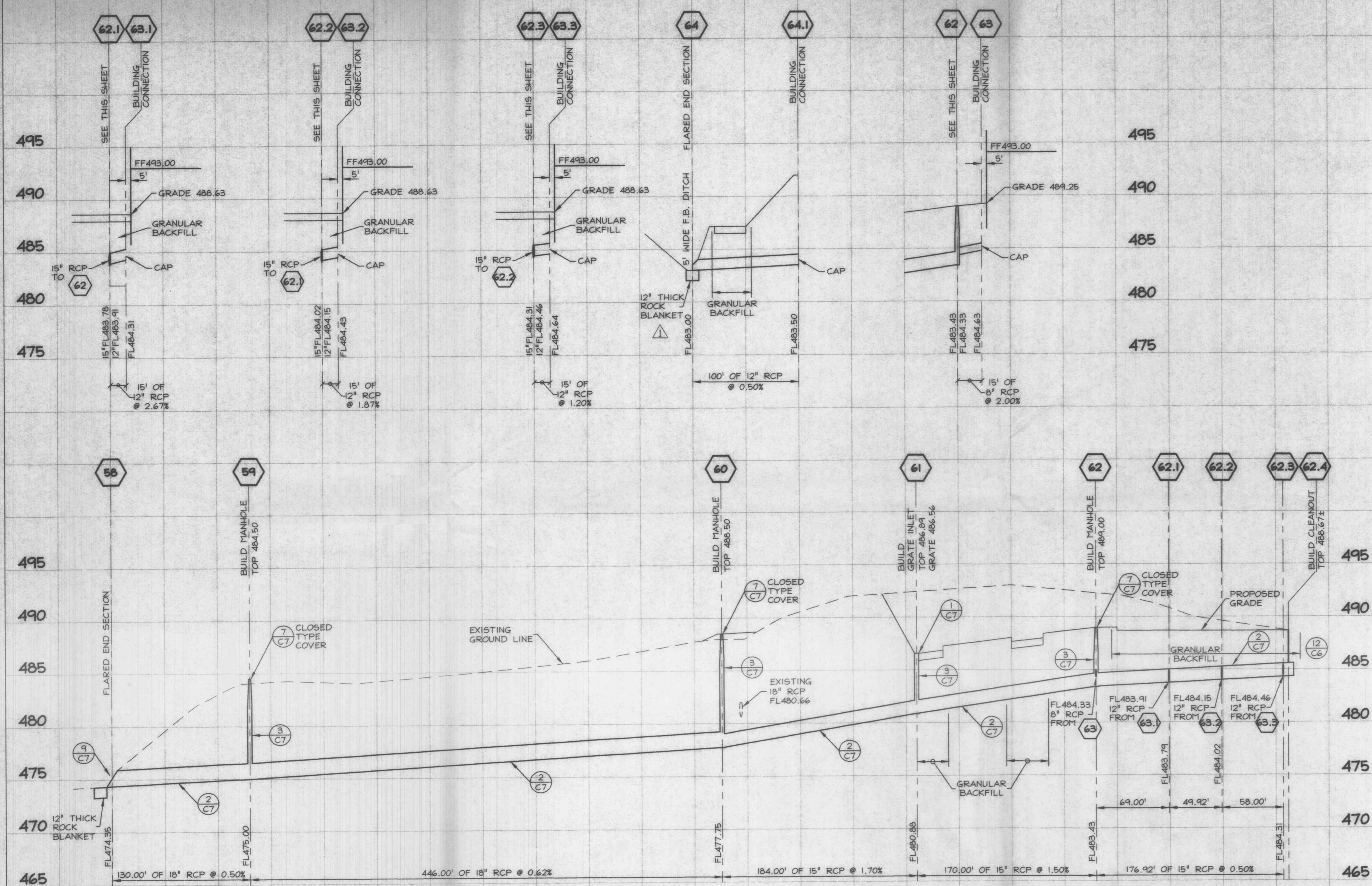
WAREHOUSE STORM SEWER PROFILES SCALE: 1" = 50'HORIZ. 1" = 5'VERT.
