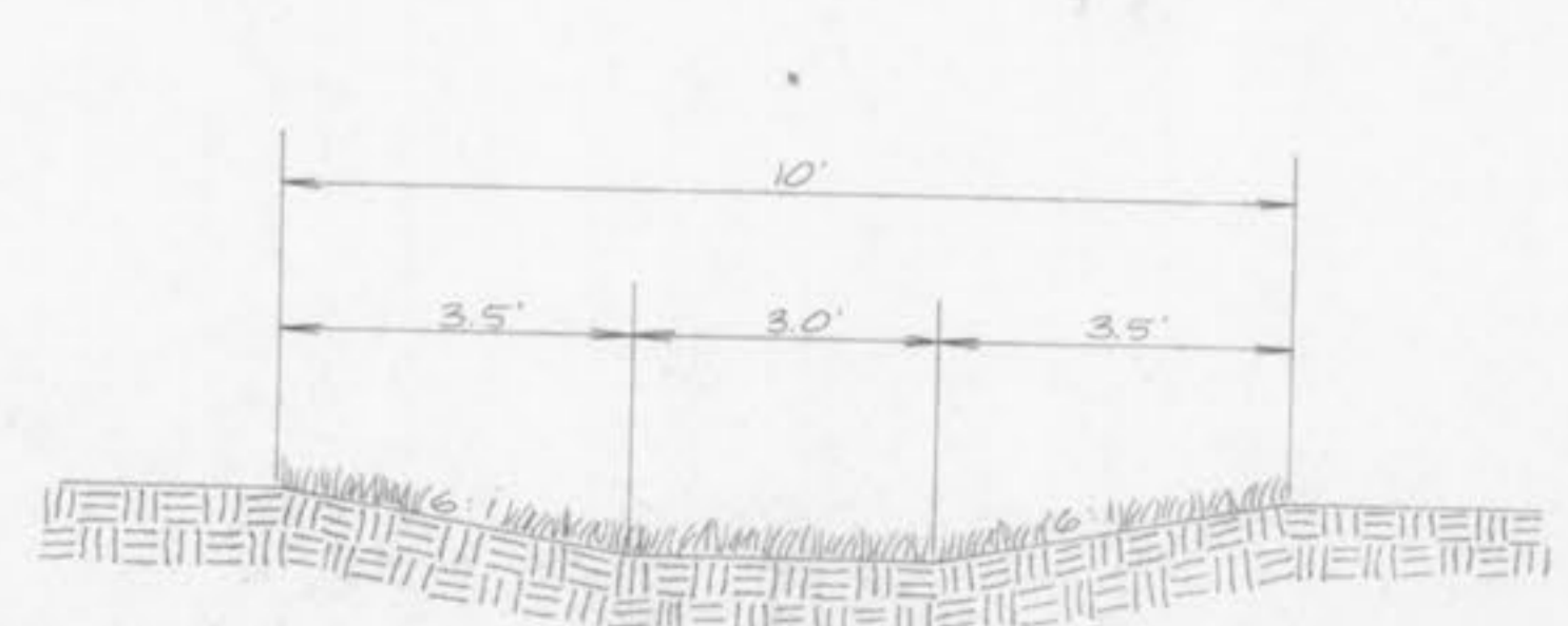
TYPICAL EMERGENCY RELIEF SWALE (THRU WALK-OUT TERRACE) CHANNEL WIDTH 3'-0"
