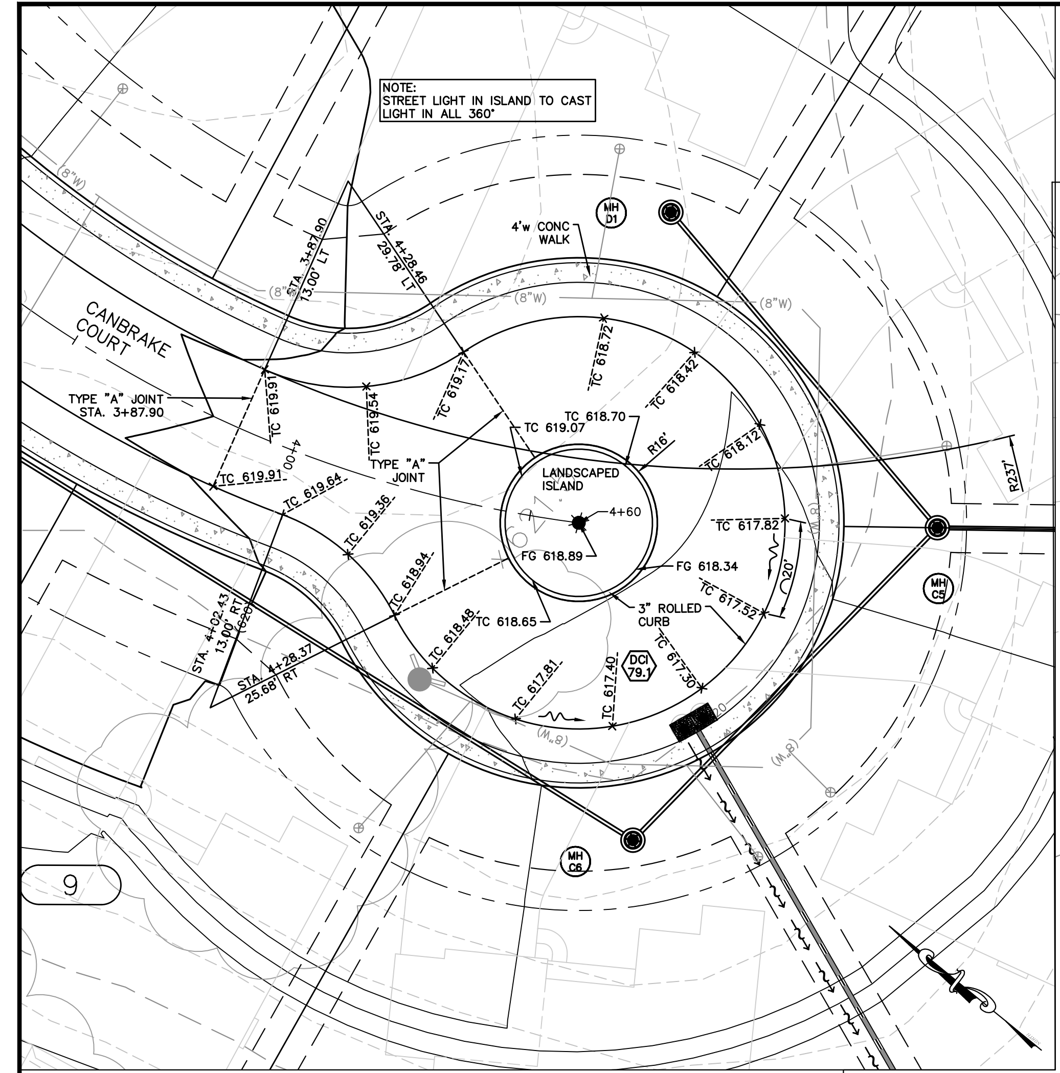
CANBRAKE COURT CUL-DE-SAC SCALE: 1"=20'
