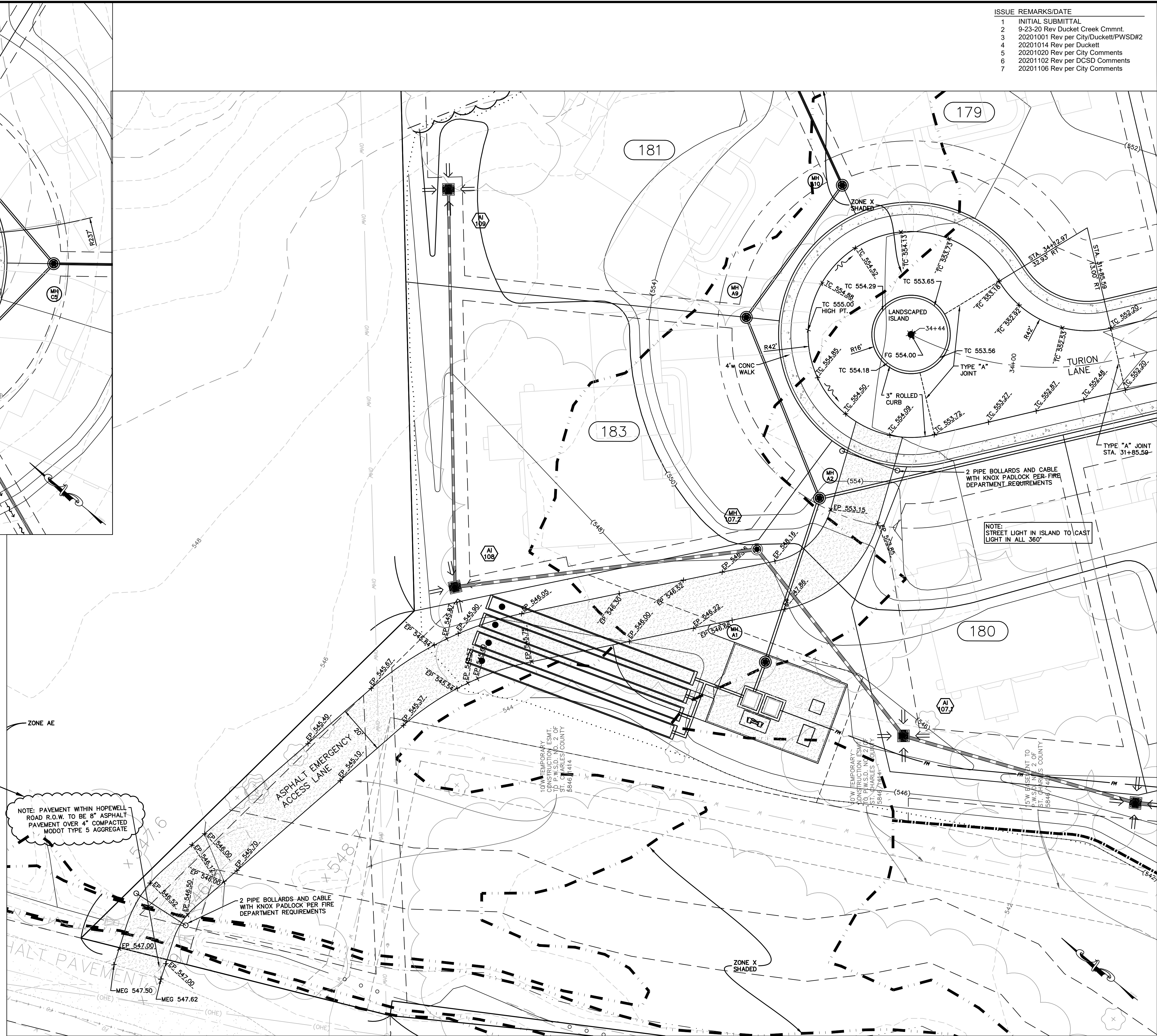
TURION LANE & EMERGENCY ACCESS LANE SCALE: 1"=20'
