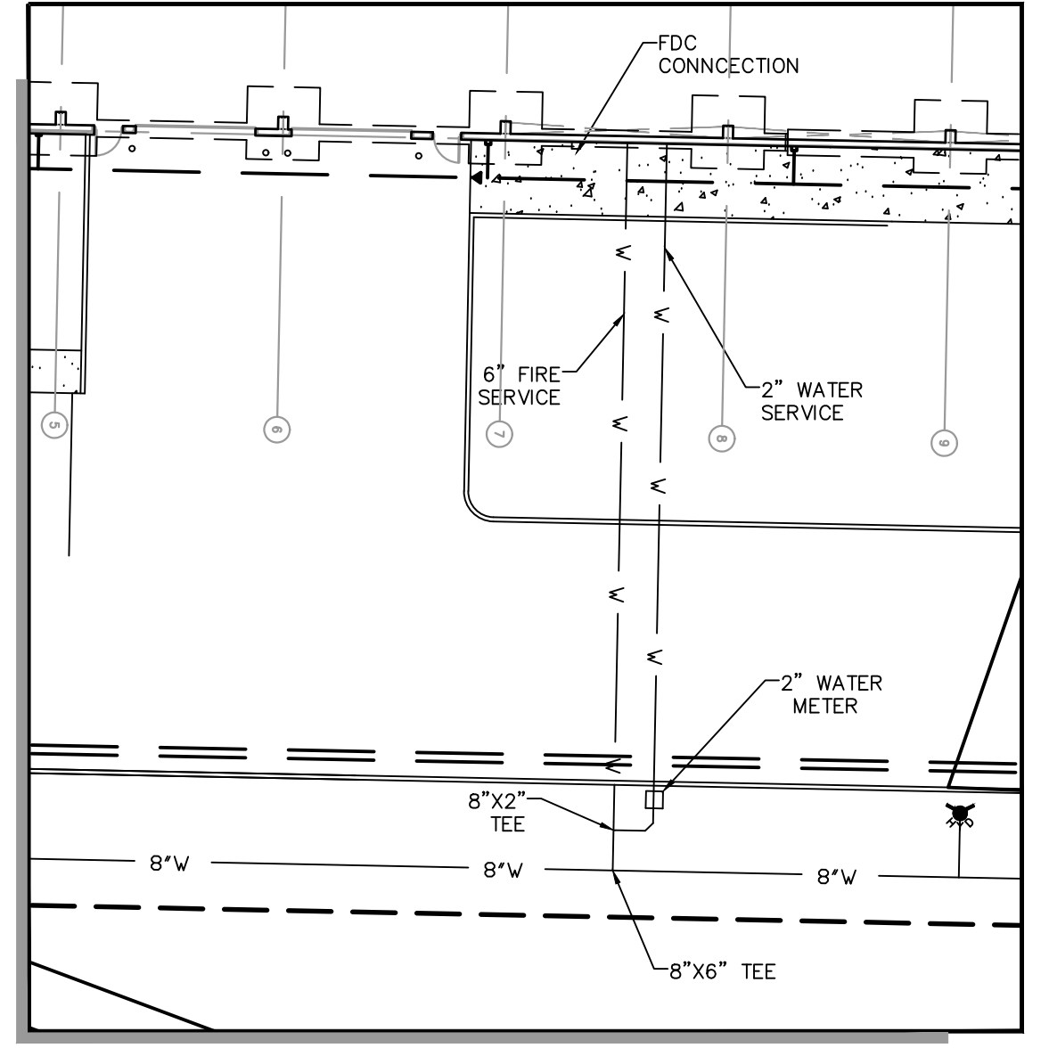
WATER SERVICE DETAIL
