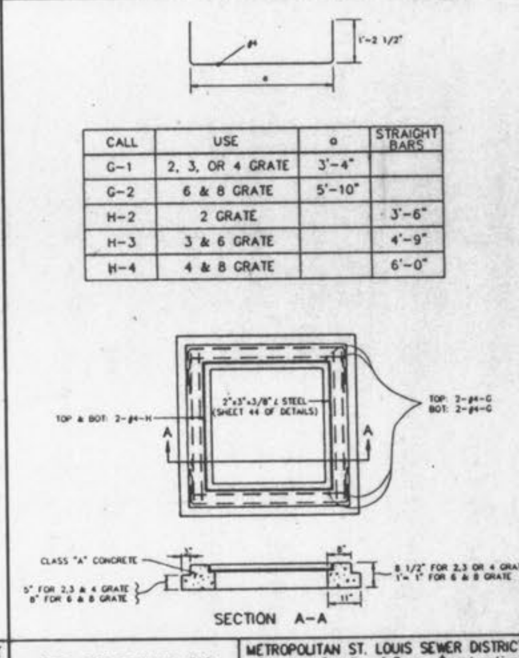
STEEL REQUIREMENTS FOR GRATE INLET SEAT METROPOLITAN ST. LOUIS SEWER DISTRICT Standard Details of Sewer Construction Dr. W.S.H. 1992 SHEET 46
