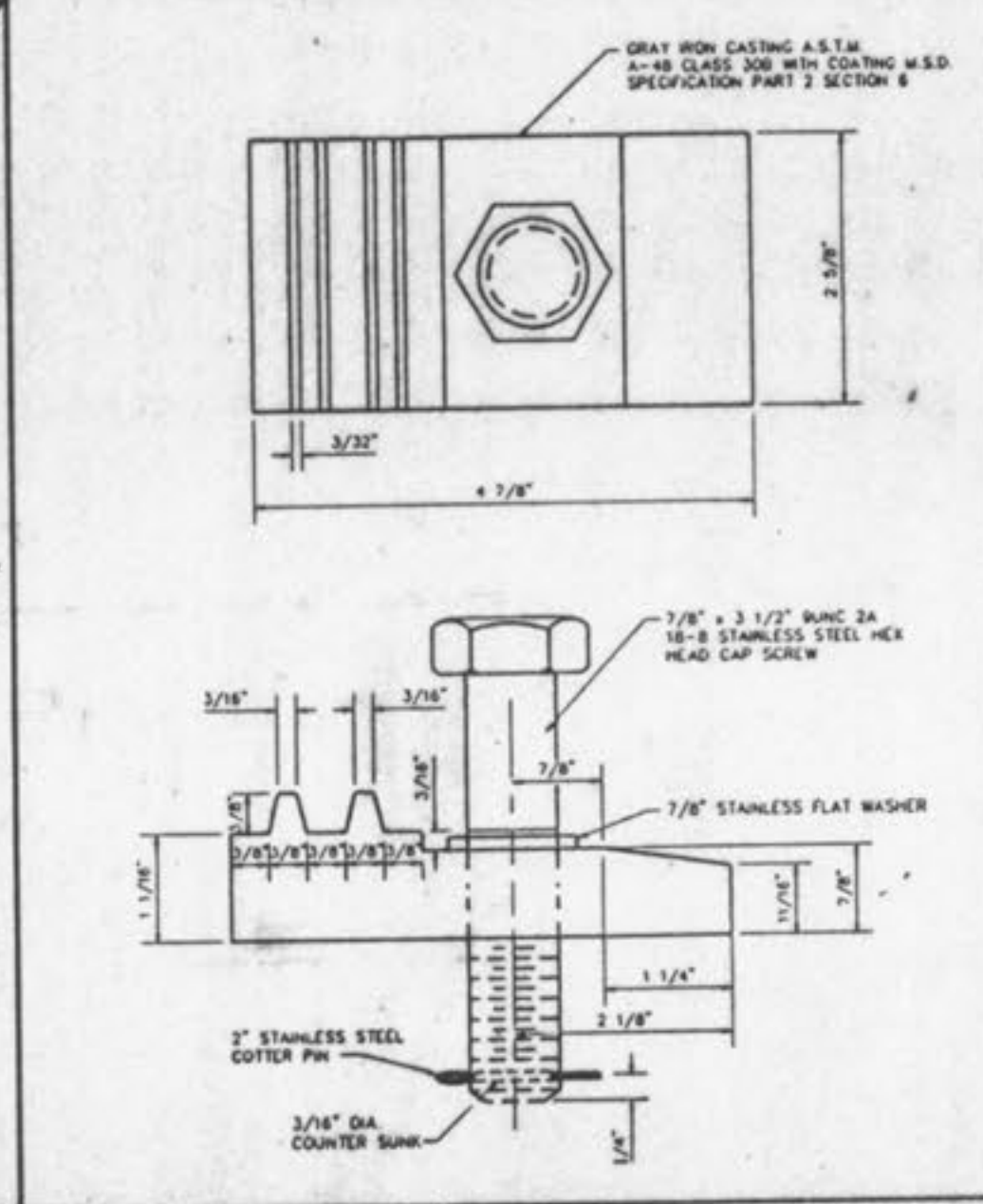
LOCKING DEVICE FOR TYPE 'T' LOCK TYPE MANHOLE COVER METROPOLITAN ST. LOUIS SEWER DISTRICT Standard Details of Sewer Construction Dr. R.C.W. 1992 SHEET 51
