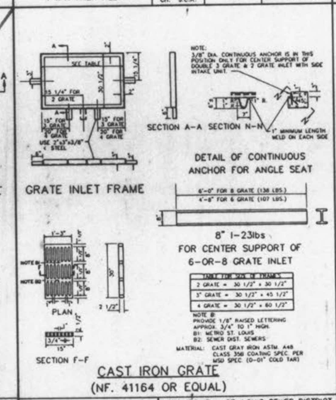
DETAILS OF INLET FRAME AND GRATES METROPOLITAN ST. LOUIS SEWER DISTRICT Standard Details of Sewer Construction Dr. R.C.W. 1992 SHEET 44
