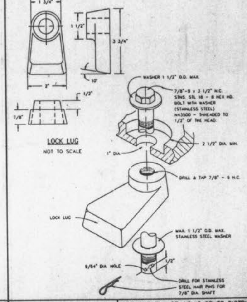
LOCKING DEVICE FOR TYPE 'N' LOCK TYPE MANHOLE COVER METROPOLITAN ST. LOUIS SEWER DISTRICT Standard Details of Sewer Construction Dr. J.L.G. 1992 SHEET 52
