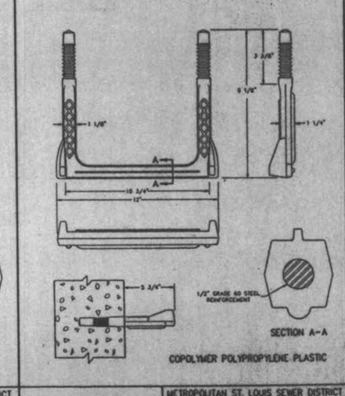
MANHOLE STEP FOR PRECAST MANHOLE METROPOLITAN ST. LOUIS SEWER DISTRICT Standard Details of Sewer Construction Dr. D.A.B. 1992 SHEET 54
