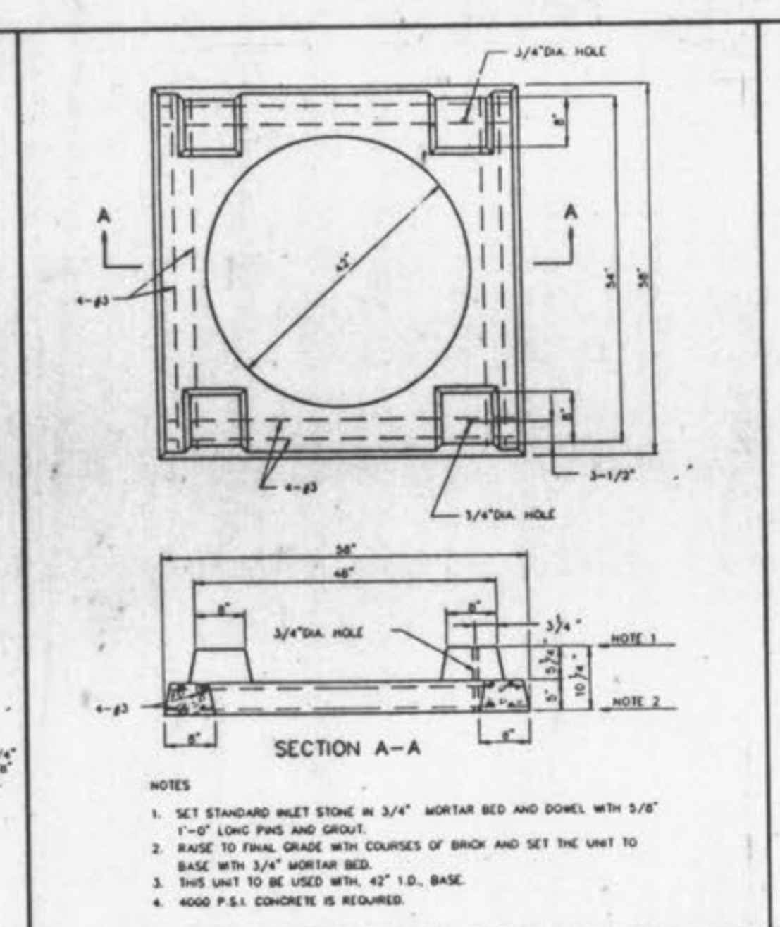
PRE-CAST CONCRETE UNIT FOR 4 WAY AREA INLET METROPOLITAN ST. LOUIS SEWER DISTRICT Standard Details of Sewer Construction Dr. D.A.B. 1992 SHEET 38
