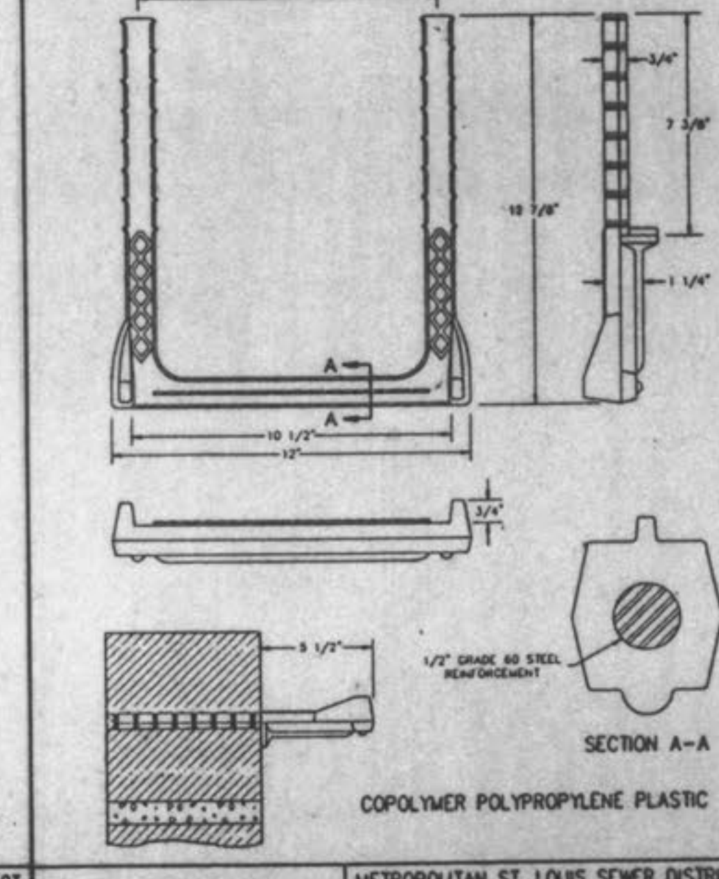
PSI-B MANHOLE STEP INTO JOINT METROPOLITAN ST. LOUIS SEWER DISTRICT Standard Details of Sewer Construction Dr. W.S.H. 1992 SHEET 53
