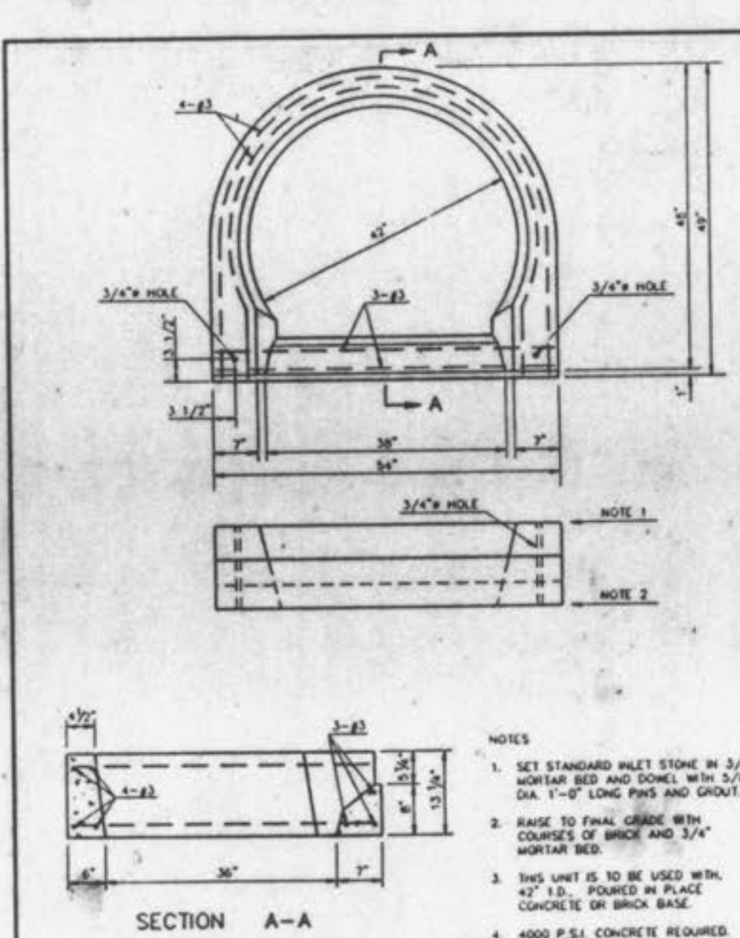
PRE-CAST CONCRETE UNIT FOR SINGLE STREET INLET METROPOLITAN ST. LOUIS SEWER DISTRICT Standard Details of Sewer Construction Dr. W.S.H. 1992 SHEET 37
