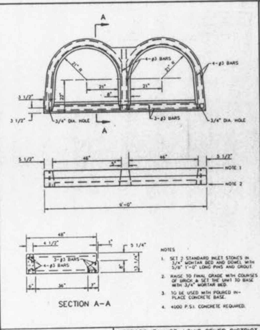
PRE-CAST CONCRETE UNIT A FOR STREET DOUBLE INLET METROPOLITAN ST. LOUIS SEWER DISTRICT Standard Details of Sewer Construction Dr. R.C.W. 1992 SHEET 40
