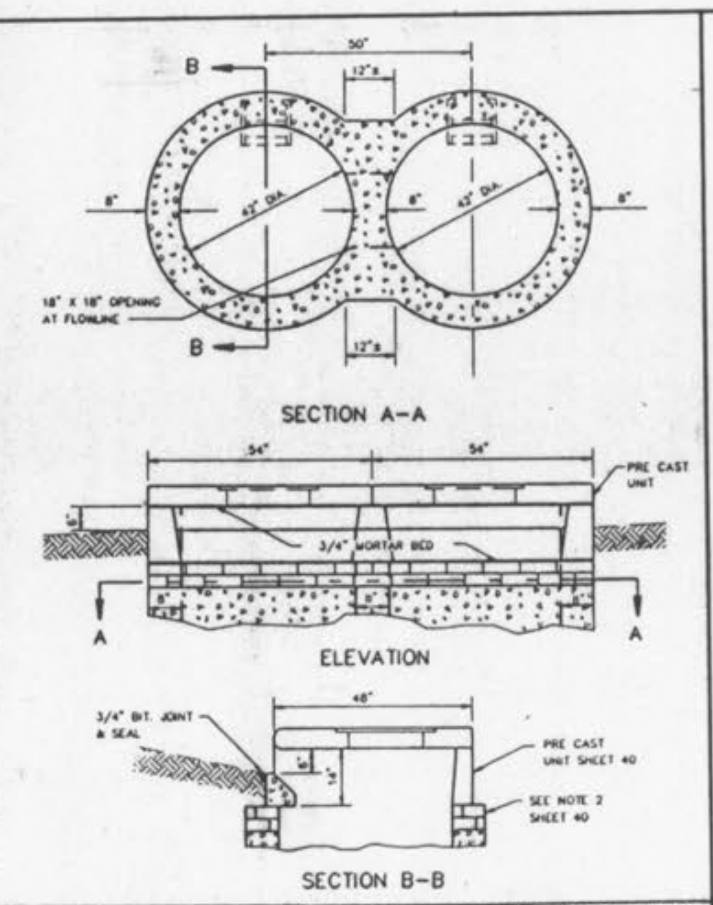
CONCRETE DOUBLE STREET INLET W/PRE CAST CONCRETE UNIT A METROPOLITAN ST. LOUIS SEWER DISTRICT Standard Details of Sewer Construction Dr. R.C.W. 1992 SHEET 39
