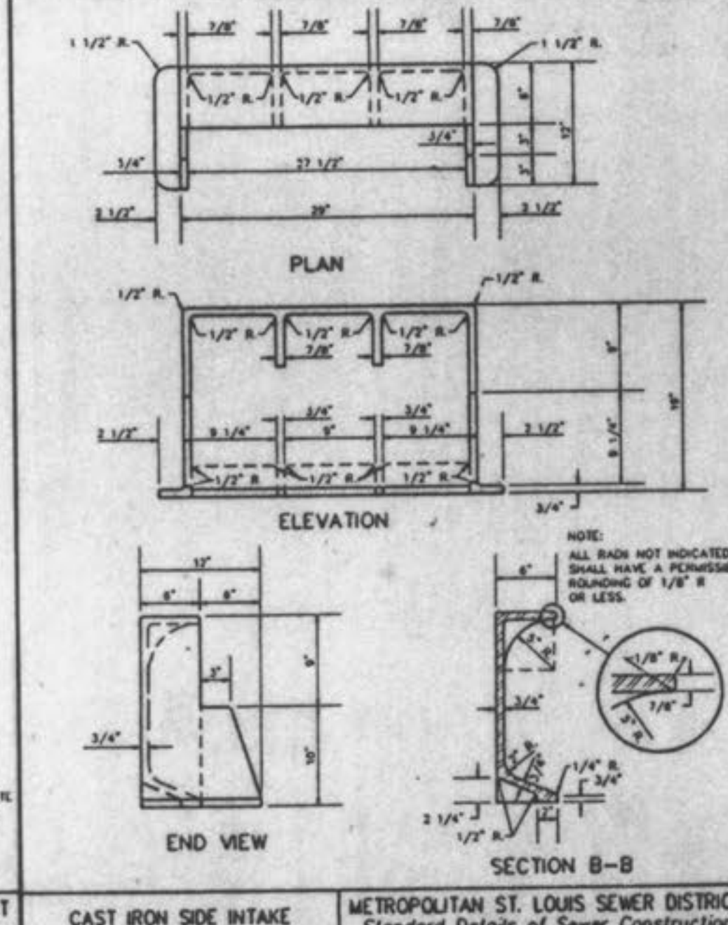
CAST IRON SIDE INTAKE UNIT FOR GRATED INLETS 249 LBS. METROPOLITAN ST. LOUIS SEWER DISTRICT Standard Details of Sewer Construction Dr. R.C.W. 1992 SHEET 47
