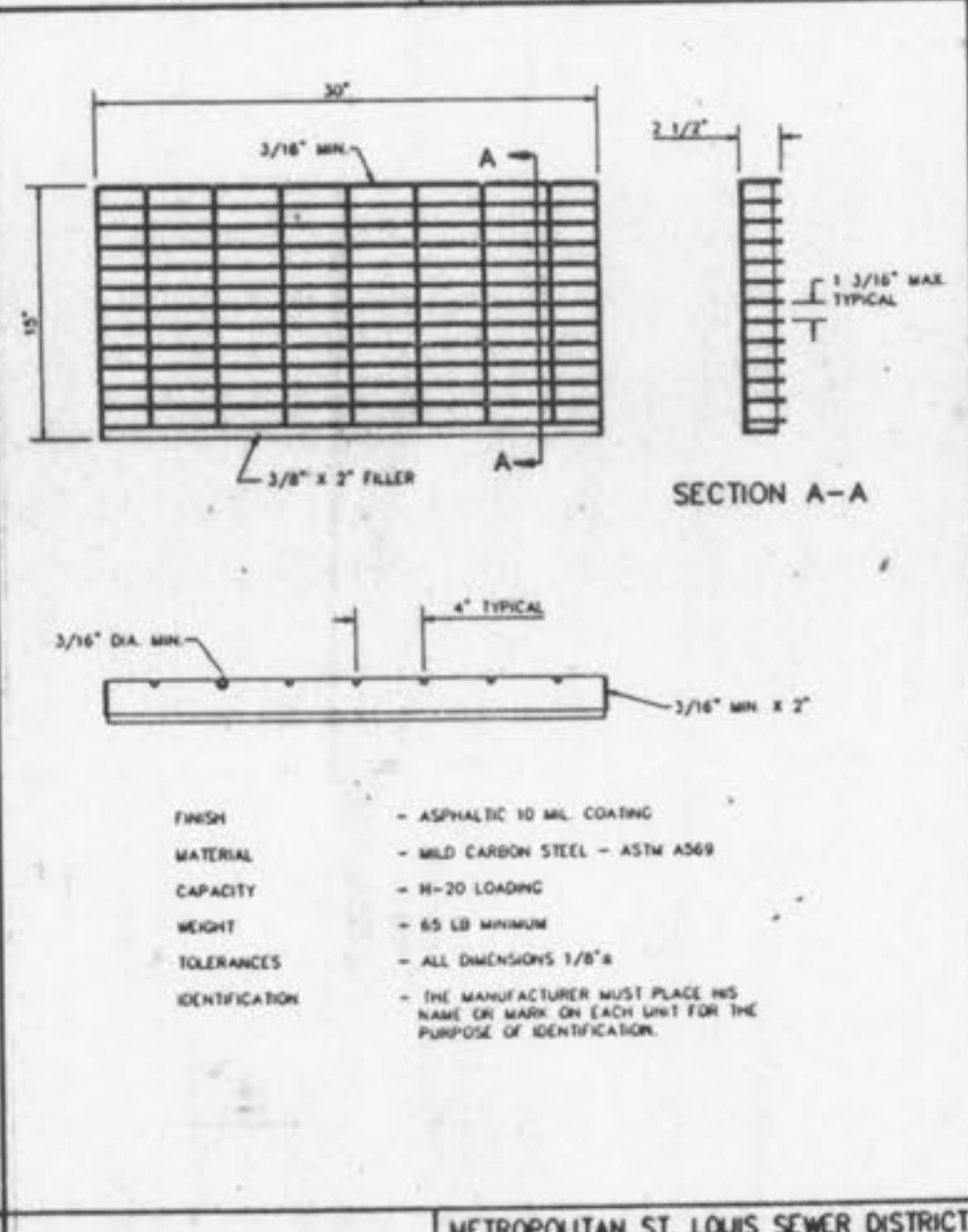
DETAIL OF STEEL GRATE METROPOLITAN ST. LOUIS SEWER DISTRICT Standard Details of Sewer Construction Dr. R.C.W. 1992 SHEET 45
