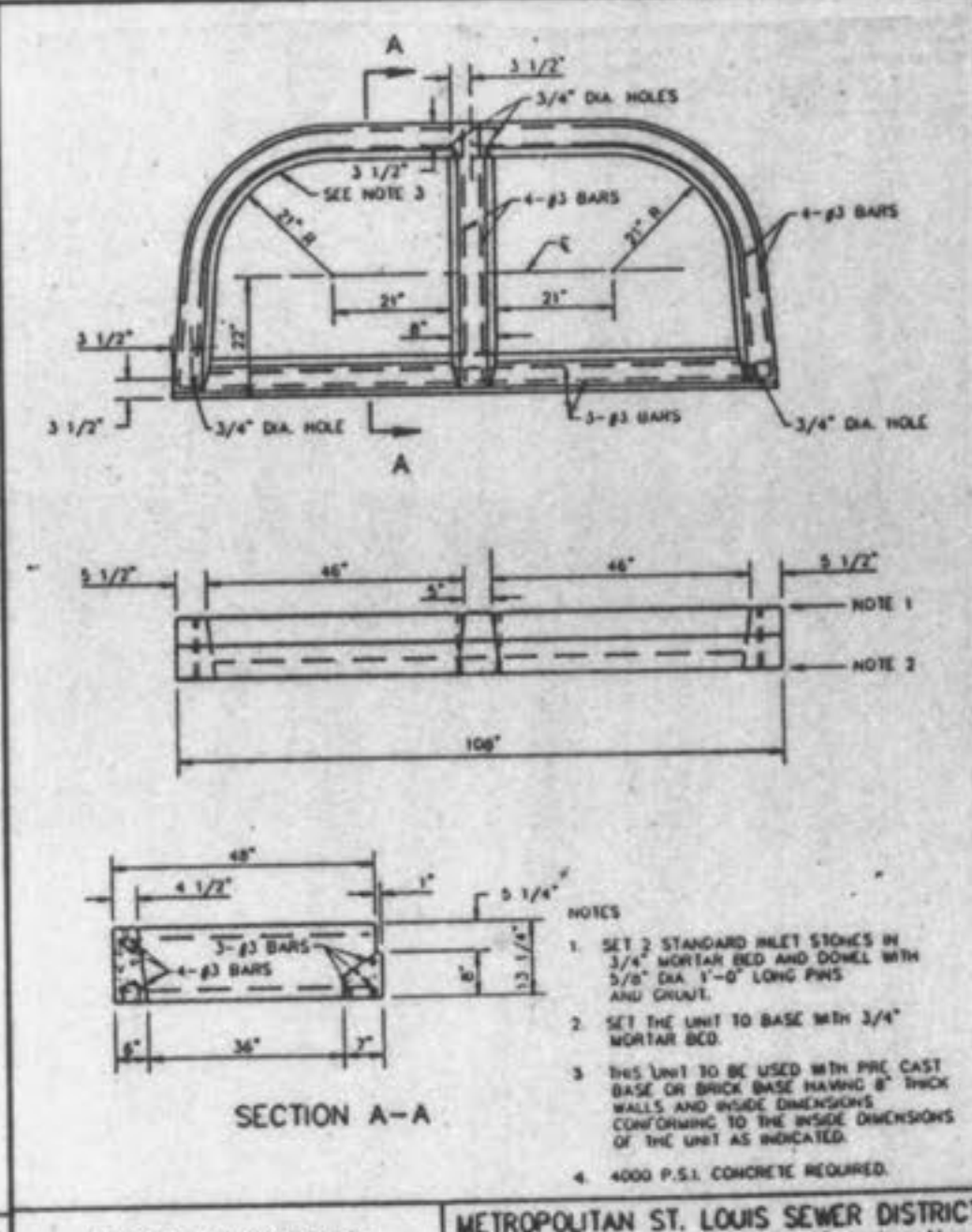
PRE-CAST CONCRETE UNIT B FOR STREET DOUBLE INLET METROPOLITAN ST. LOUIS SEWER DISTRICT Standard Details of Sewer Construction Dr. R.C.W. 1992 SHEET 41
