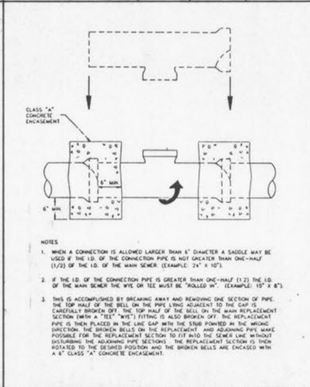
"ROLL-IN" (FOR EXISTING CLAY OR CONCRETE PIPE) METROPOLITAN ST. LOUIS SEWER DISTRICT Standard Details of Sewer Construction Dr. D.A.B. 1992 SHEET 63 Ch. J.C.K.
