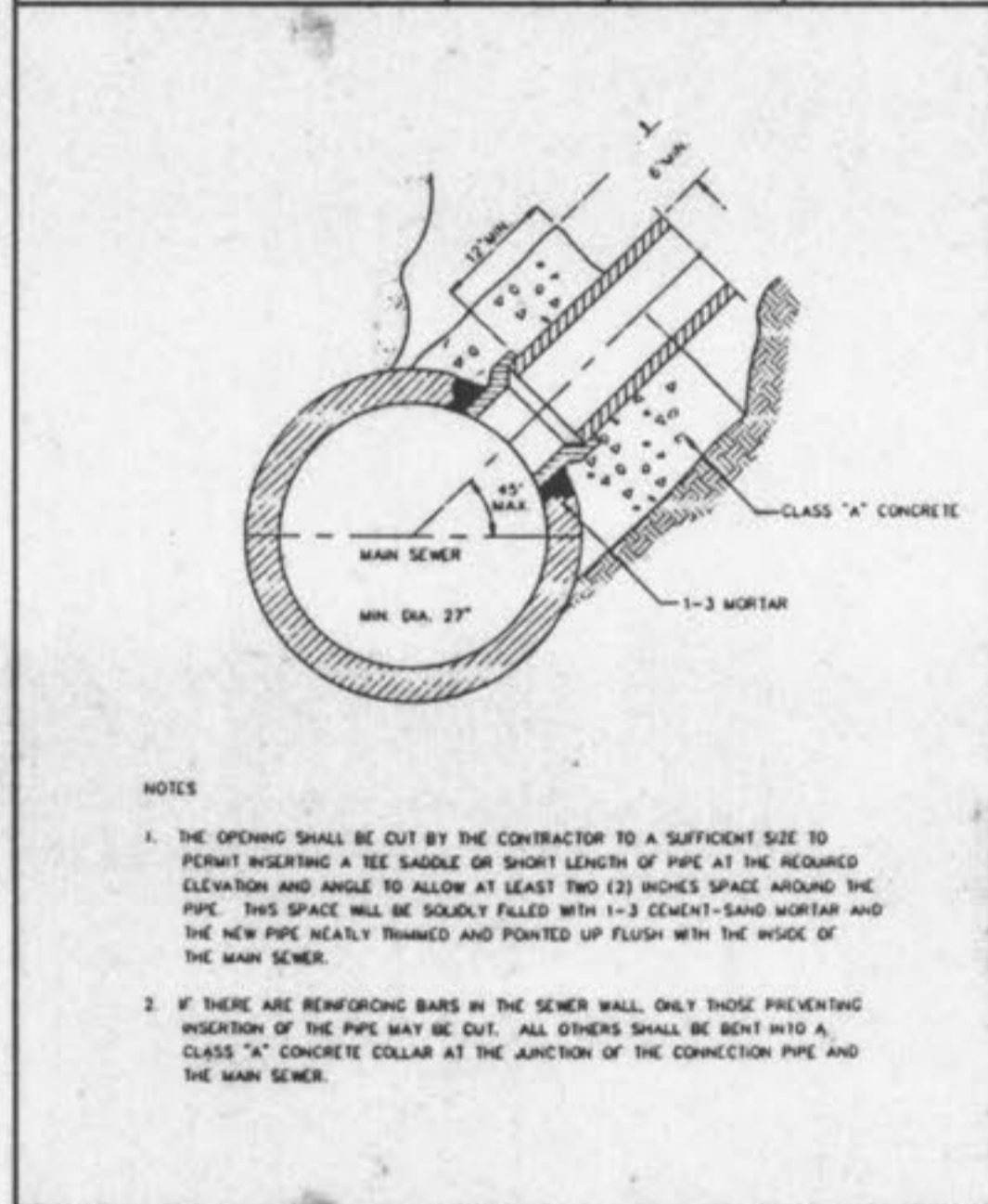
HOUSE CONNECTIONS ALLOWED BY TEE SADDLE METROPOLITAN ST. LOUIS SEWER DISTRICT Standard Details of Sewer Construction Dr. D.A.B. 1992 SHEET 61 Ch. J.C.K.
