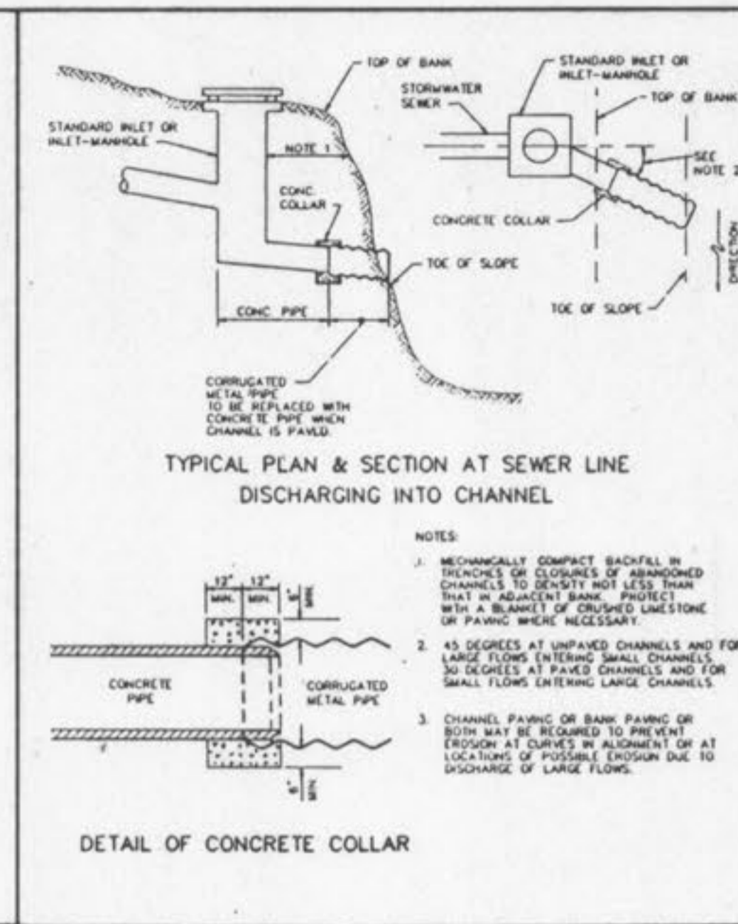
STORMWATER CHANNELS METROPOLITAN ST. LOUIS SEWER DISTRICT Standard Details of Sewer Construction Dr. R.G.W. 1992 SHEET 58 Ch. J.C.K.
