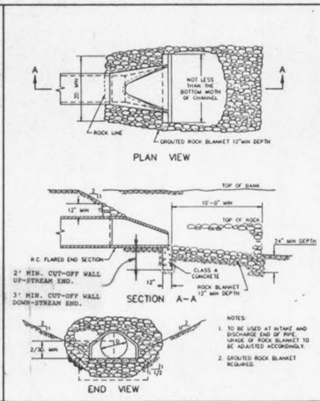
FLARED END SECTION METROPOLITAN ST. LOUIS SEWER DISTRICT Standard Details of Sewer Construction Dr. W.S.H. 1992 SHEET 57 Ch. J.C.K.
