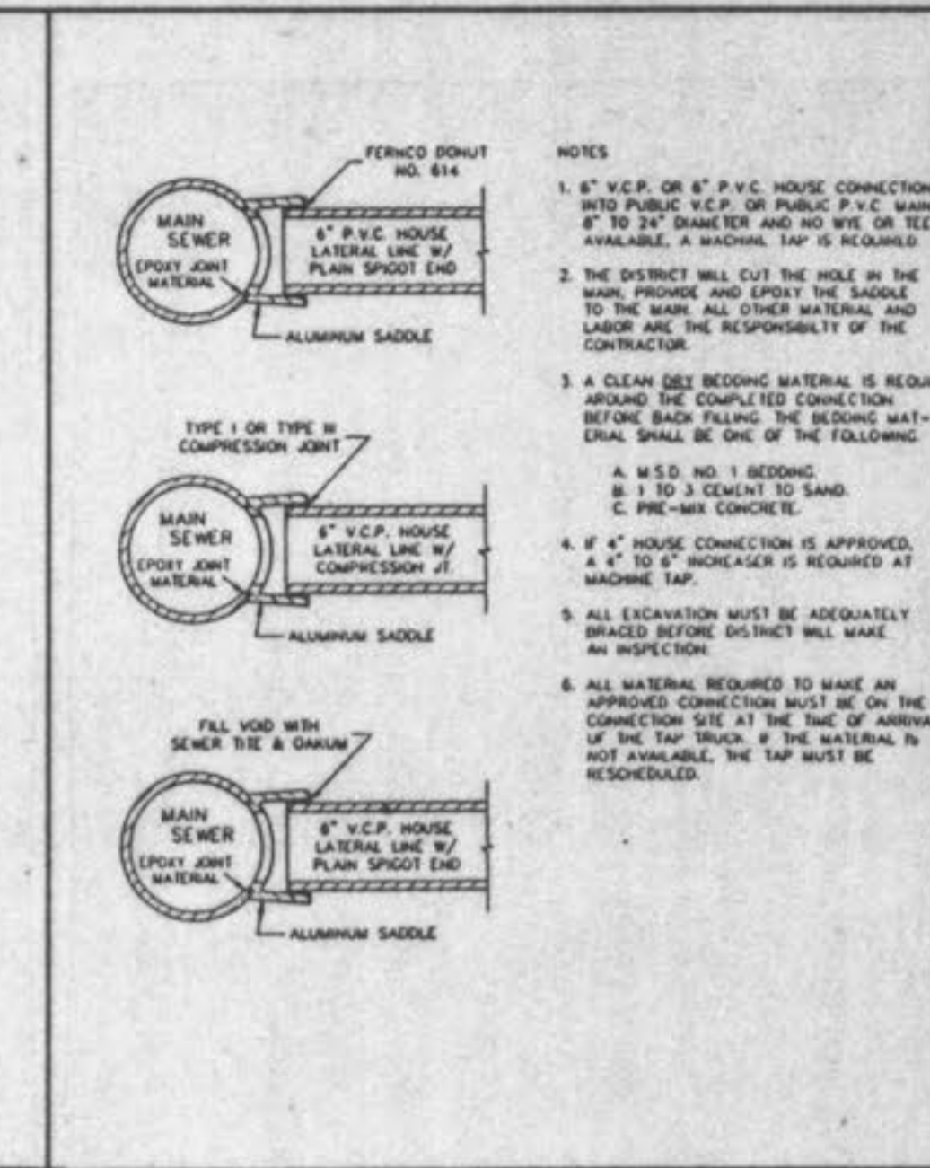
MACHINE TAP METROPOLITAN ST. LOUIS SEWER DISTRICT Standard Details of Sewer Construction Dr. W.S.H. 1992 SHEET 60 Ch. J.C.K.
