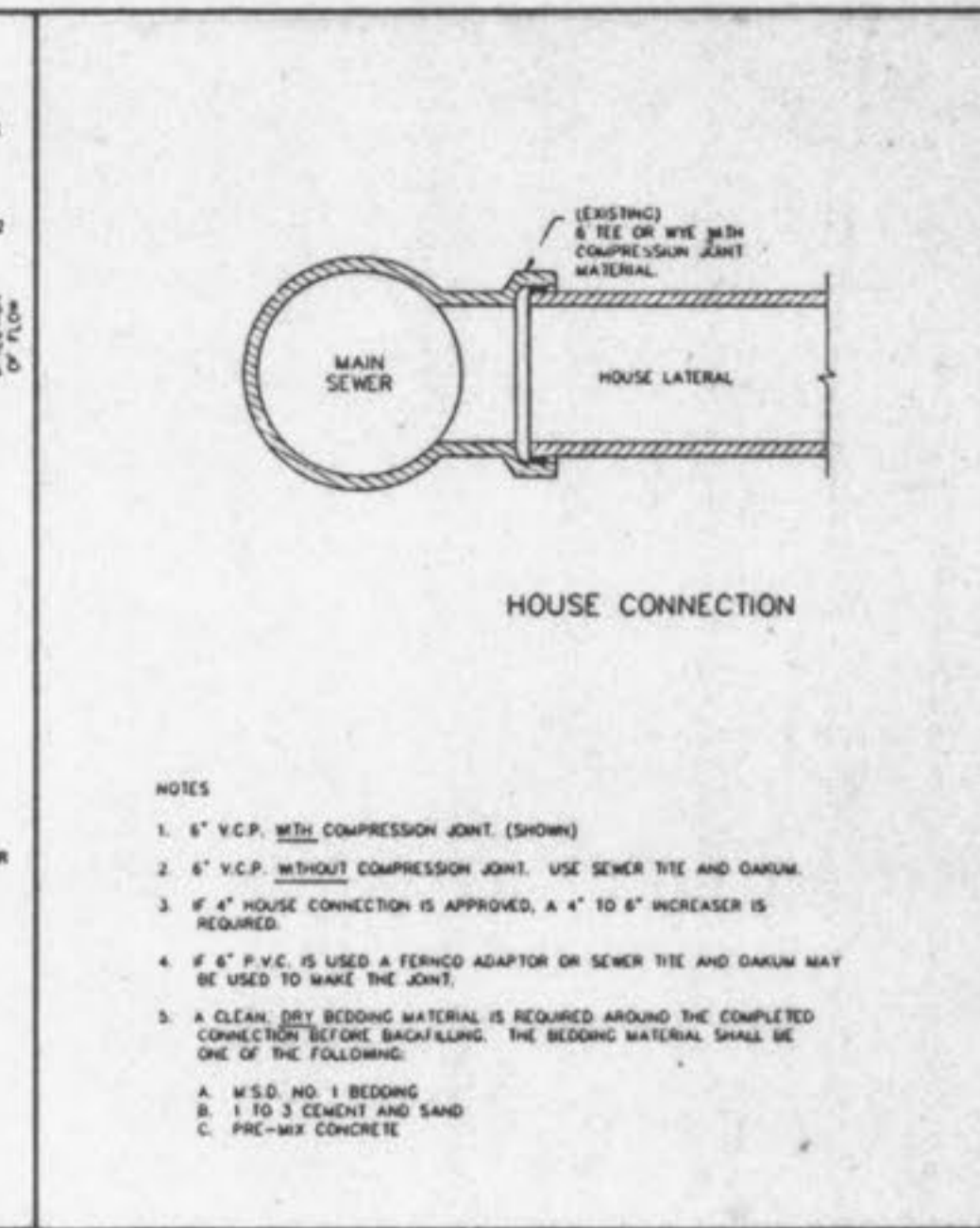
HOUSE CONNECTION TO EXISTING TEE OR WYE METROPOLITAN ST. LOUIS SEWER DISTRICT Standard Details of Sewer Construction Dr. D.A.B. 1992 SHEET 59 Ch. J.C.K.
