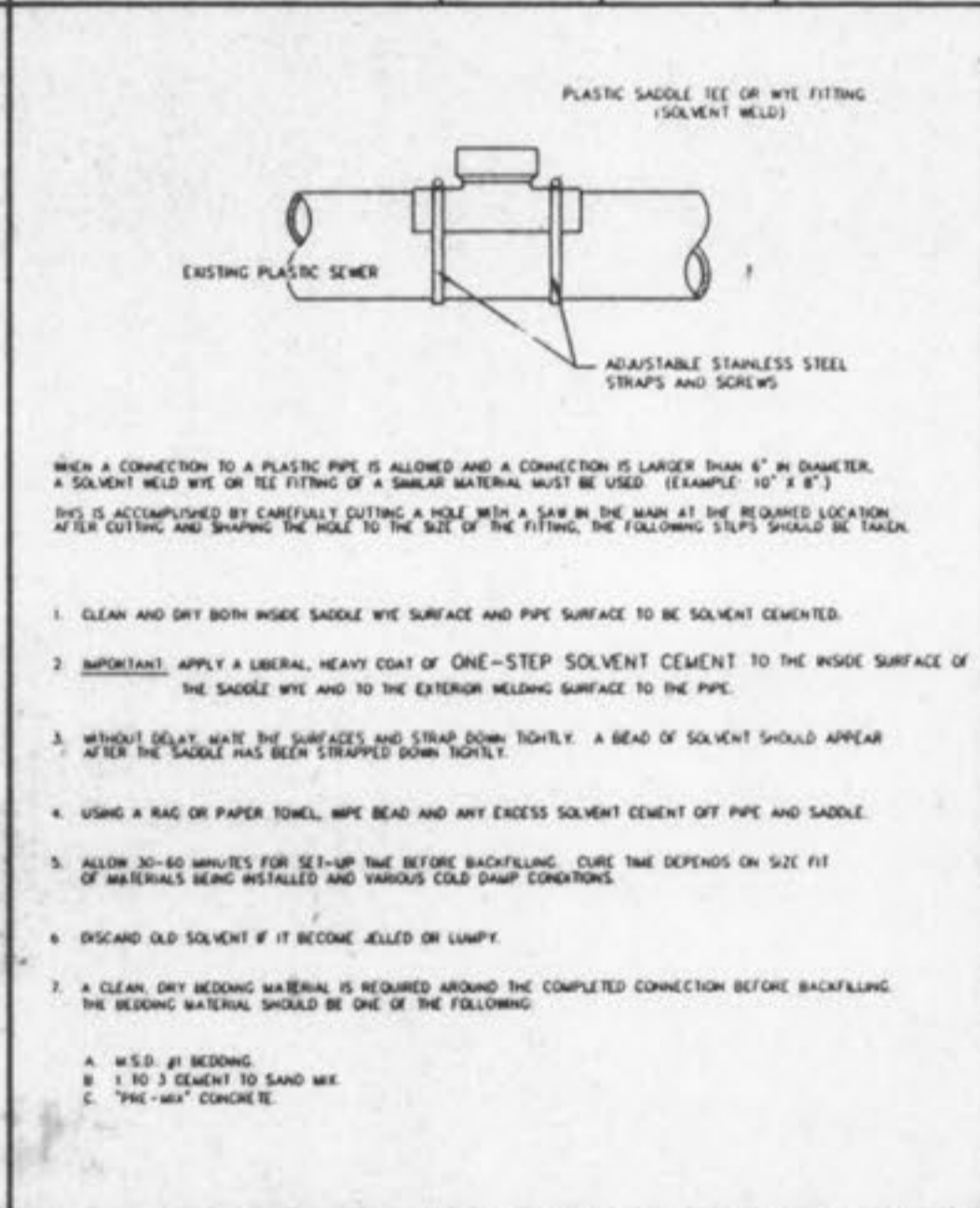
8" (& LARGER) CONNECTION TO PLASTIC MAIN METROPOLITAN ST. LOUIS SEWER DISTRICT Standard Details of Sewer Construction Dr. D.A.B. 1992 SHEET 62 Ch. J.C.K.
