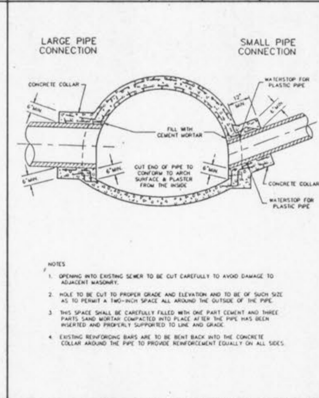
CONNECTIONS TO LARGE SEWERS METROPOLITAN ST. LOUIS SEWER DISTRICT Standard Details of Sewer Construction Dr. W.S.H. 1992 SHEET 64 Ch. J.C.K.
