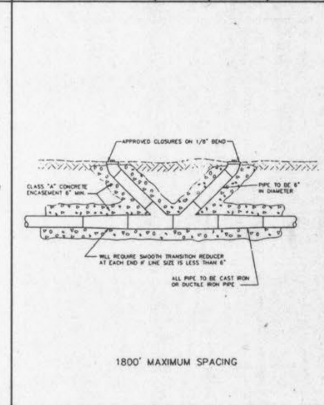
FORCE MAIN CLEANOUT (6" DIA. & SMALLER) METROPOLITAN ST. LOUIS SEWER DISTRICT Standard Details of Sewer Construction Dr. R.G.W. 1992 SHEET 65 Ch. J.C.K.
