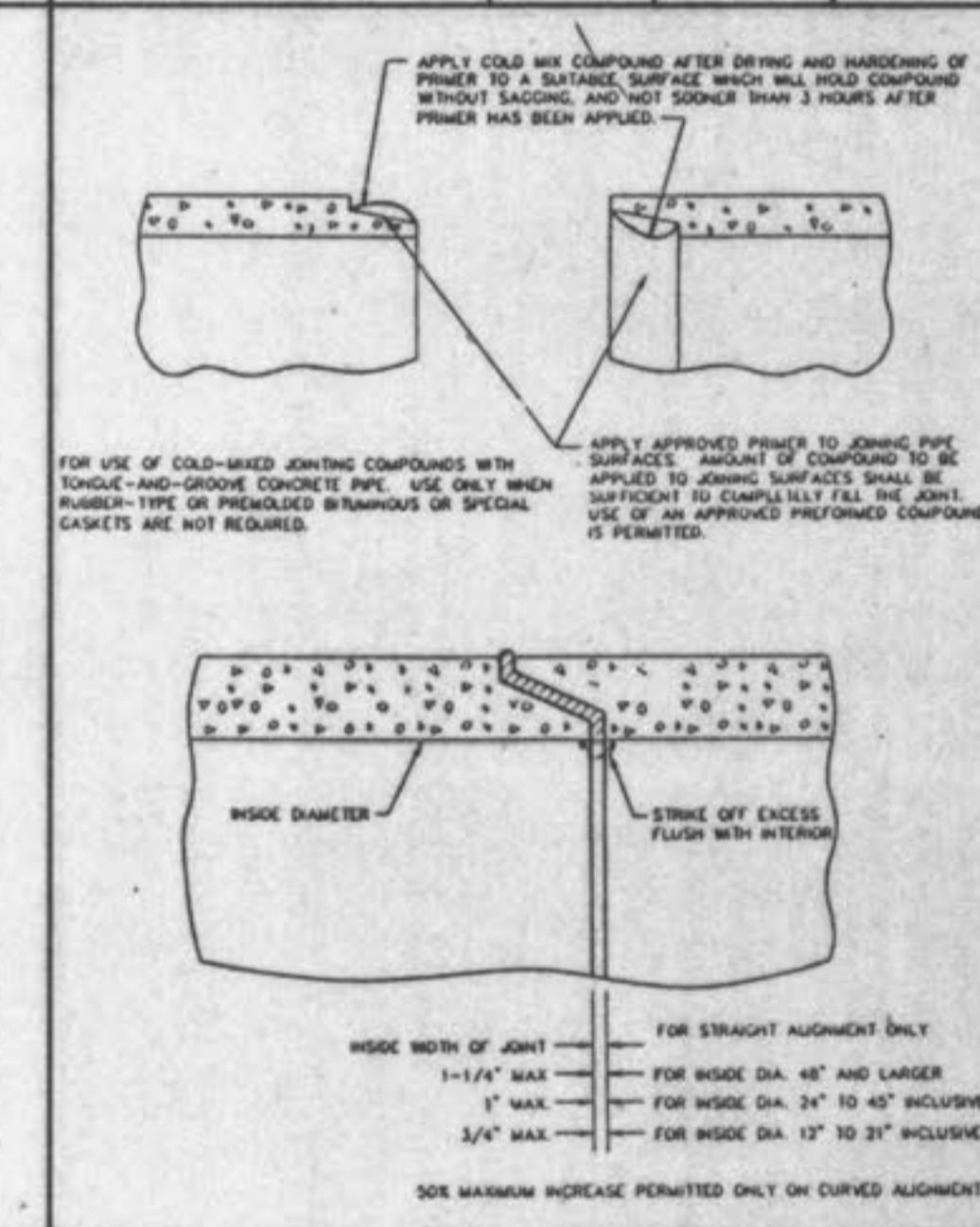
TONGUE AND GROOVE CONCRETE PIPE JOINTS METROPOLITAN ST. LOUIS SEWER DISTRICT Standard Details of Sewer Construction Dr. D.A.B. 1992 SHEET 66 Ch. J.C.K.
