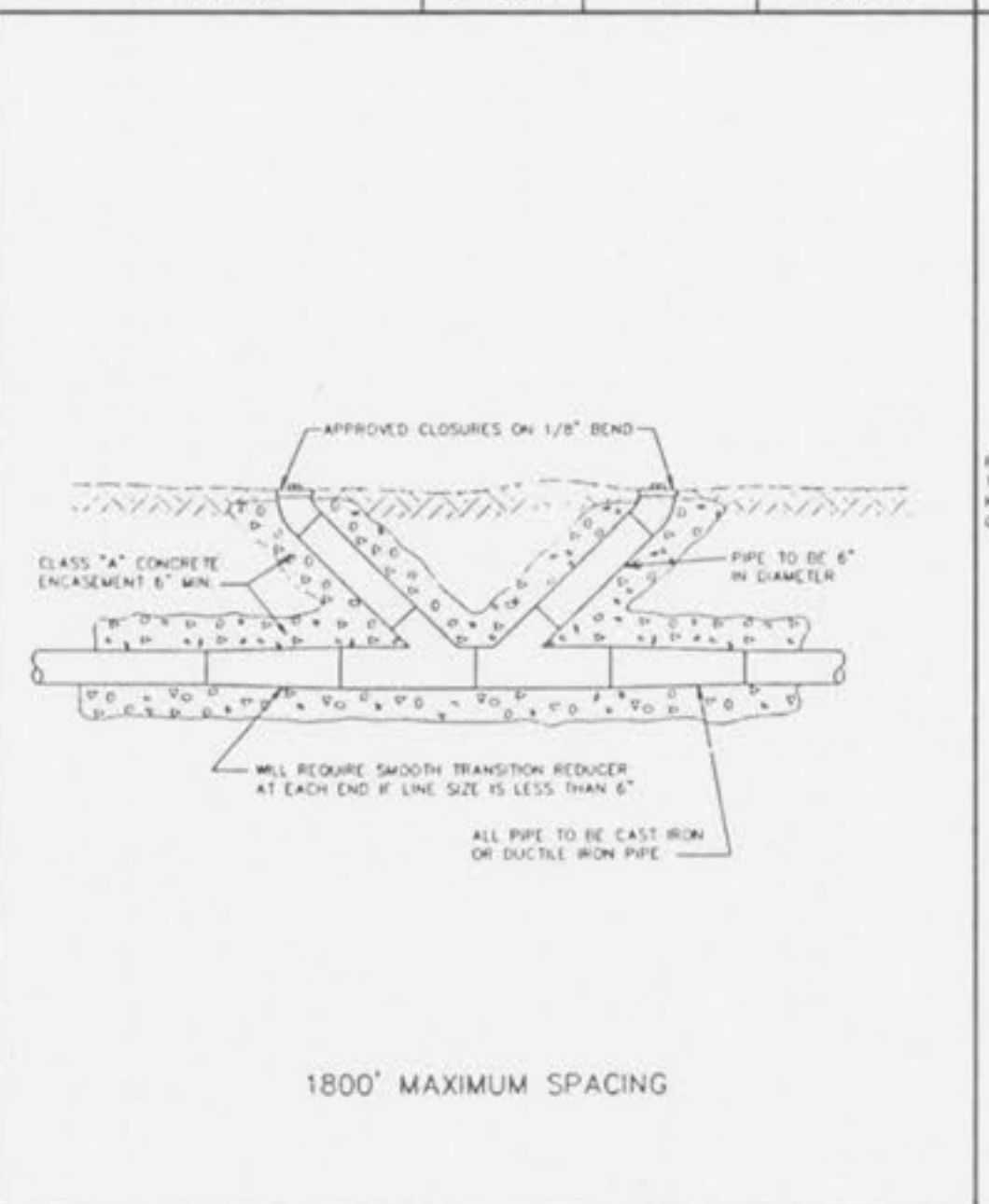
FORCE MAIN CLEANOUT (6\"/>
