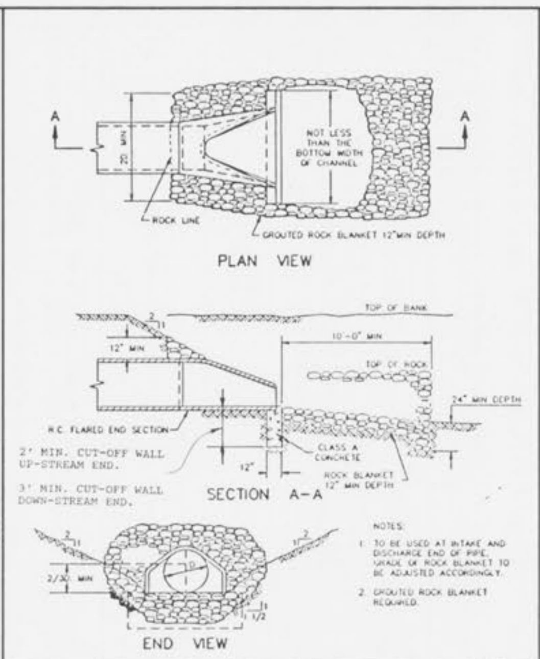
FLARED END SECTION METROPOLITAN ST. LOUIS SEWER DISTRICT Standard Details of Sewer Construction
