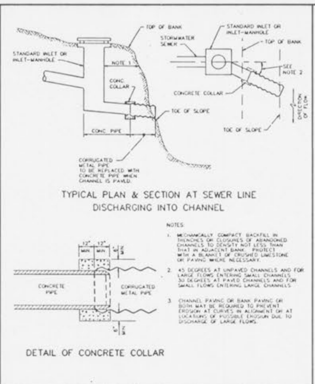
STORMWATER CHANNELS METROPOLITAN ST. LOUIS SEWER DISTRICT Standard Details of Sewer Construction
