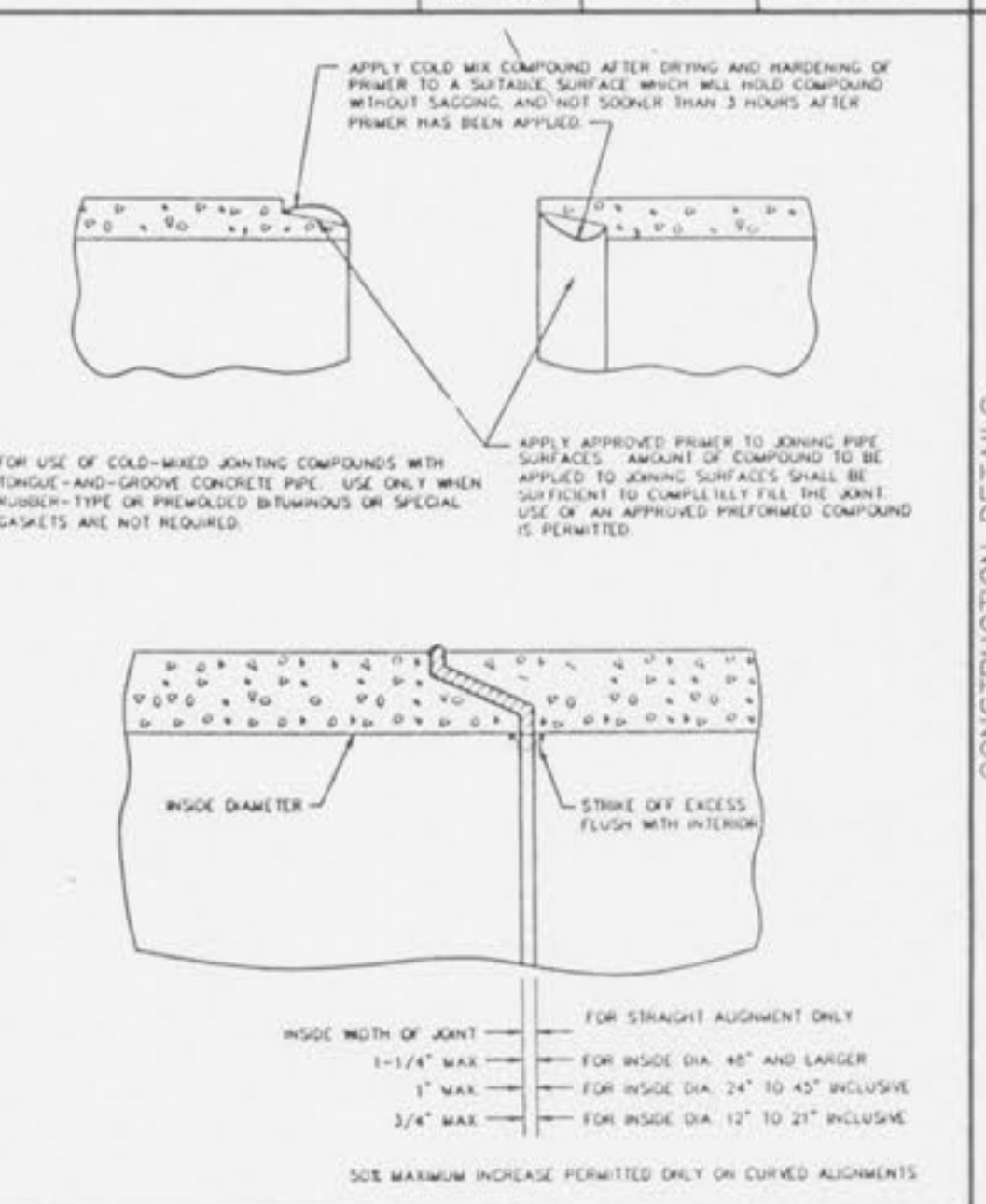
TONGUE AND GROOVE CONCRETE PIPE JOINTS METROPOLITAN ST. LOUIS SEWER DISTRICT Standard Details of Sewer Construction
