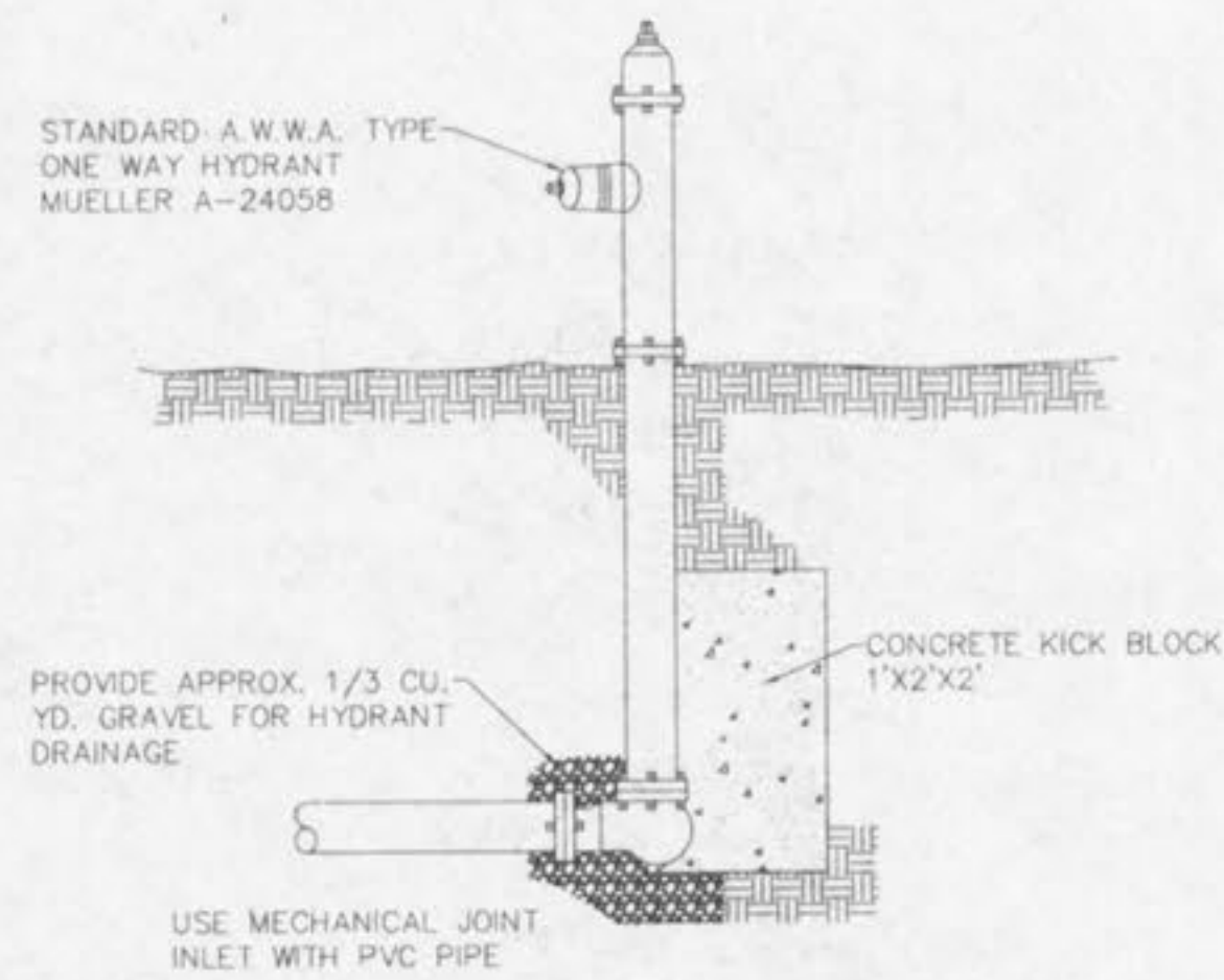
FLUSHING HYDRANT NOT TO SCALE
