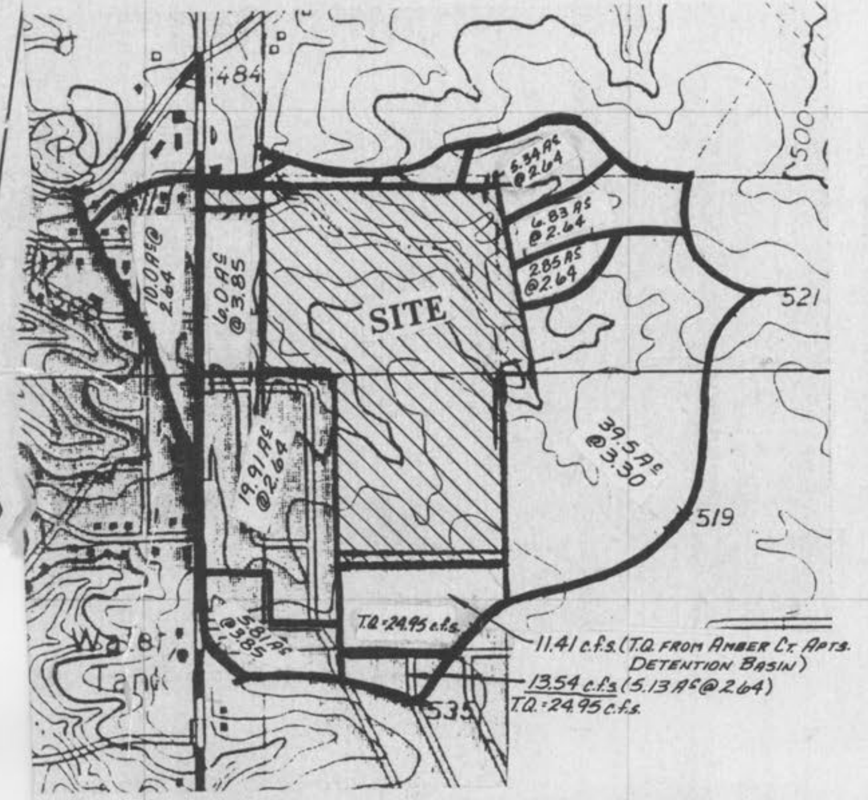
OFFSITE DRAINAGE AREA MAP SCALE = 1" = 500'
