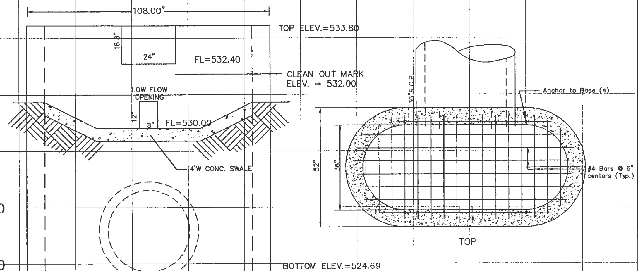
OVERFLOW STRUCTURE (PRECAST CONCRETE) OS 30 DETAIL
