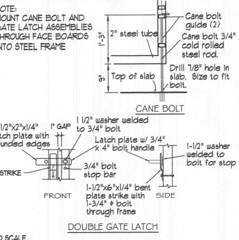
12 GATE LATCH / BOLT DETAILS
