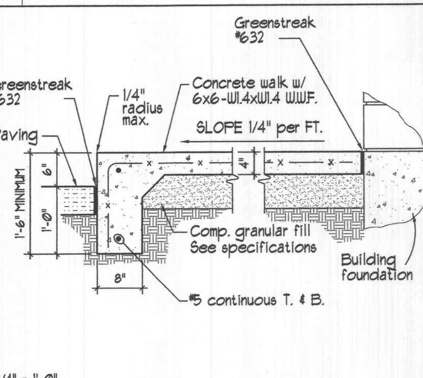
17 TYPICAL WALK SECTION
