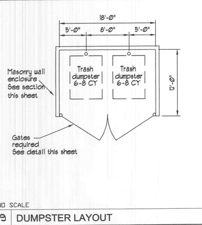
9 DUMPSTER LAYOUT
