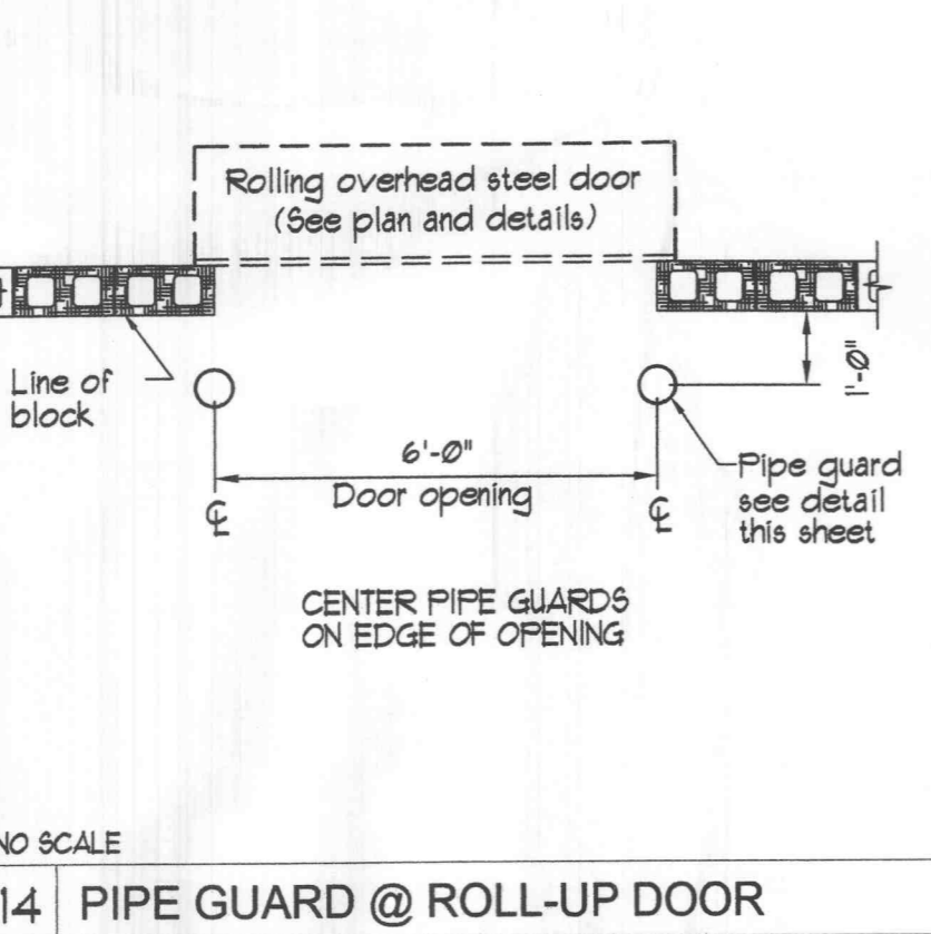
14 PIPE GUARD @ ROLL-UP DOOR
