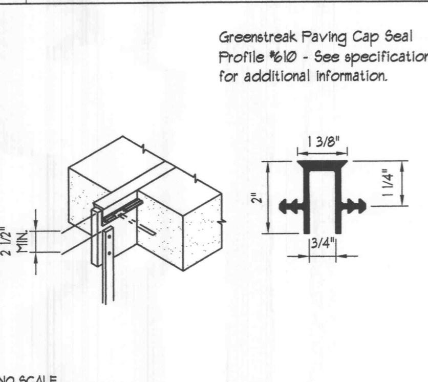
18 TYPICAL EXPANSION JOINT
