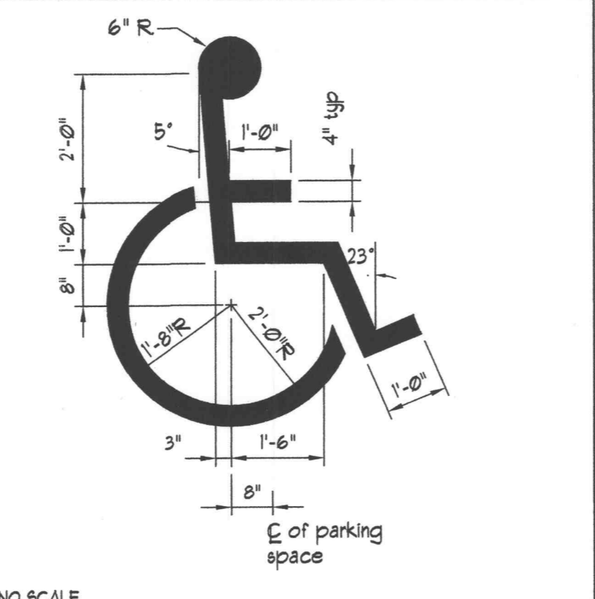
7 INT'L BARRIER FREE SYMBOL
