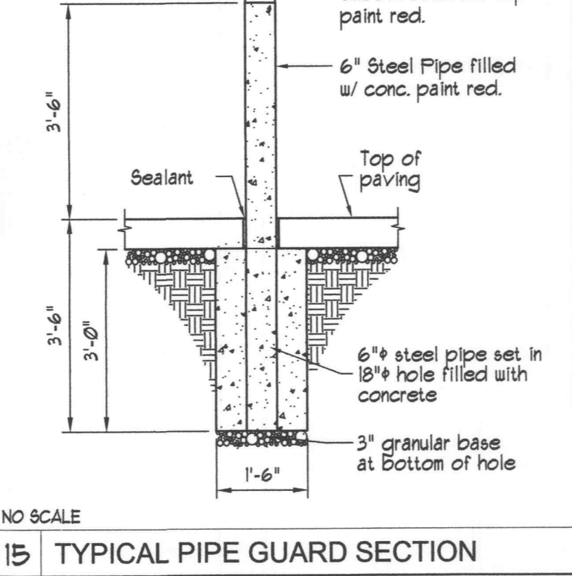
15 TYPICAL PIPE GUARD SECTION
