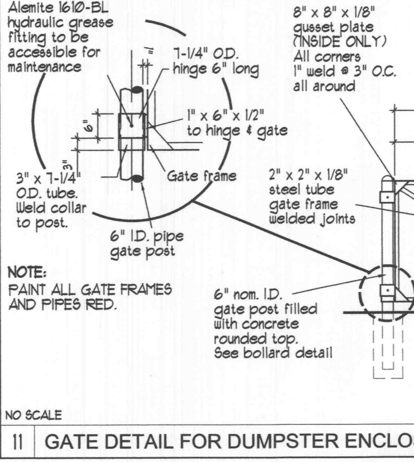
11 GATE DETAIL FOR DUMPSTER ENCLOSURE
