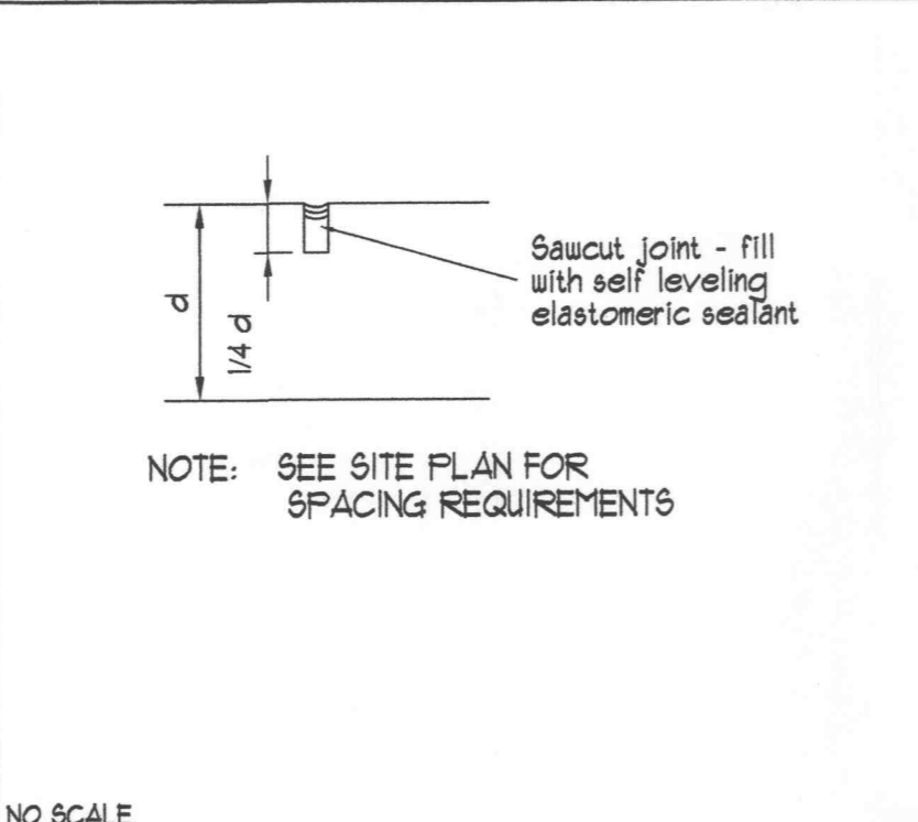
19 TYPICAL CONTROL JOINT
