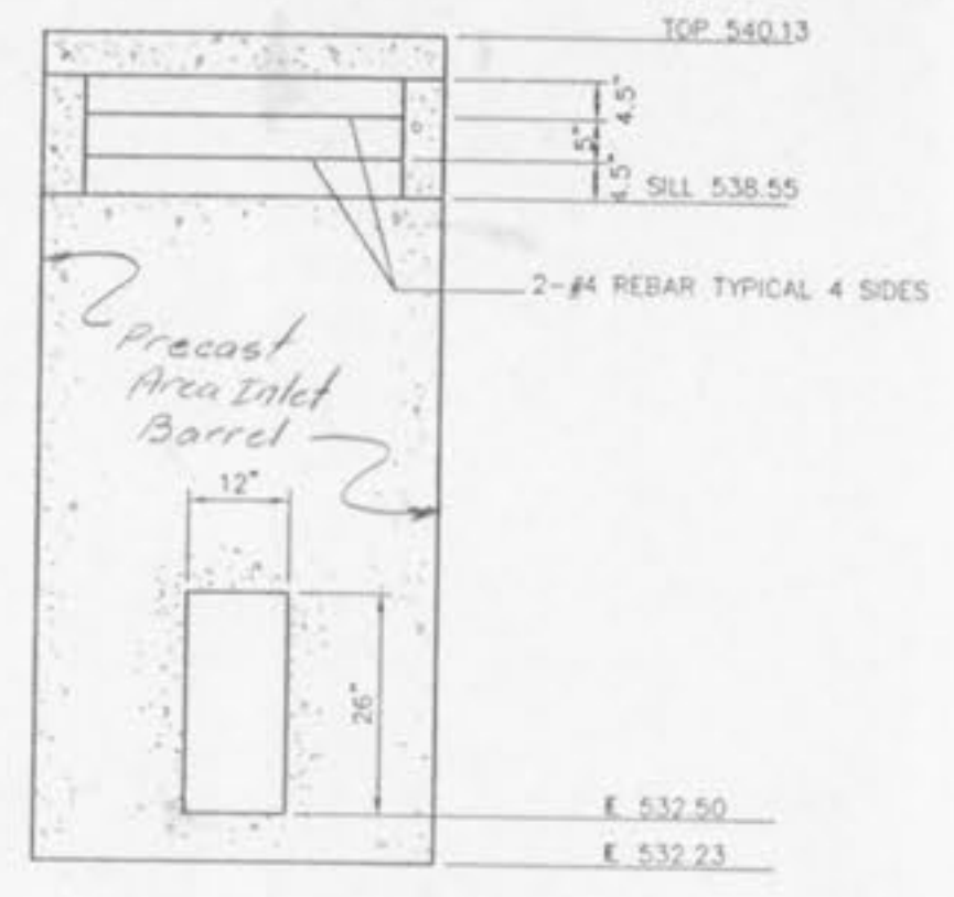
OUTFLOW STRUCTURE 222
