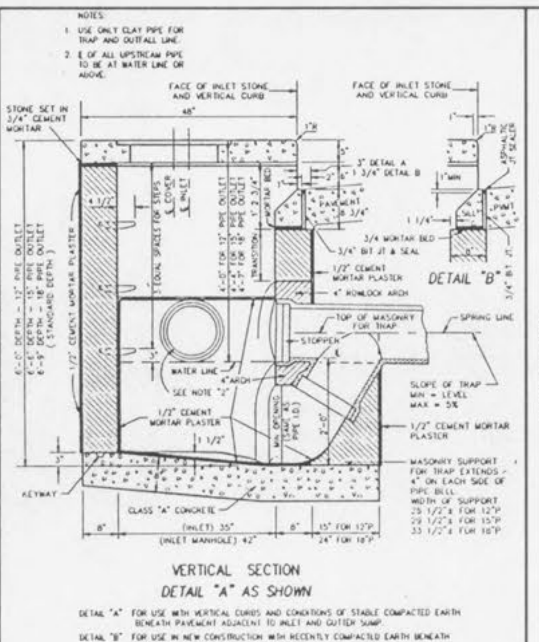
TRAPPED STREET INLET BRICK CONSTRUCTION METROPOLITAN ST. LOUIS SEWER DISTRICT Standard Details of Sewer Construction
