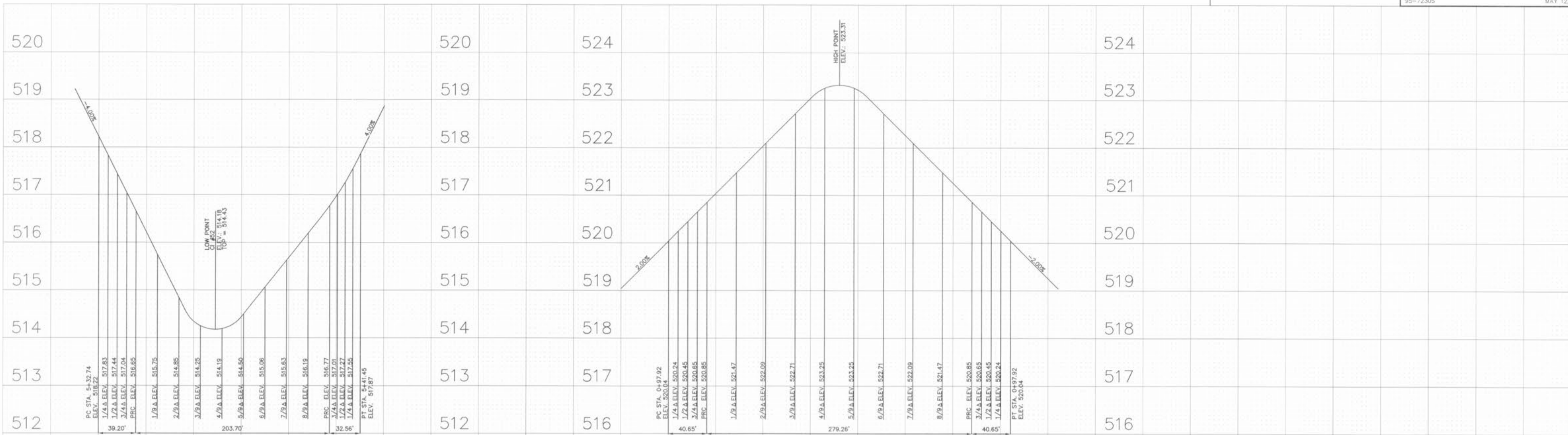
HARRISBURG COURT CUL-DE-SAC WARPING TOP OF CURB ELEVATION
