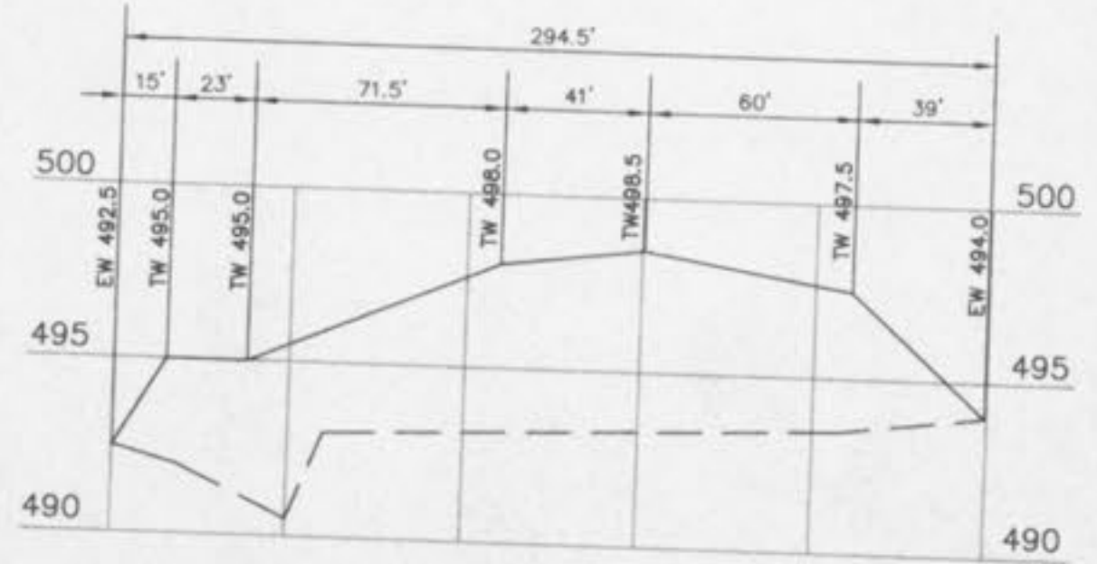
WALL PROFILE SCALE: 1"=50'H, 1"=5'V
