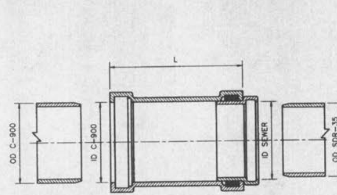
SDR-35 x C900 BELL & BELL ADAPTERS
