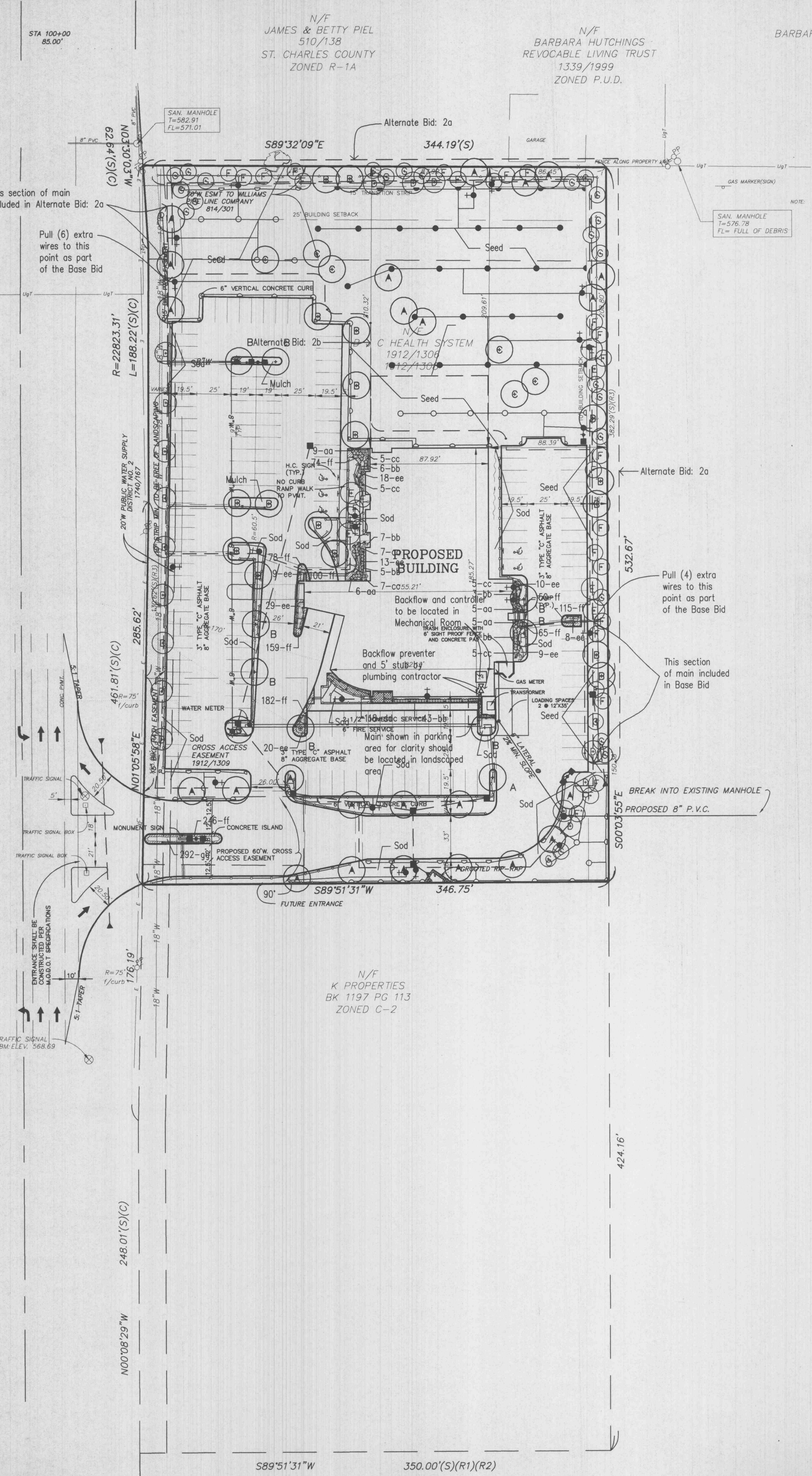
Irrigation Plan Scale: 1" = 40'-0"
