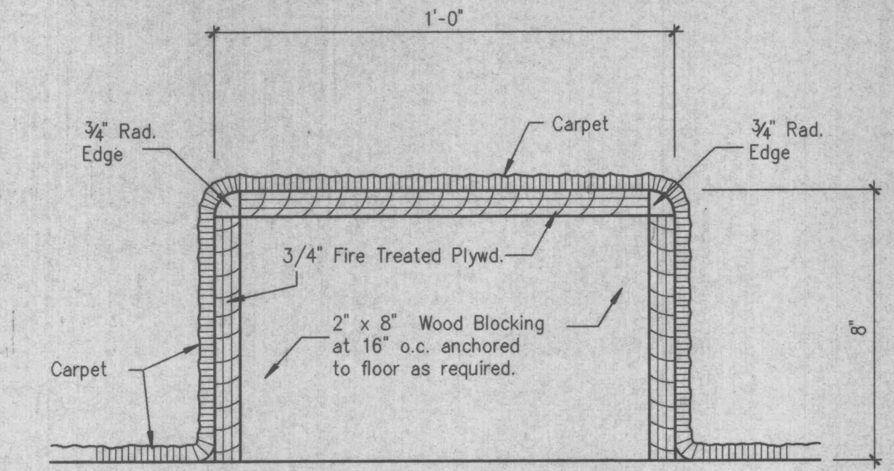
5 SECTION AT PLAY CURB
