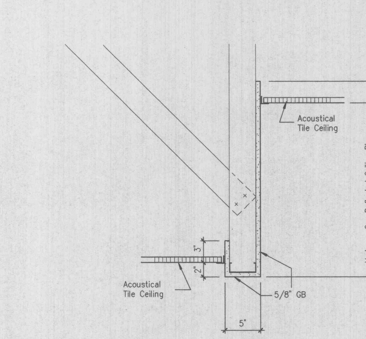
8 GYP. BD. SOFFIT DETAIL
