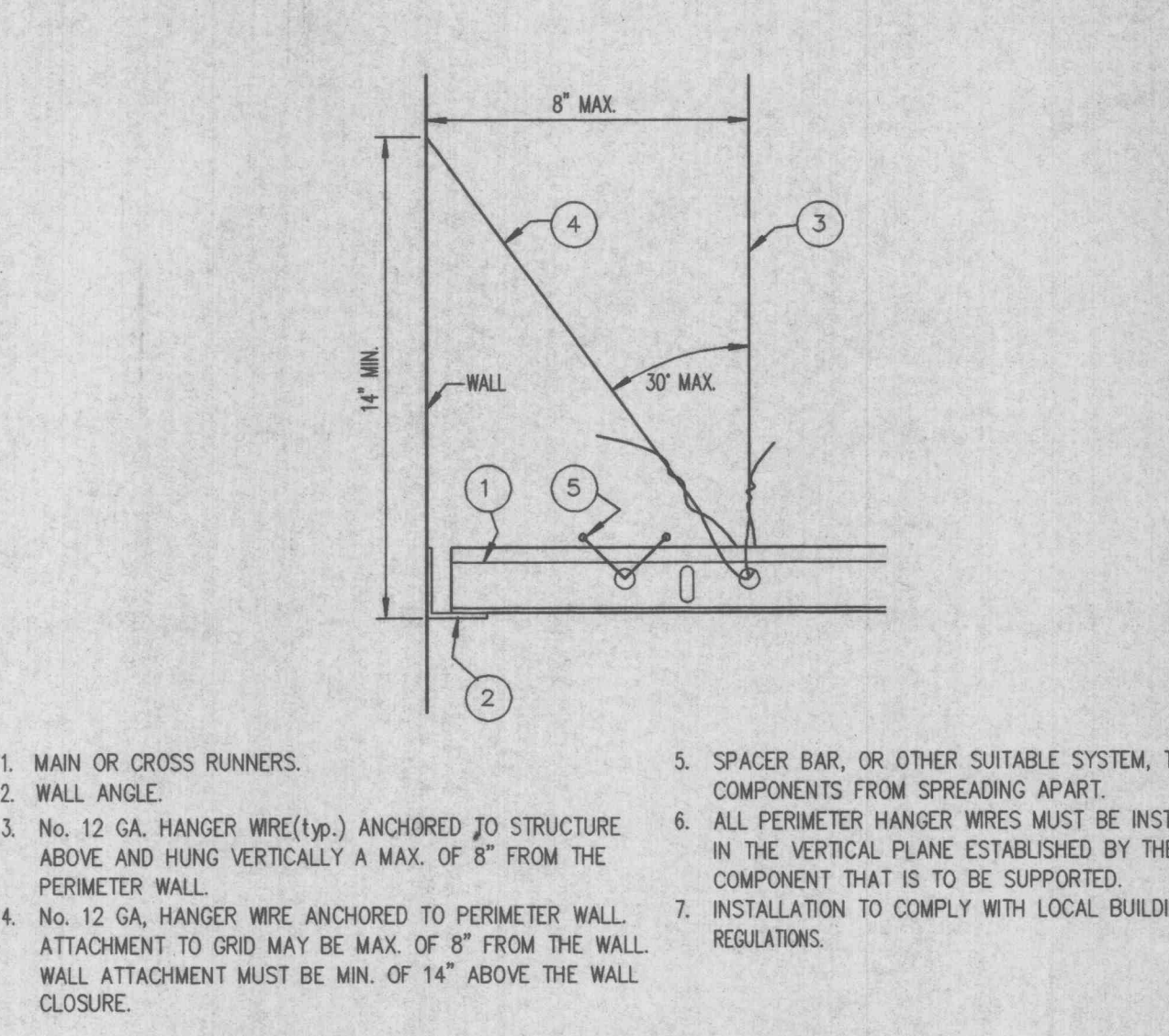
SUSPENDED ACOUST. CEILINGS PERIMETER SEISMIC BRACING DET.
