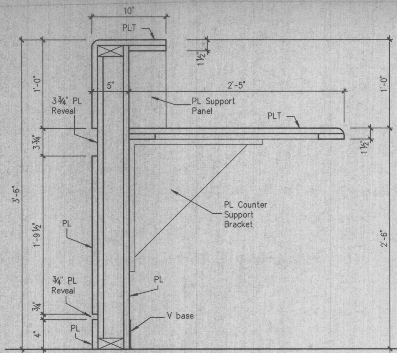
1 CASEWORK SECTION
