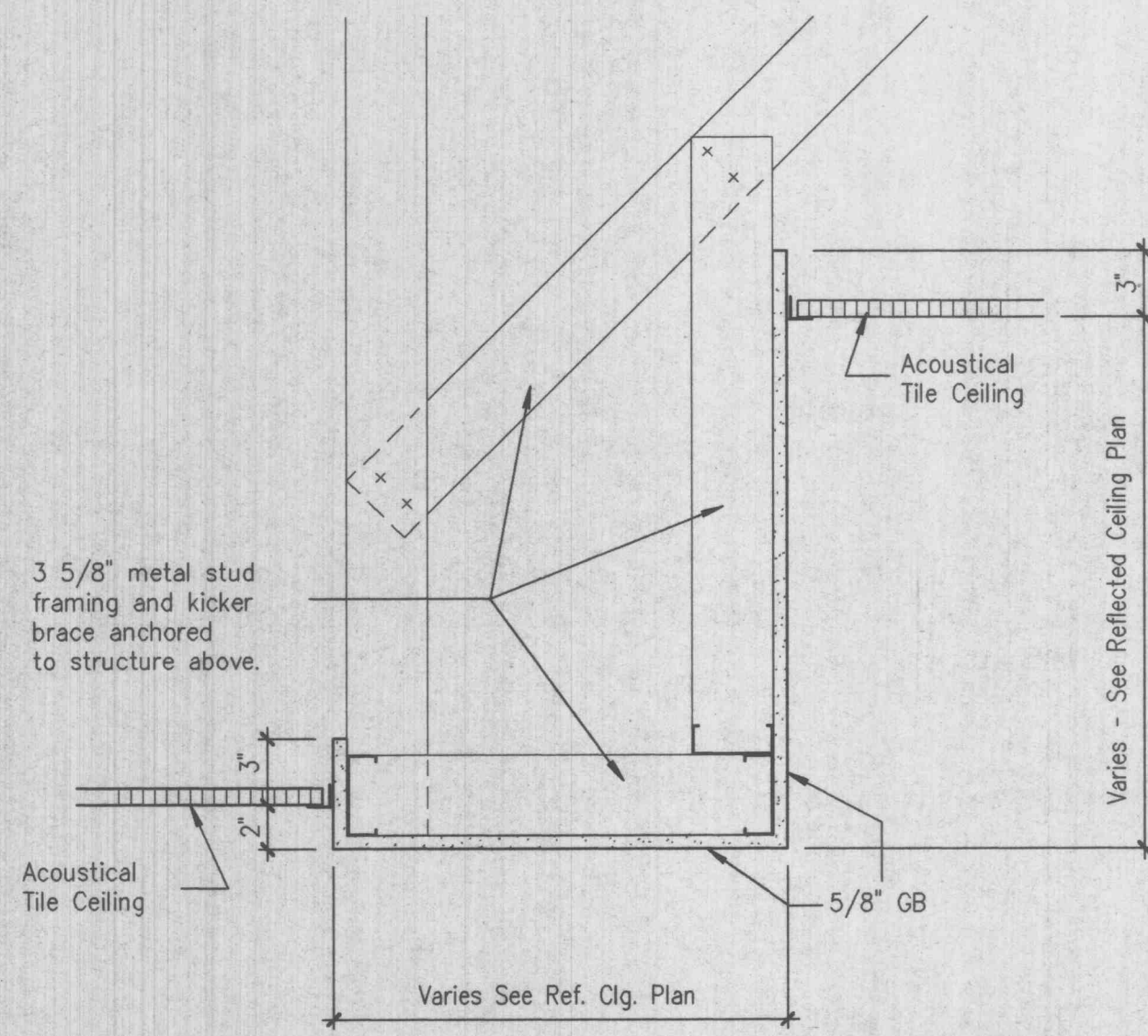
7 GYP. BD. SOFFIT DETAIL
