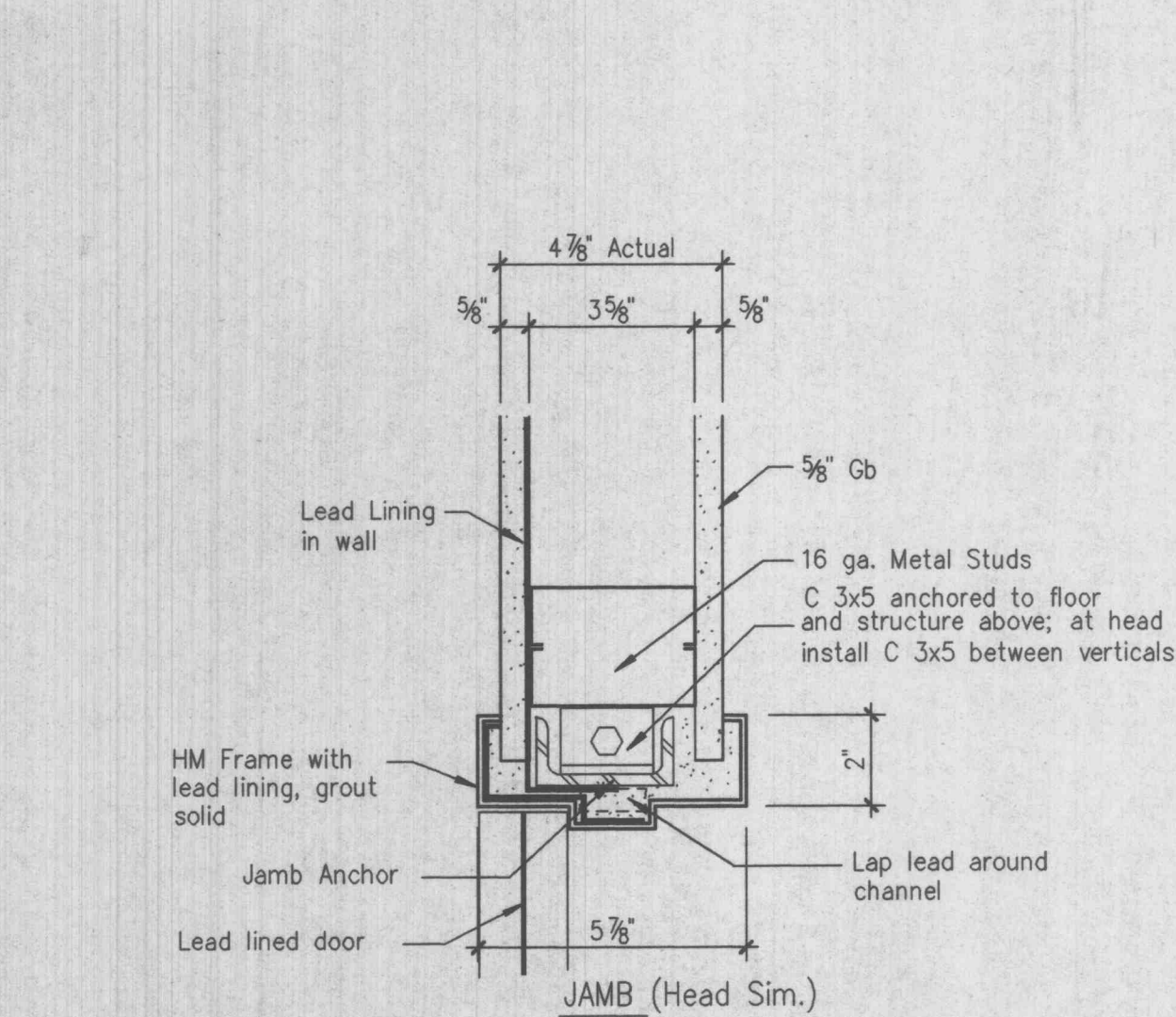
12 LEAD LINED DOOR FRAME
