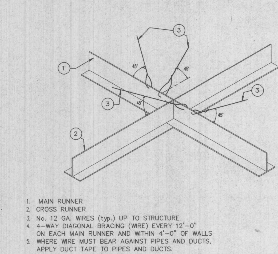
SUSPENDED ACOUSTICAL CEILINGS SEISMIC BRACING DETAIL
