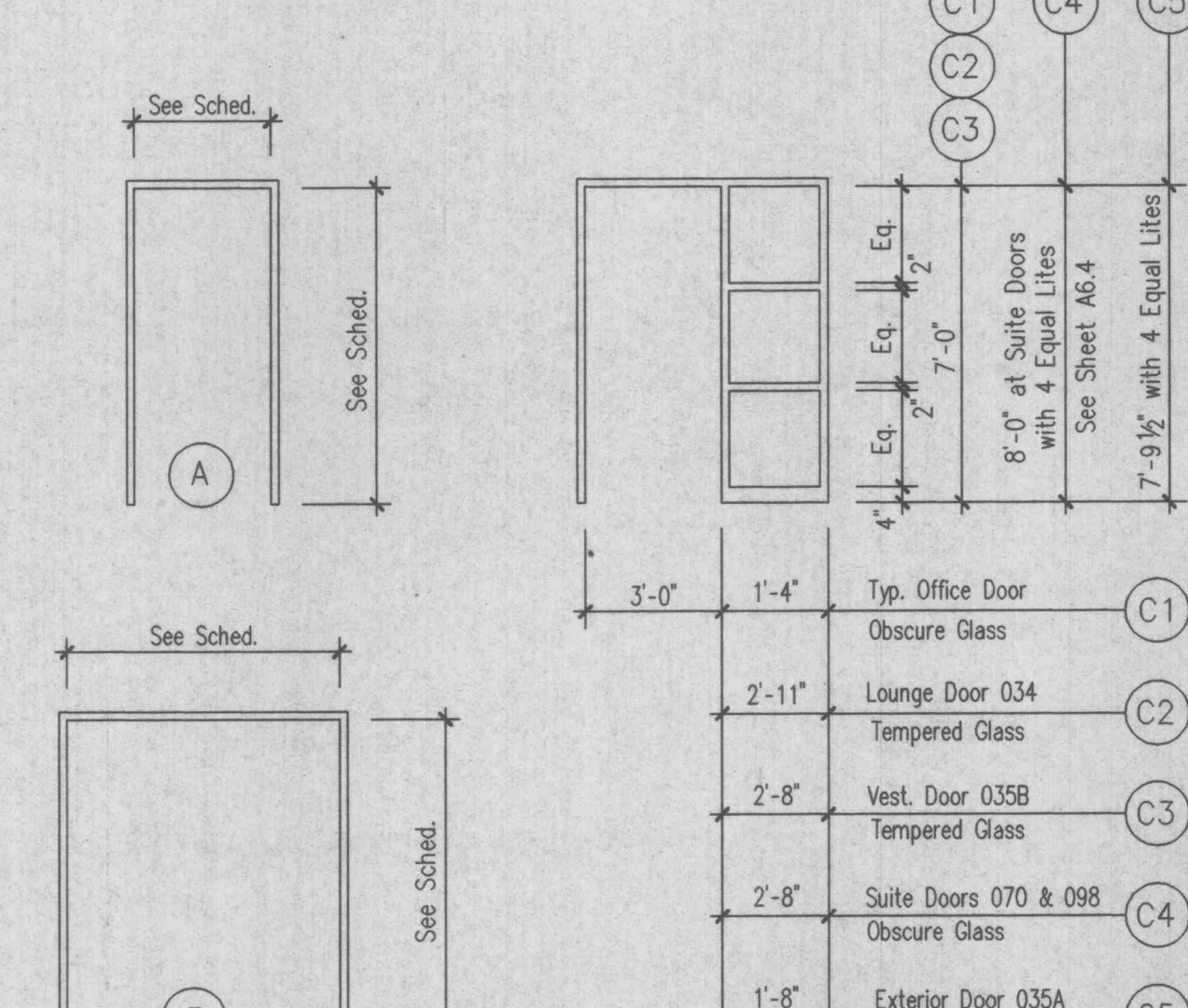
15 FRAME TYPES
