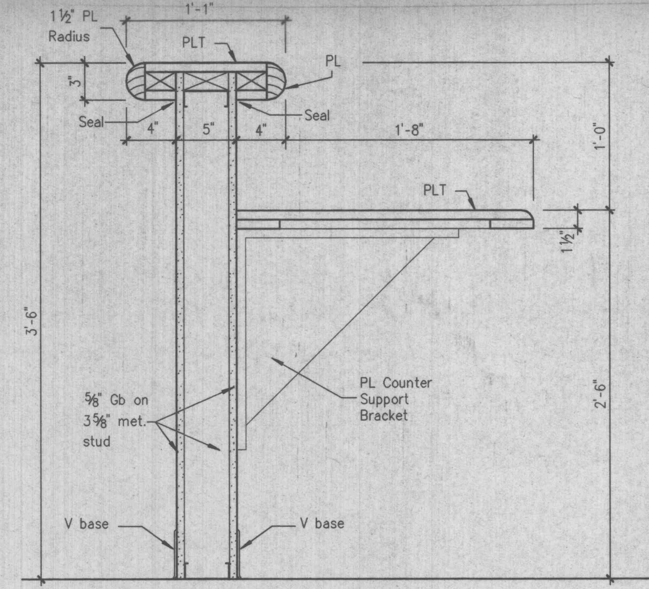
4 CASEWORK SECTION
