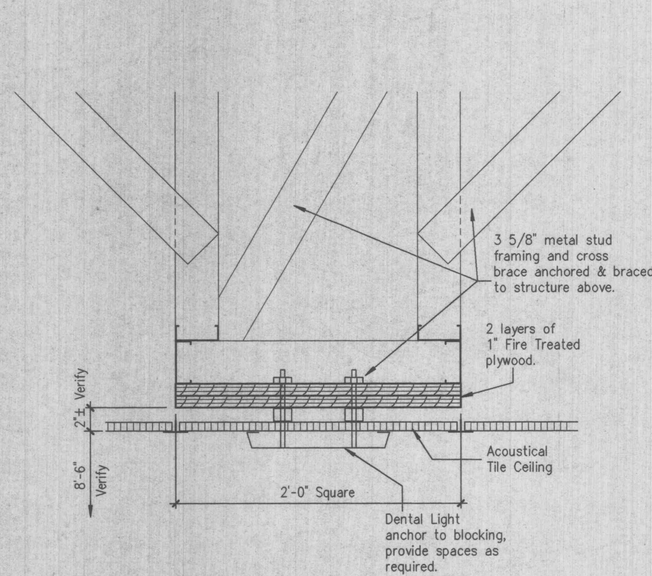
6 SUSPENSION DETAIL
