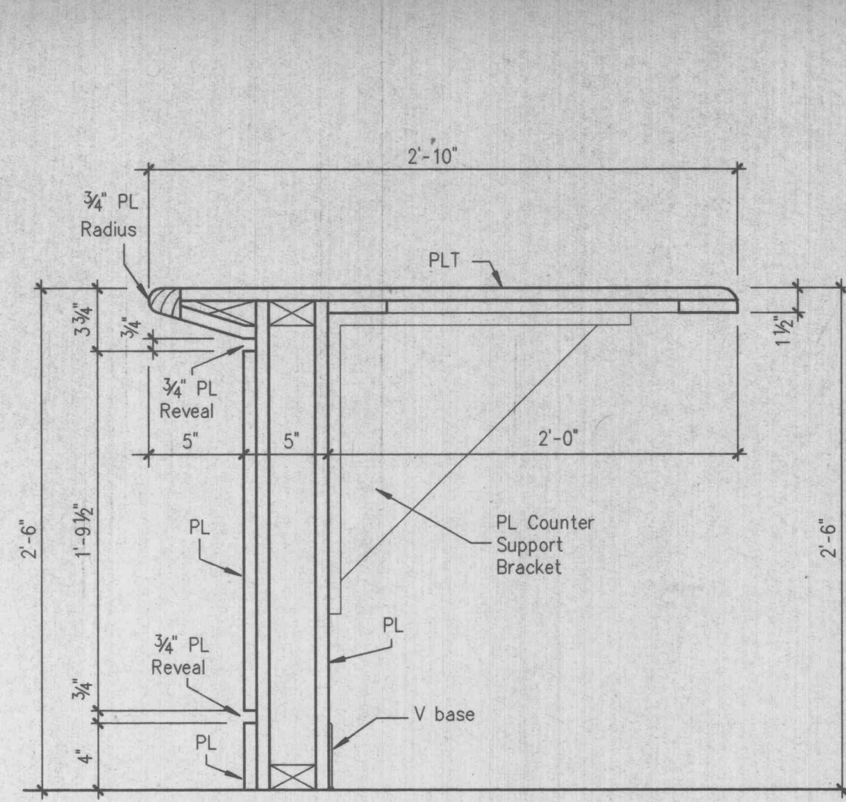
3 CASEWORK SECTION
