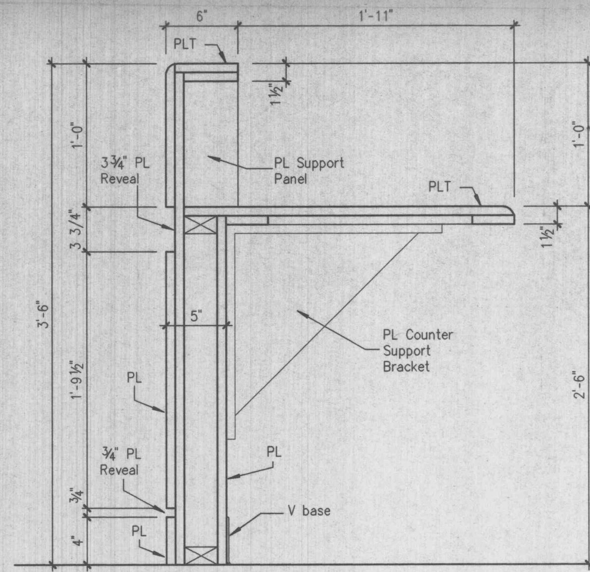
2 CASEWORK SECTION
