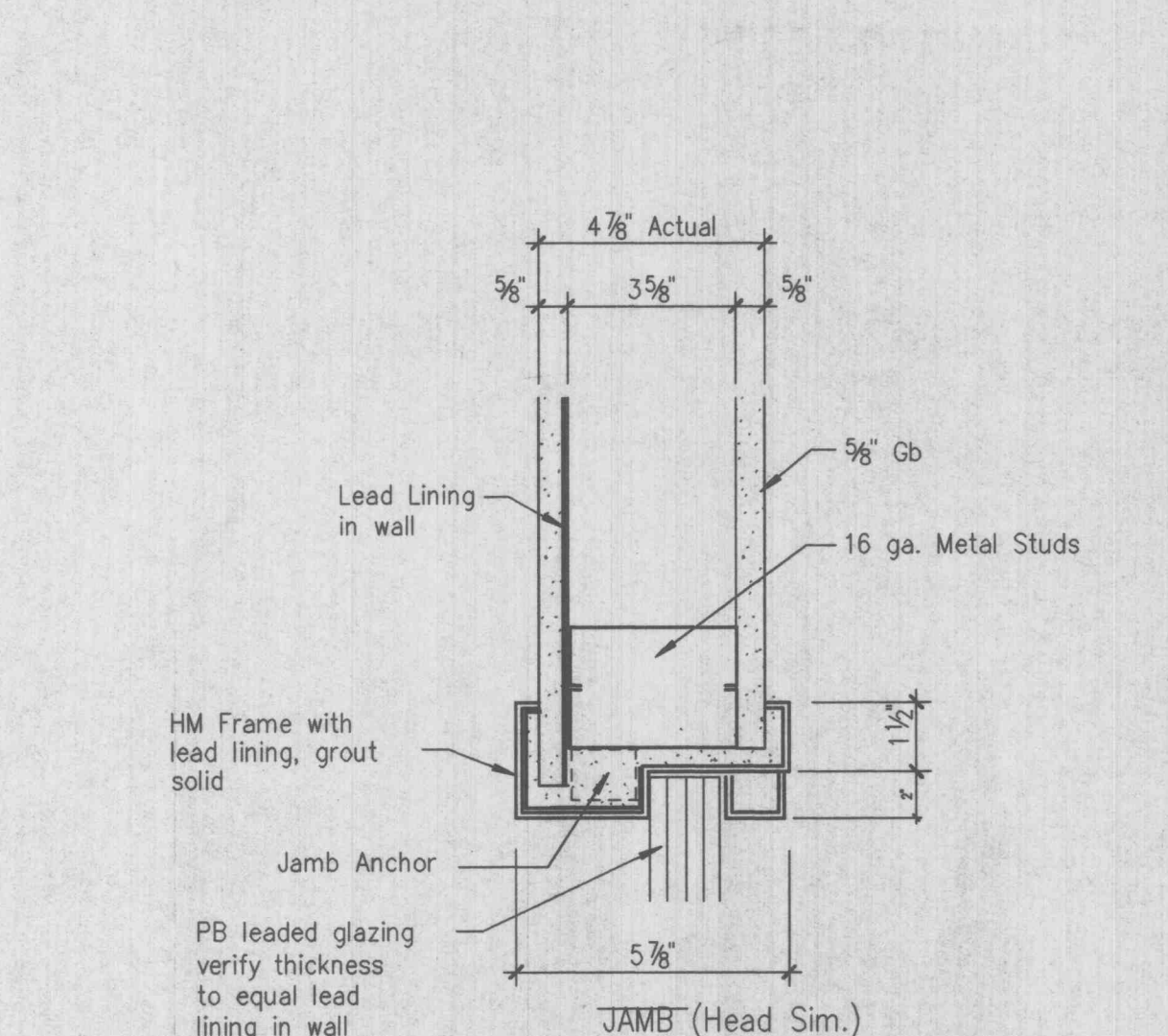
13 LEAD LINED BORROW LITE
