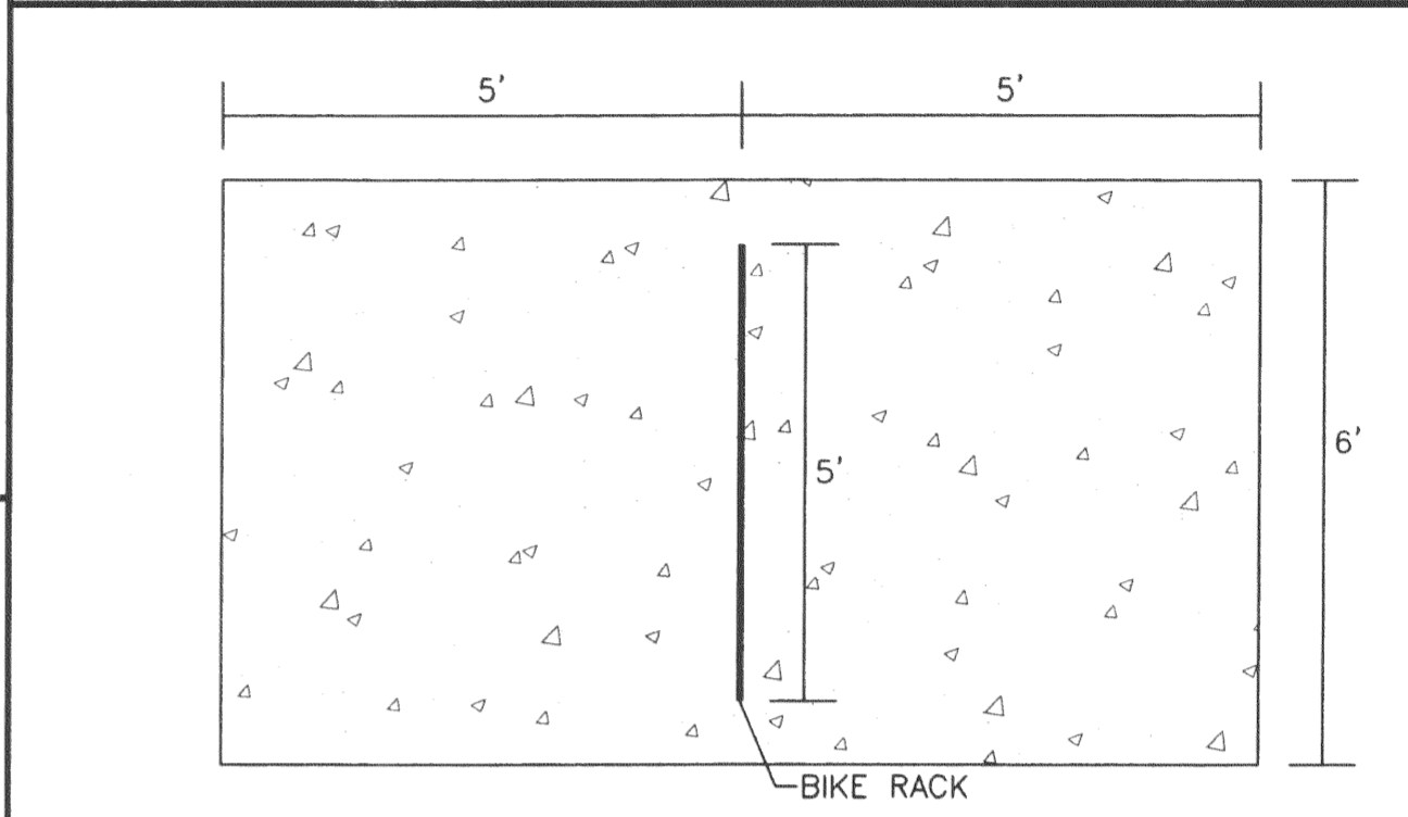
BICYCLE RACK DETAIL
