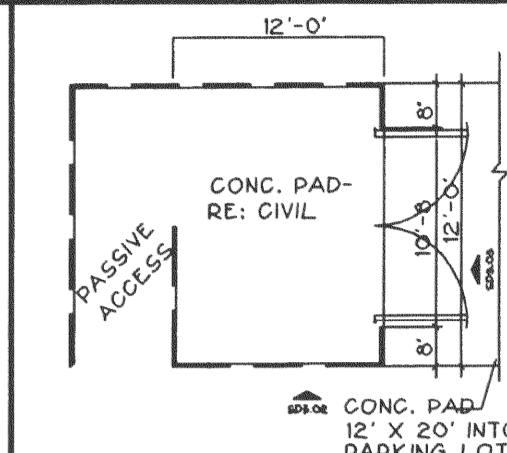
SD3.01 TRASH ENCLOSURE PLAN
