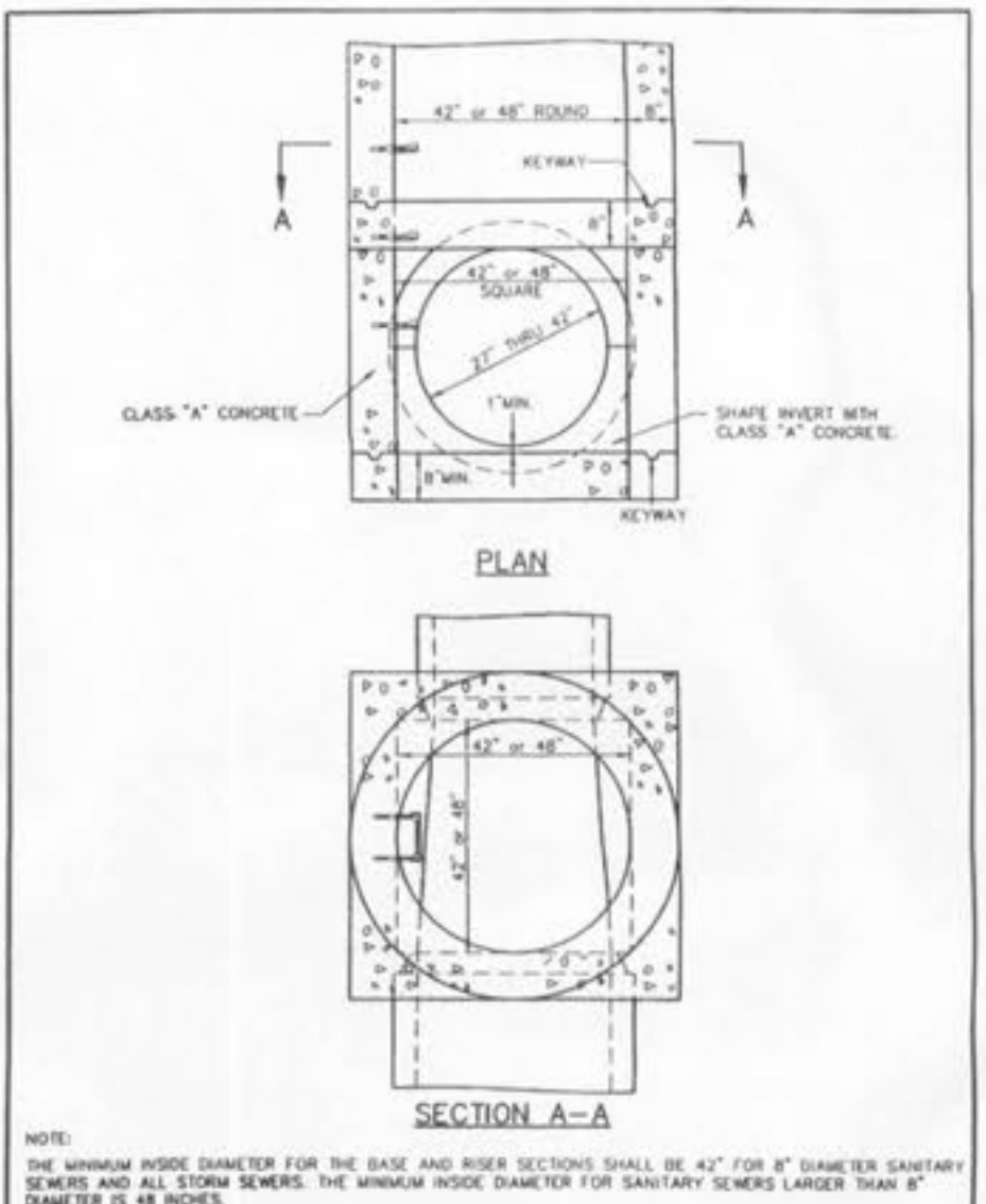
MANHOLE ON PIPE SEWER 27" THRU 42" (ALTERNATE) METROPOLITAN ST. LOUIS SEWER DISTRICT Standard Details of Sewer Construction Dr. D.A.B./S.A.M. Ch. J.C.K. 2000 SHEET 12
