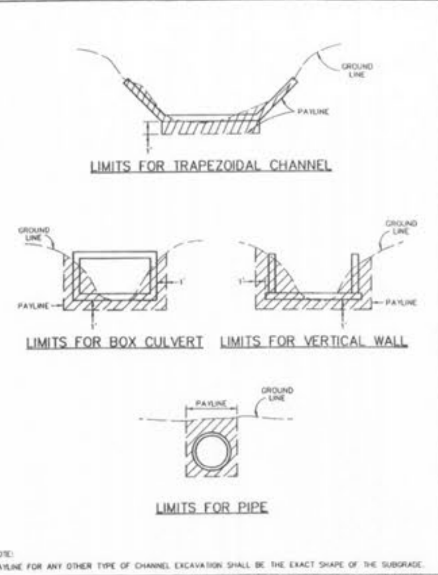
PAYLINE LIMITS FOR EXCAVATION METROPOLITAN ST. LOUIS SEWER DISTRICT Standard Details of Sewer Construction Dr. W.S.H. Ch. J.C.K. 2000 SHEET 2
