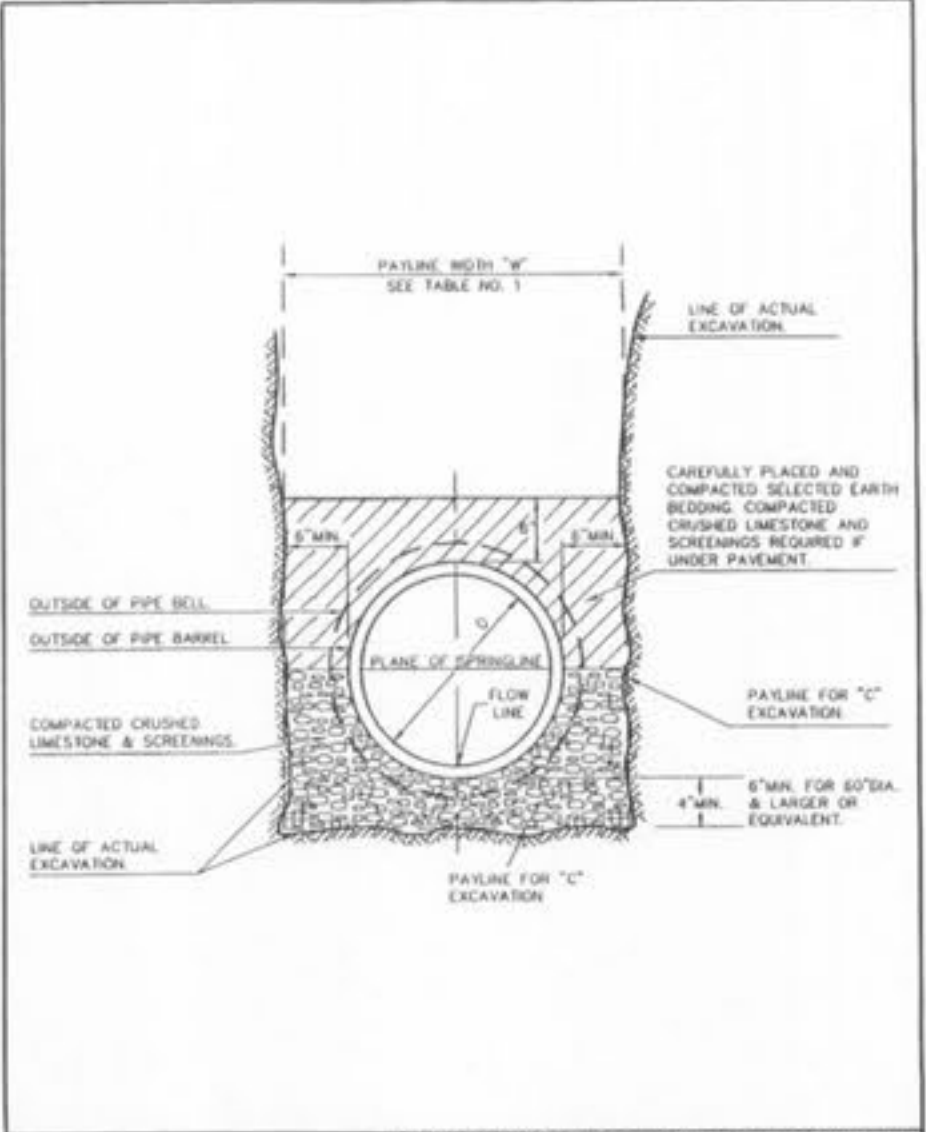
PIPE BEDDING CLASS "C" (MODIFIED FOR REINFORCED CONCRETE PIPE) METROPOLITAN ST. LOUIS SEWER DISTRICT Standard Details of Sewer Construction Dr. W.S.H. Ch. J.C.K. 2000 SHEET 5
