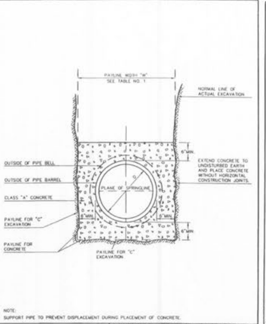
CONCRETE ENCASEMENT METROPOLITAN ST. LOUIS SEWER DISTRICT Standard Details of Sewer Construction Dr. W.S.H. Ch. J.C.K. 2000 SHEET 8
