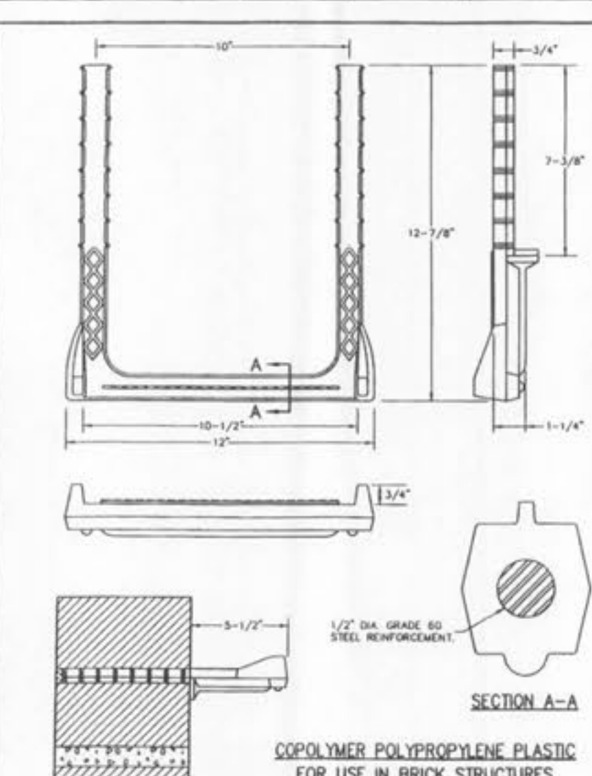
PS1-B MANHOLE STEP INTO JOINT METROPOLITAN ST. LOUIS SEWER DISTRICT Standard Details of Sewer Construction Dr. W.S.H. Ch. J.C.K. 2000 SHEET 57
