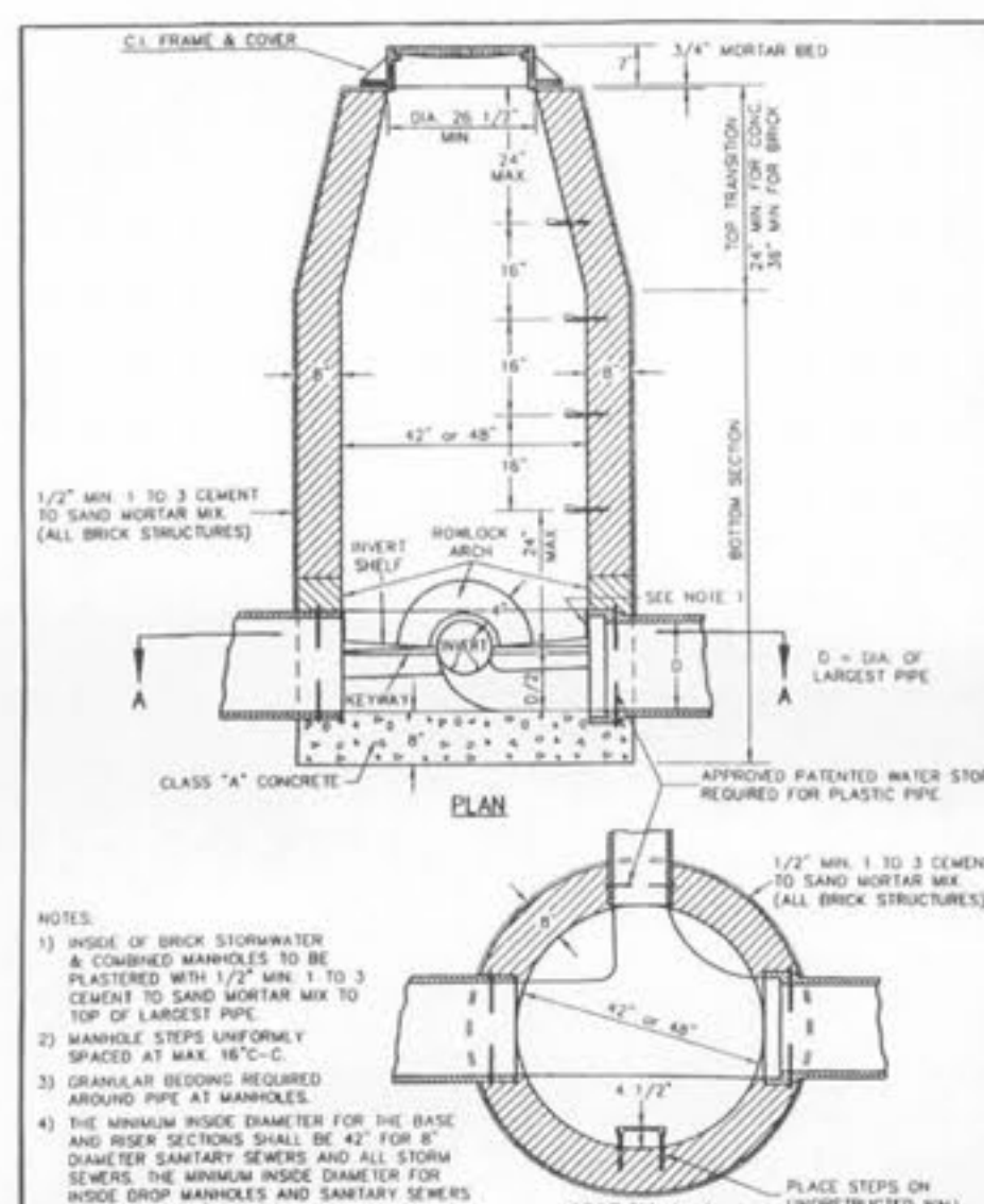
LINE MANHOLE ON PIPE SEWER 8"-24" DIA. METROPOLITAN ST. LOUIS SEWER DISTRICT Standard Details of Sewer Construction Dr. W.S.H./S.A.M. Ch. J.C.K. 2000 SHEET 10
