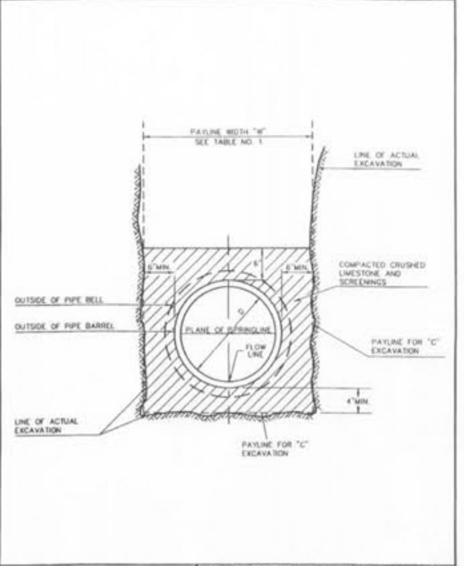
PIPE BEDDING CLASS "C" (MODIFIED FOR REINFORCED CONCRETE PIPE) METROPOLITAN ST. LOUIS SEWER DISTRICT Standard Details of Sewer Construction Dr. W.S.H. Ch. J.C.K. 2000 SHEET 4
