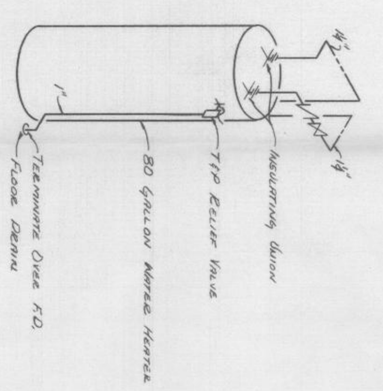
DOMESTIC WATER HEATER DETAIL NO SCALE
