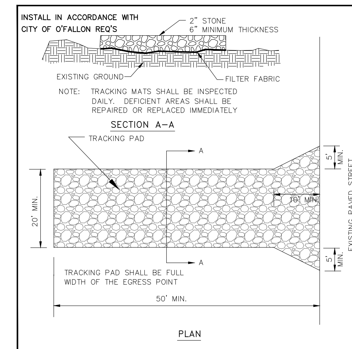
AGGREGATE WASH OFF ENTRANCE DETAIL NO SCALE
