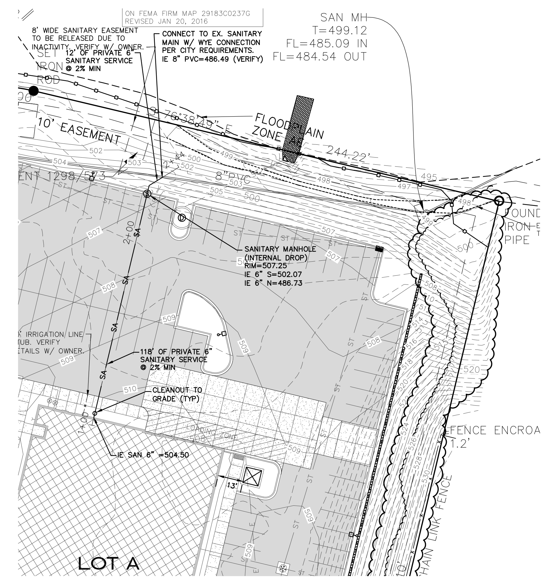
NORTH SANITARY PLAN SCALE: 1"=30'
