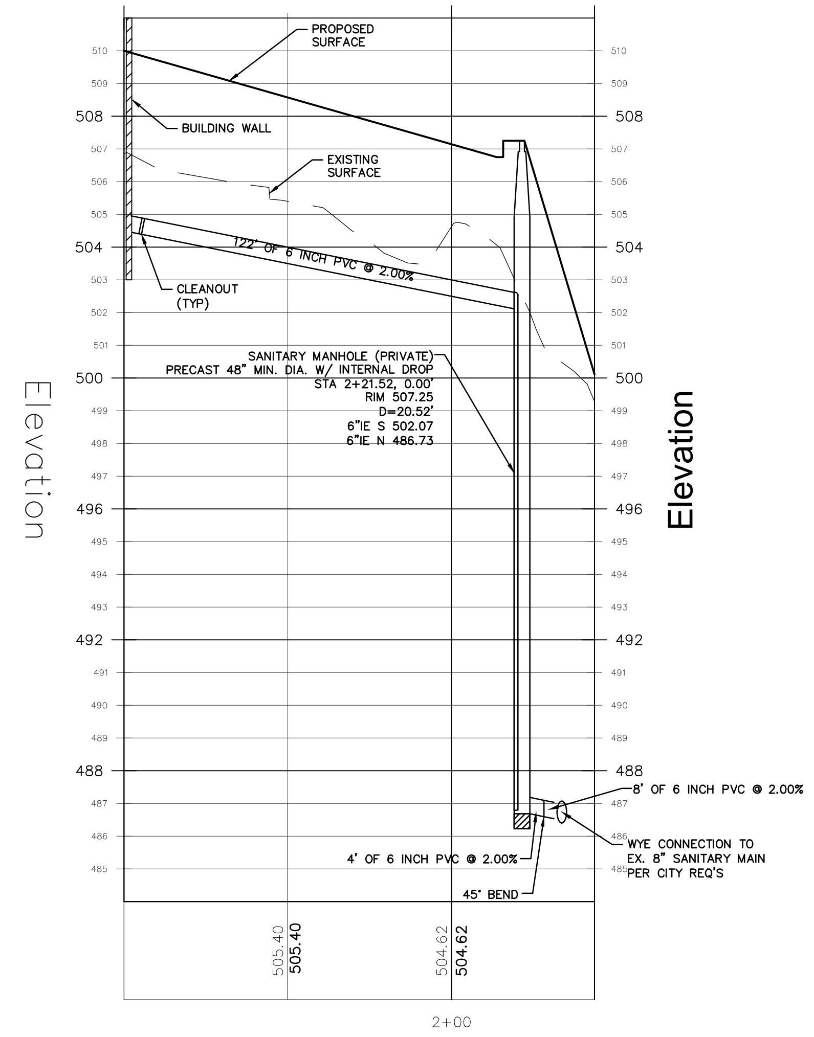
SANITARY PROFILE SCALE: HORIZONTAL: 1"=30' VERTICAL: 1"=3'
