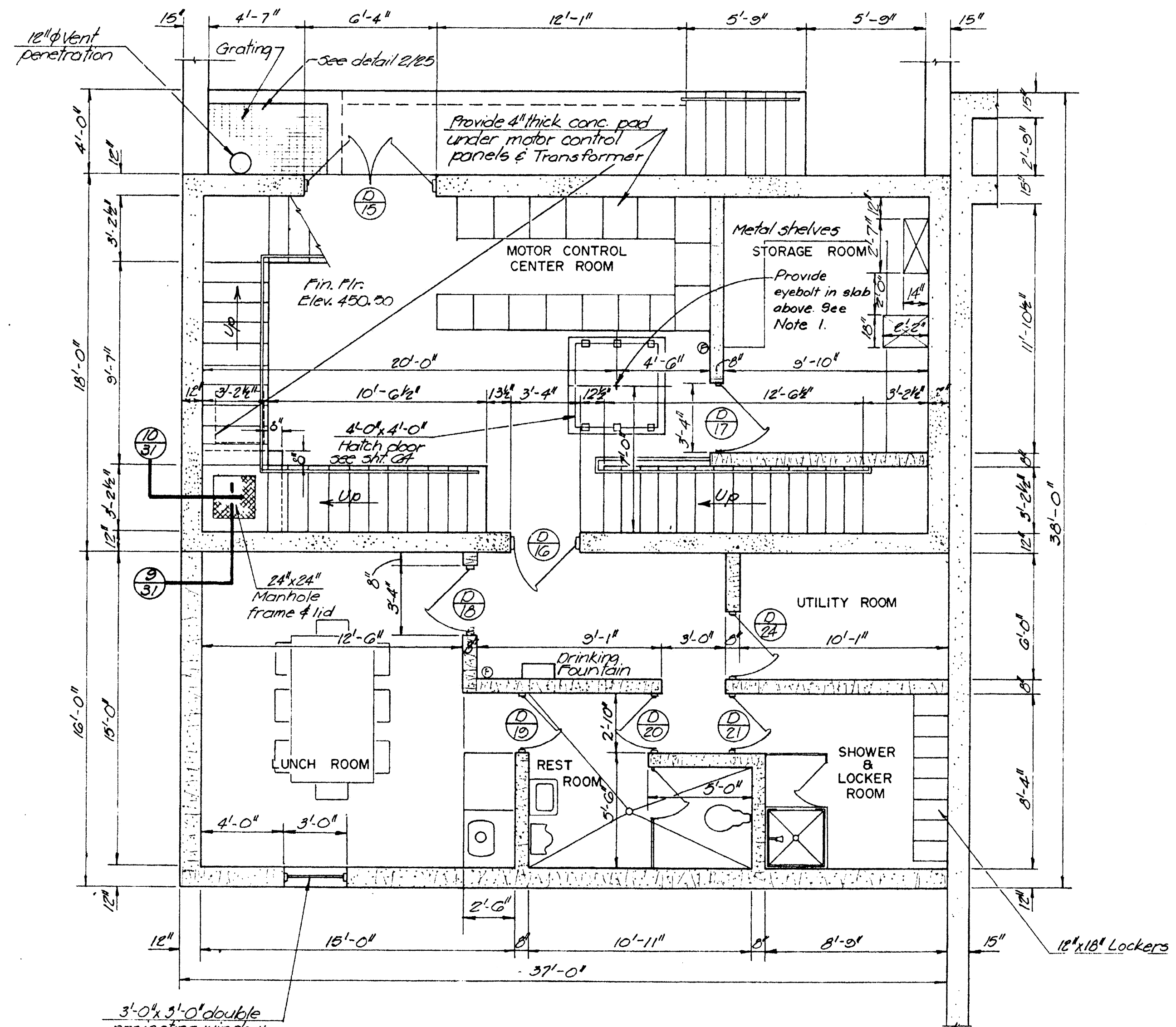
OPERATING FLOOR PLAN Scale: 1/4" = 1'-0"
