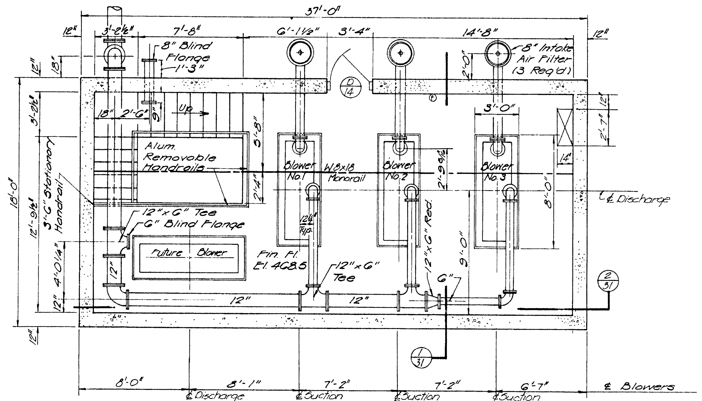
BLOWER FLOOR PLAN Scale: 1/4" = 1'-0"
