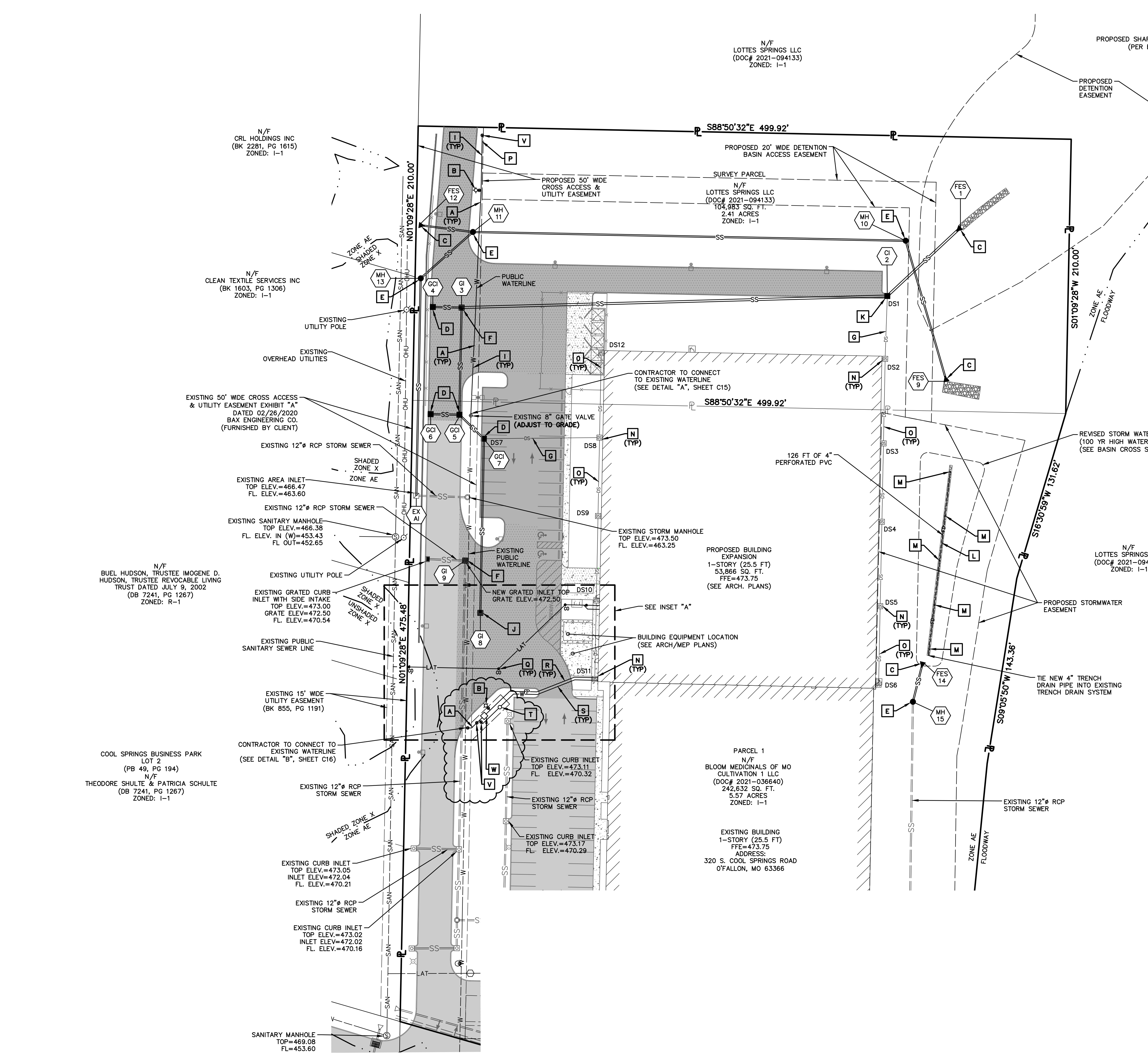
NOTE: SEE COMMERCIAL SERVICE CONNECTION WITH FIRE PROTECTION DETAIL "H" ON SHEET C16. INSET "A" SCALE: 1"=20"
