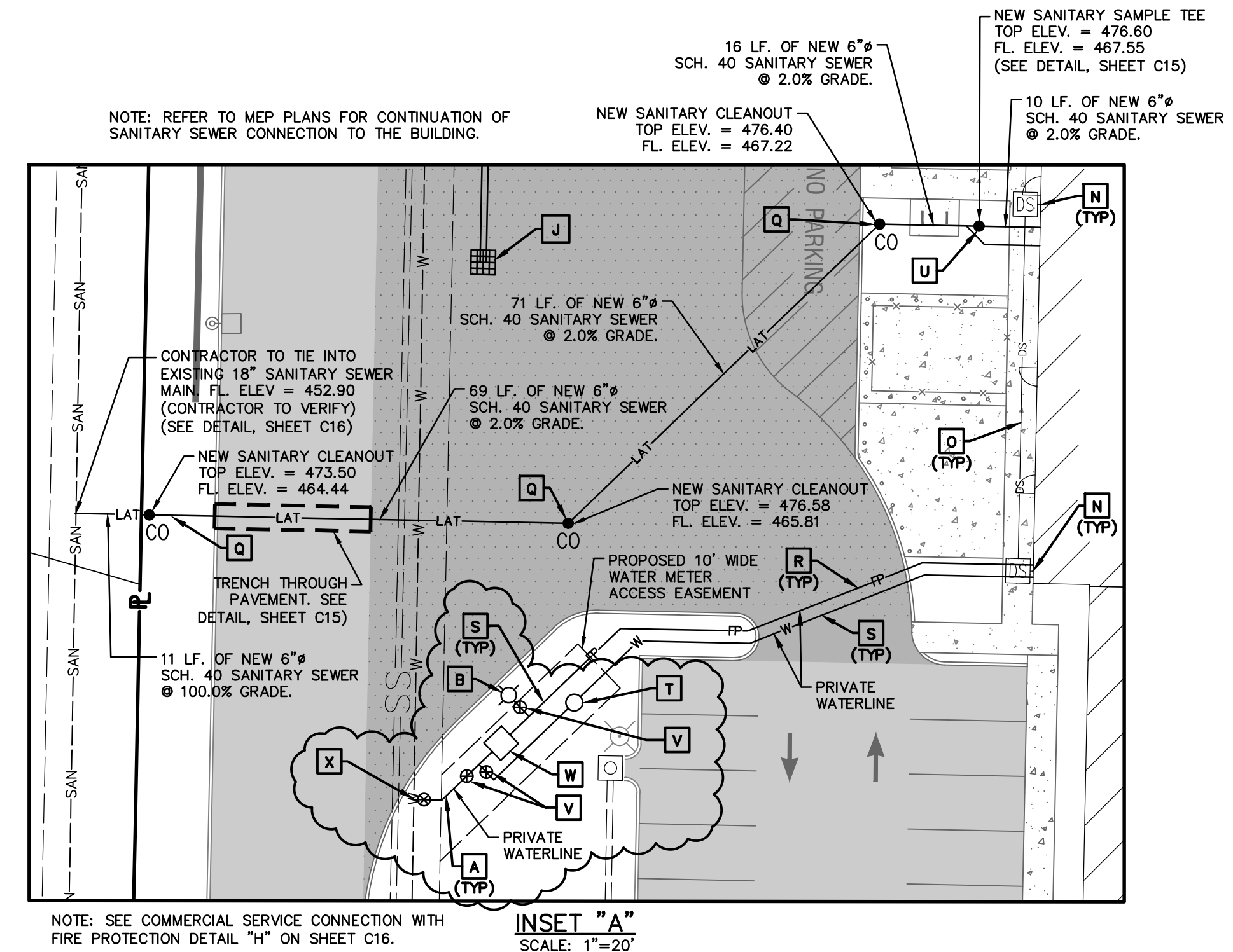
NOTE: SEE COMMERCIAL SERVICE CONNECTION WITH FIRE PROTECTION DETAIL "H" ON SHEET C16. INSET "A" SCALE: 1"=20"
