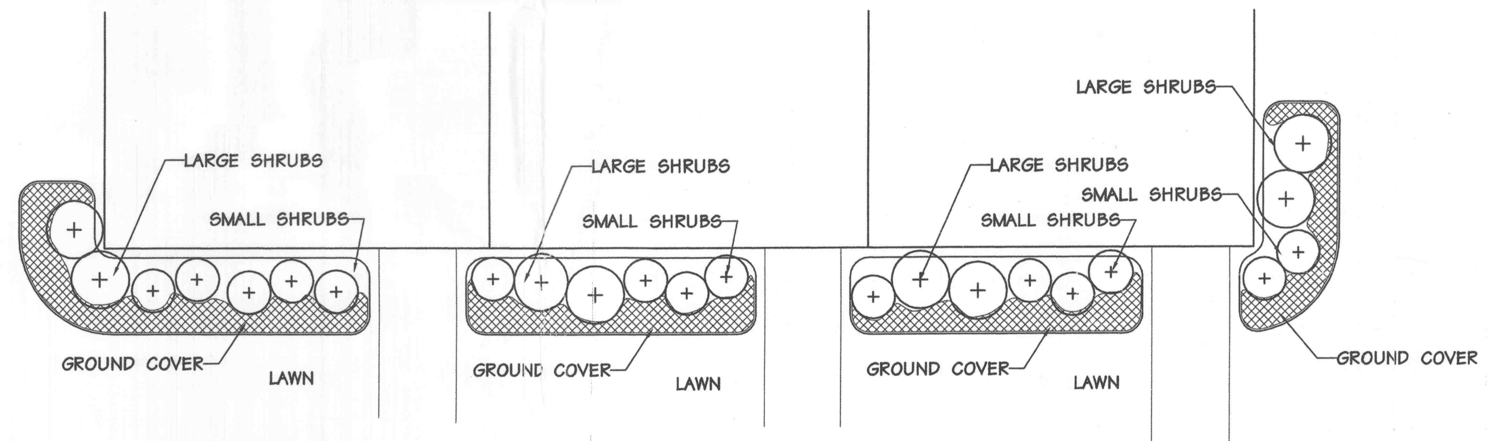
1 PLANTING DETAIL-Typical Building Entries LD-B SCALE 1"=5'
