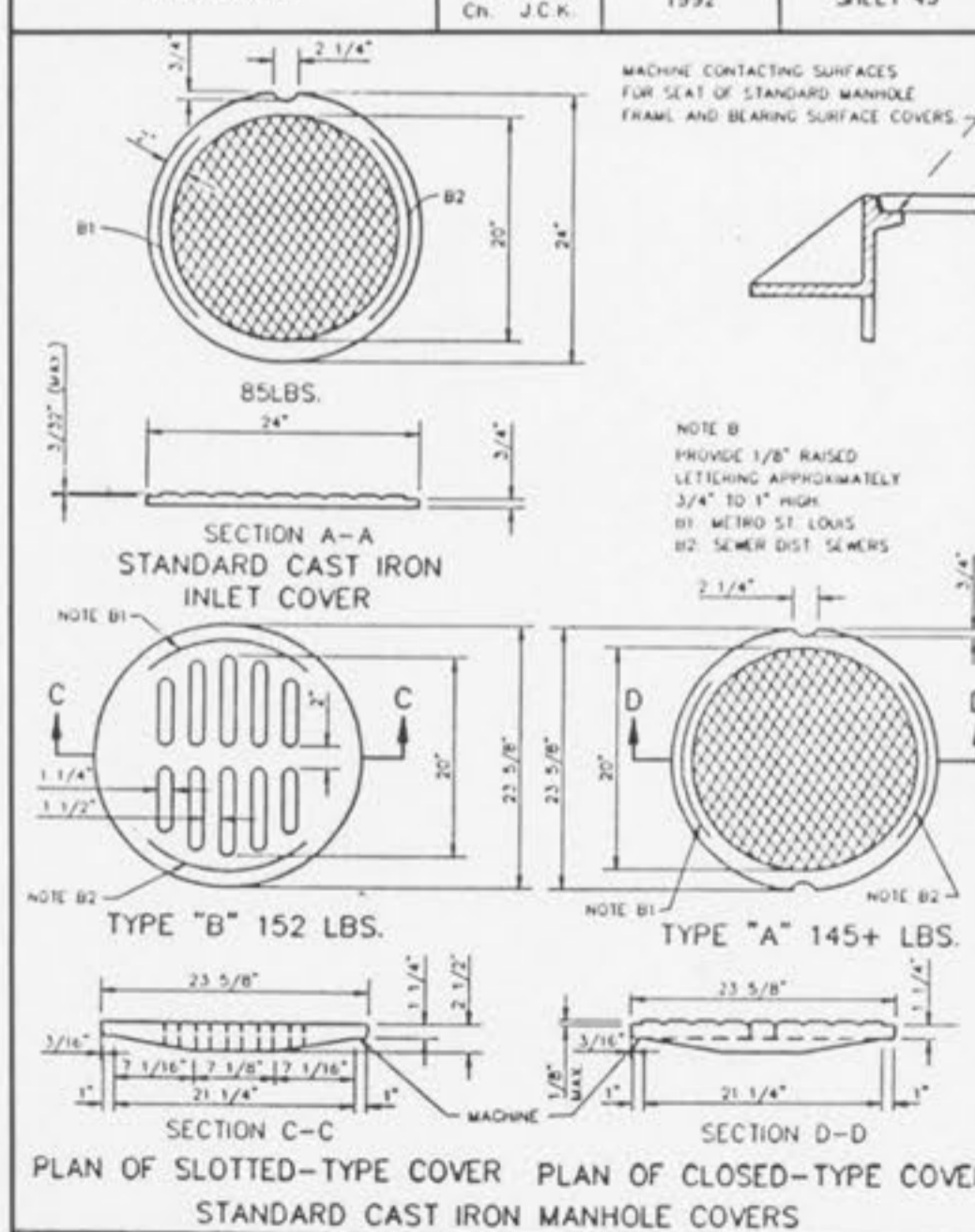
CAST IRON COVERS MANHOLES AND INLETS METROPOLITAN ST. LOUIS SEWER DISTRICT Standard Details of Sewer Construction Dr. R.C.W. Ch. J.C.K. 1992 SHEET 49
