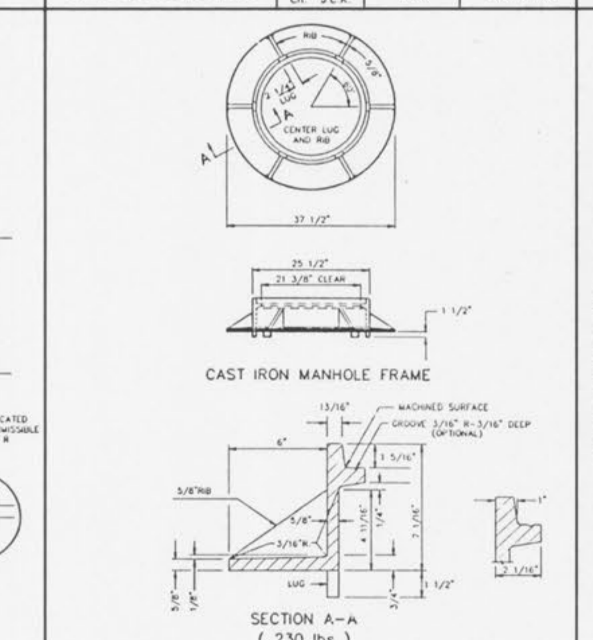
CAST IRON MANHOLE FRAME METROPOLITAN ST. LOUIS SEWER DISTRICT Standard Details of Sewer Construction Dr. D.A.B. Ch. J.C.K. 1992 SHEET 48
