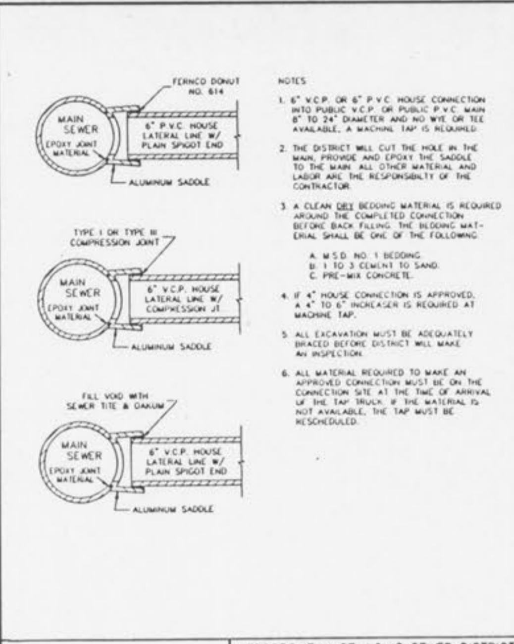
MACHINE TAP METROPOLITAN ST. LOUIS SEWER DISTRICT Standard Details of Sewer Construction Dr. W.S.H. Ch. J.C.K. 1992 SHEET 60
