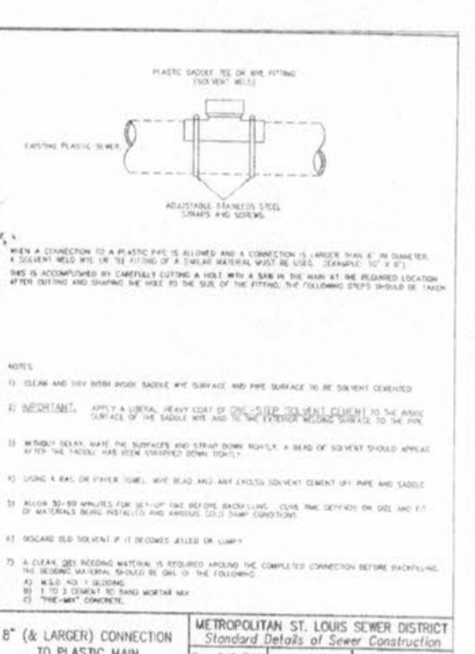
HOUSE CONNECTIONS ALLOWED BY TEE SADDLE METROPOLITAN ST. LOUIS SEWER DISTRICT Standard Details of Sewer Construction D: D.A.B./TEAM Ch. J.C.K. 2000 SHEET 65
