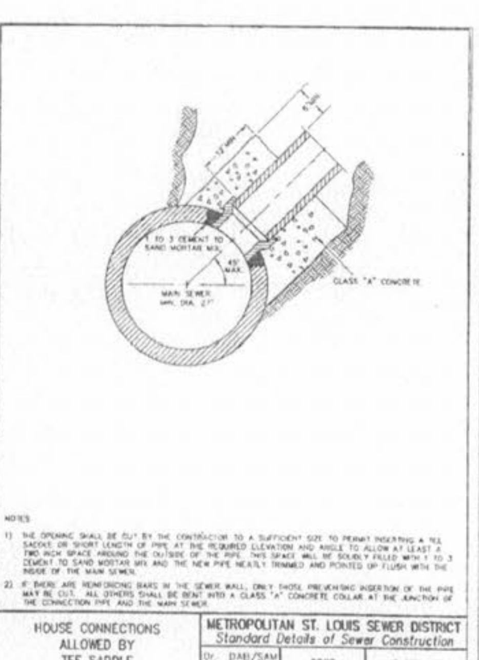
8\"/> METROPOLITAN ST. LOUIS SEWER DISTRICT Standard Details of Sewer Construction D: D.A.B./TEAM Ch. J.C.K. 2000 SHEET 66
