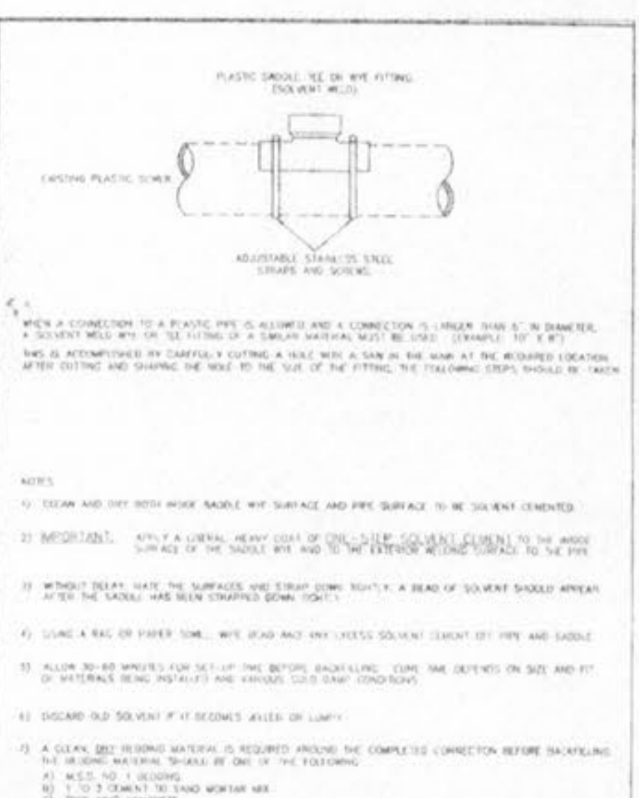
8" (& LARGER) CONNECTION TO PLASTIC MAIN METROPOLITAN ST. LOUIS SEWER DISTRICT Standard Details of Sewer Construction D. W. H. / J. C. K. 2000 SHEET 66
