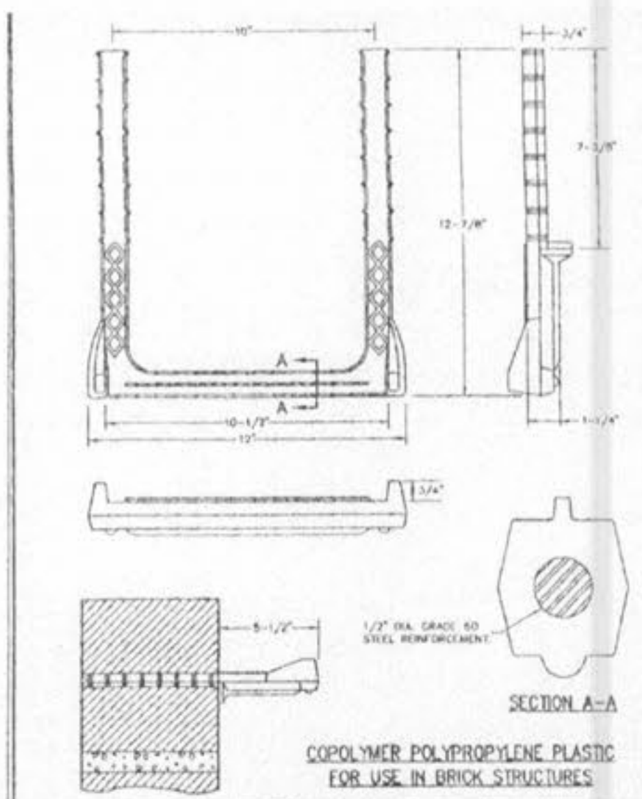
PSI-B MANHOLE STEP INTO JOINT METROPOLITAN ST. LOUIS SEWER DISTRICT Standard Details of Sewer Construction D. W. H. / J. C. K. 2000 SHEET 57
