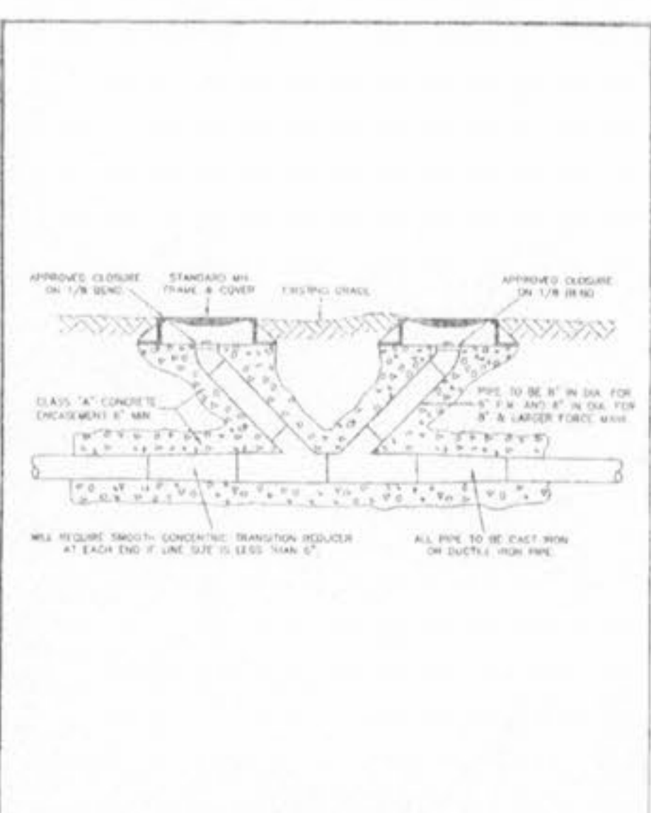
FORCE MAIN CLEANOUT (6" DIA. & SMALLER) METROPOLITAN ST. LOUIS SEWER DISTRICT Standard Details of Sewer Construction D. W. H. / J. C. K. 2000 SHEET 71
