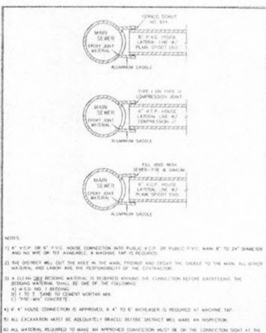
MACHINE TAP METROPOLITAN ST. LOUIS SEWER DISTRICT Standard Details of Sewer Construction D. W. H. / J. C. K. 2000 SHEET 64
