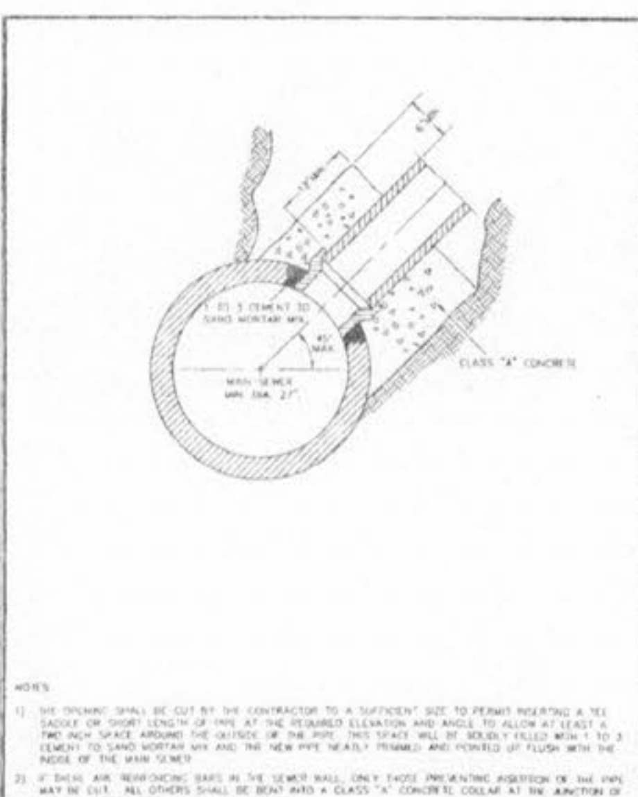
HOUSE CONNECTIONS ALLOWED BY TEE SADDLE METROPOLITAN ST. LOUIS SEWER DISTRICT Standard Details of Sewer Construction D. W. H. / J. C. K. 2000 SHEET 65
