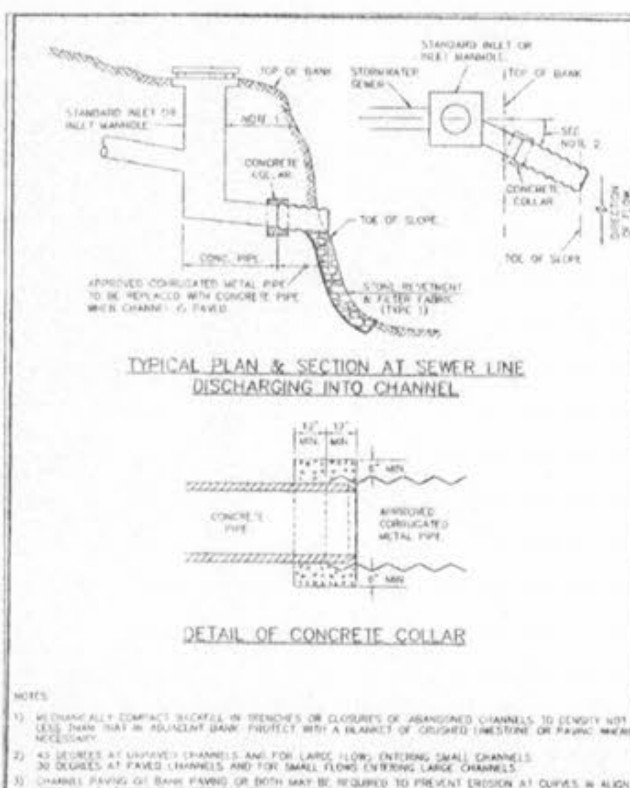
TYPICAL PLAN & SECTION AT SEWER LINE DISCHARGING INTO CHANNEL METROPOLITAN ST. LOUIS SEWER DISTRICT Standard Details of Sewer Construction D. W. H. / J. C. K. 2000 SHEET 62
