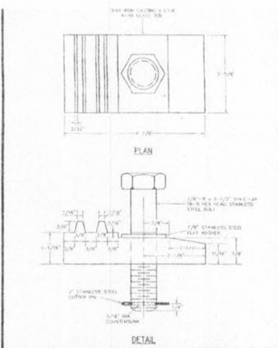
LOCKING DEVICE FOR TYPE "T" LOCK TYPE MANHOLE COVER METROPOLITAN ST. LOUIS SEWER DISTRICT Standard Details of Sewer Construction D. W. H. / J. C. K. 2000 SHEET 55
