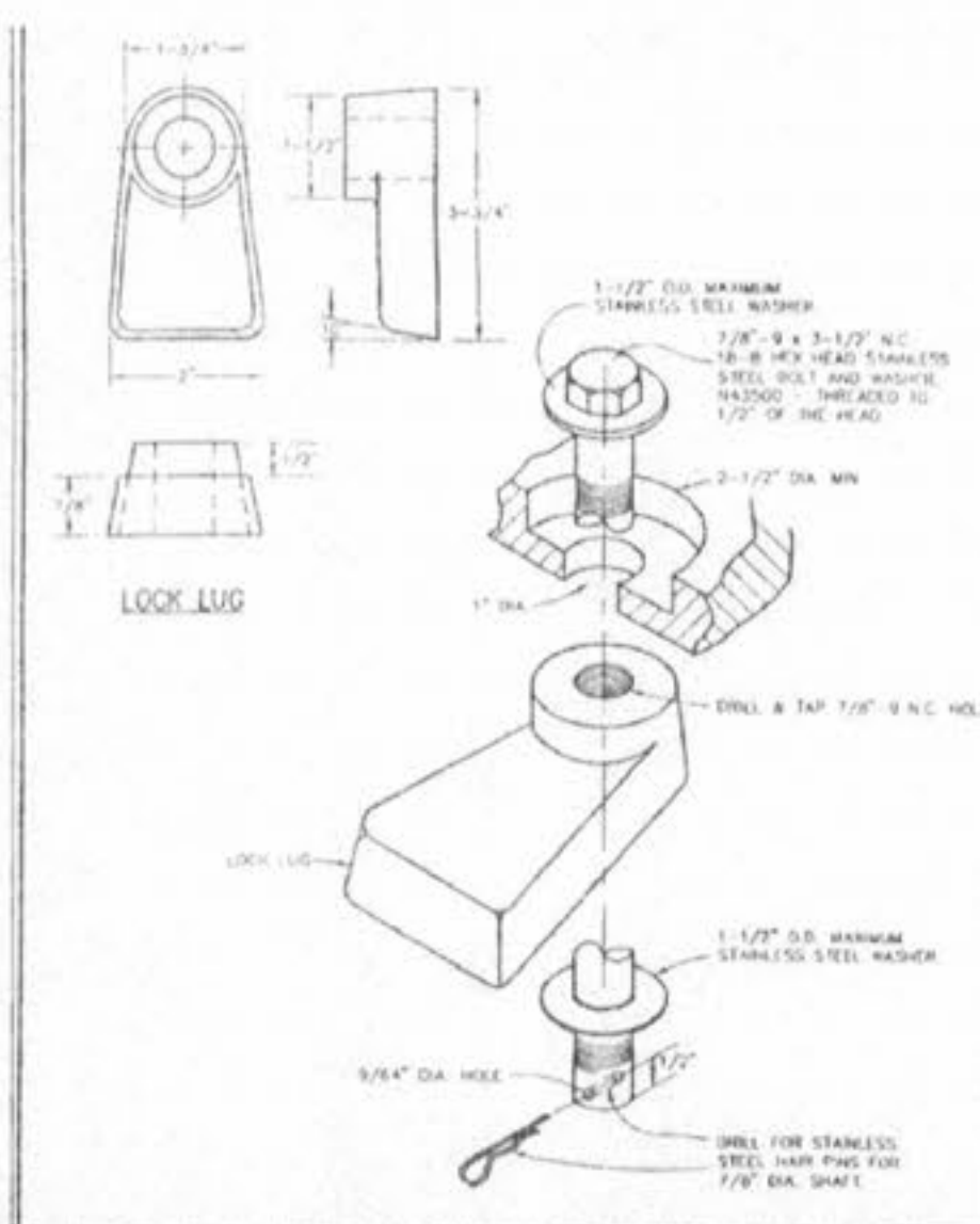
LOCKING DEVICE FOR TYPE "N" LOCK TYPE MANHOLE COVER METROPOLITAN ST. LOUIS SEWER DISTRICT Standard Details of Sewer Construction D. W. H. / J. C. K. 2000 SHEET 56
