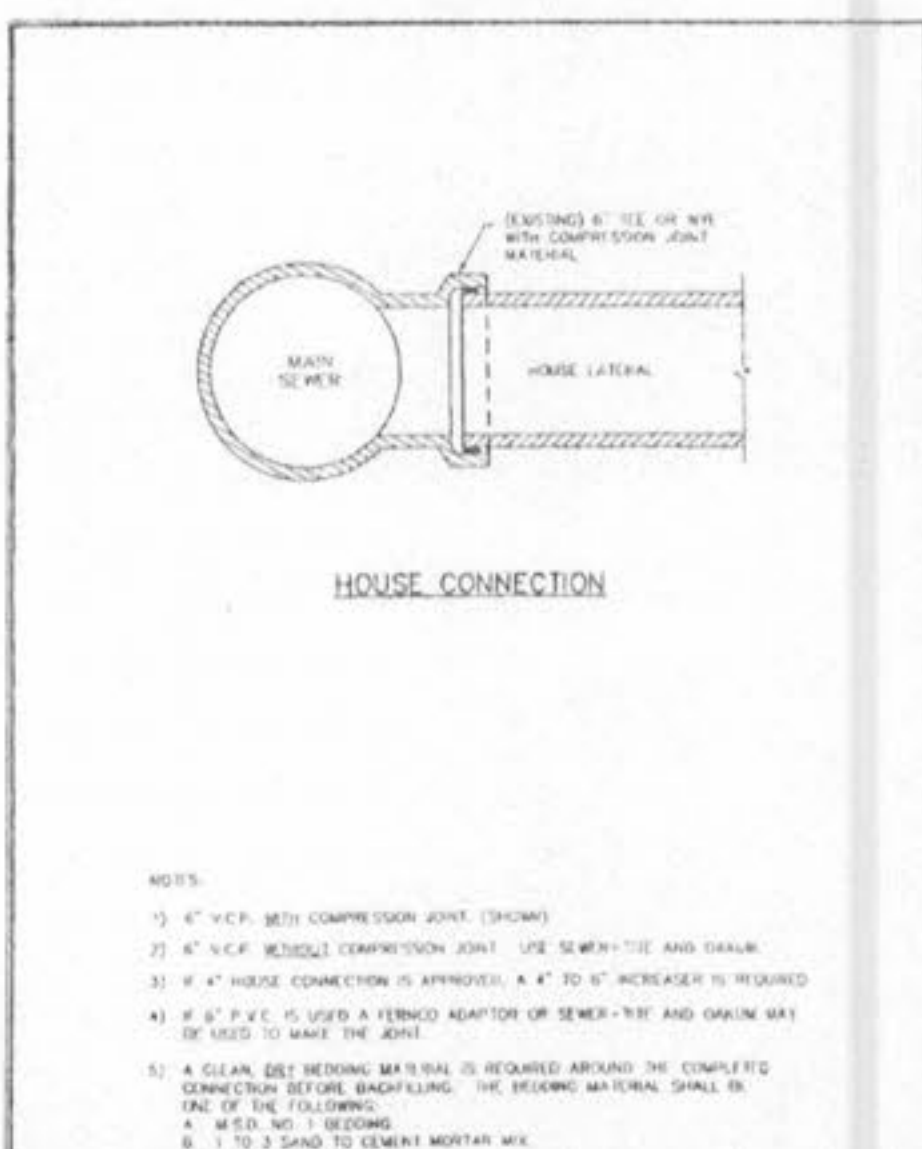
HOUSE CONNECTION METROPOLITAN ST. LOUIS SEWER DISTRICT Standard Details of Sewer Construction D. W. H. / J. C. K. 2000 SHEET 63
