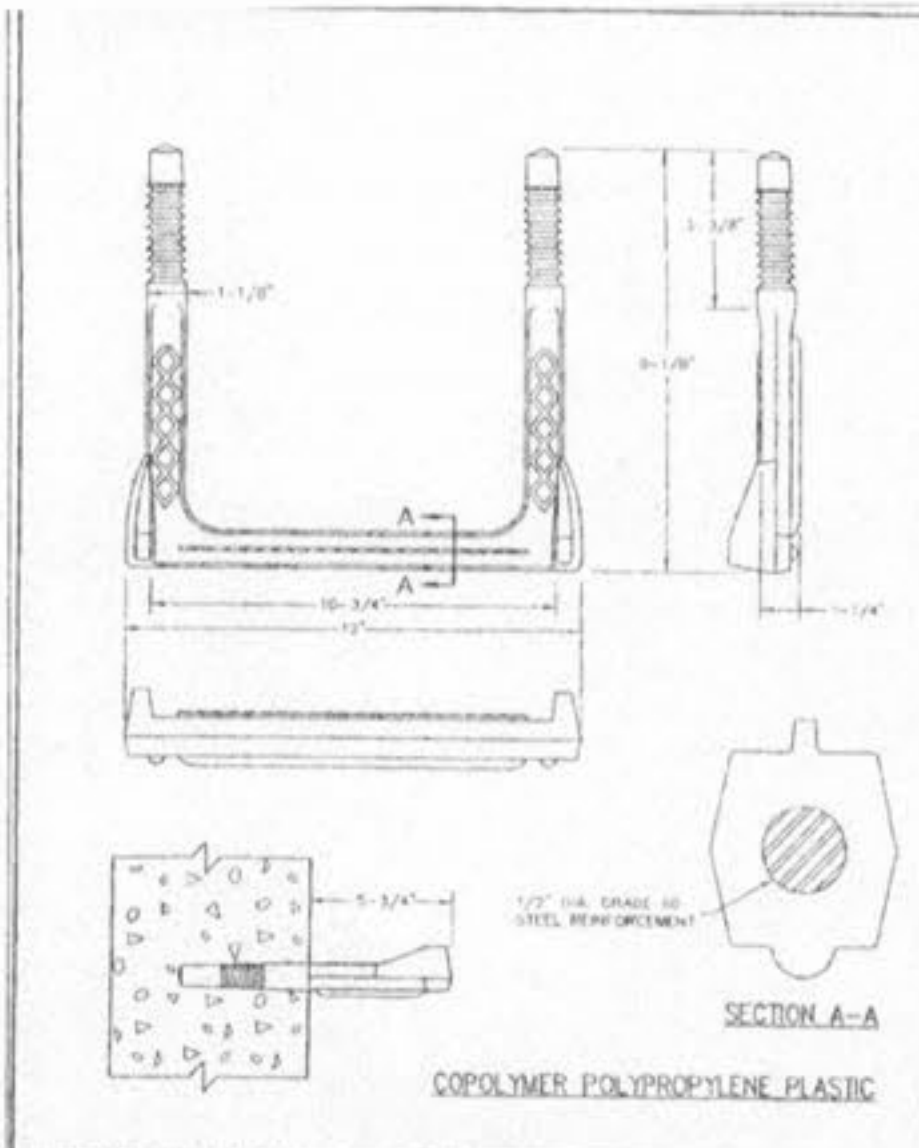
MANHOLE STEP FOR PRECAST & CAST-IN-PLACE MANHOLE METROPOLITAN ST. LOUIS SEWER DISTRICT Standard Details of Sewer Construction D. W. H. / J. C. K. 2000 SHEET 58
