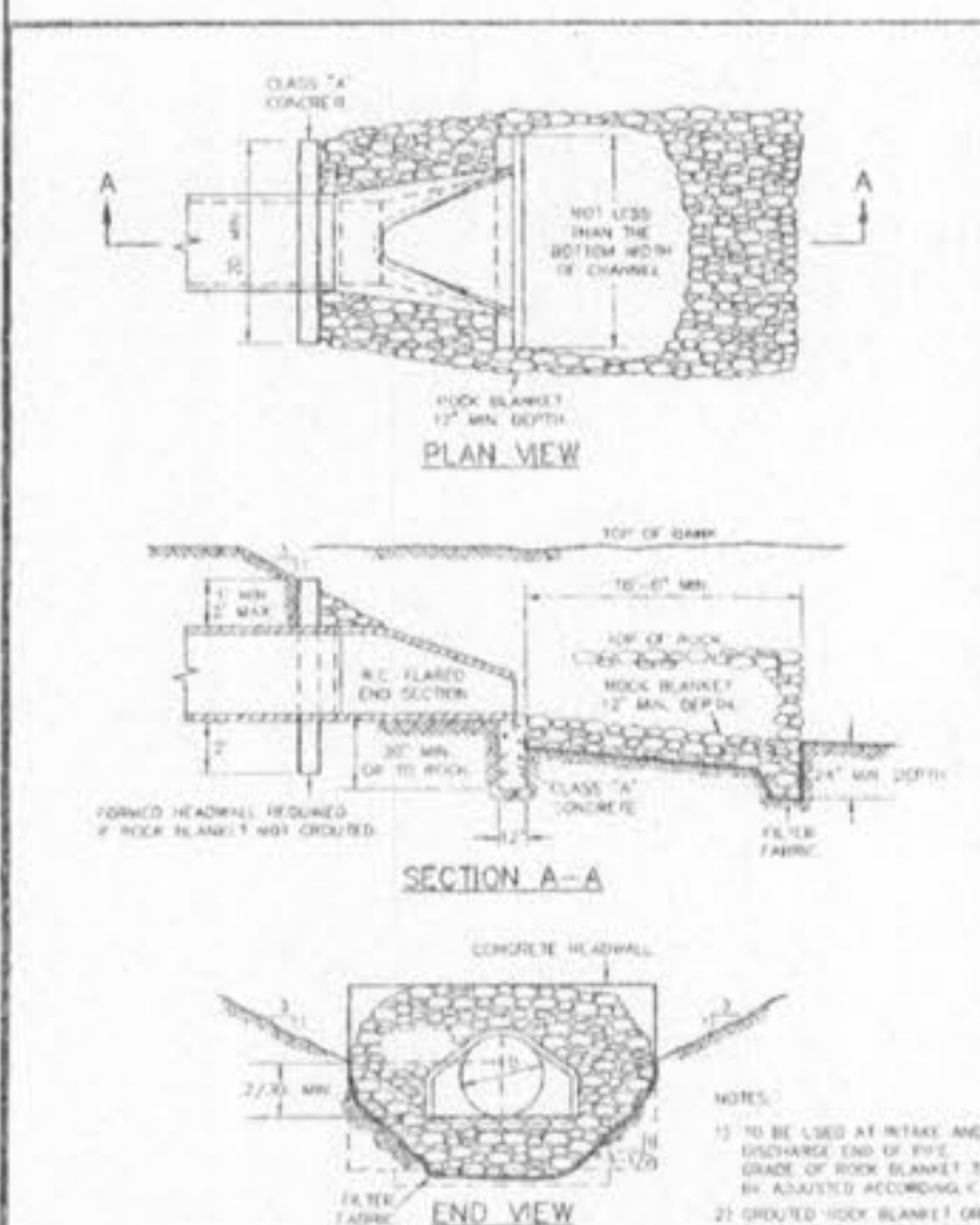
FLARED END SECTION METROPOLITAN ST. LOUIS SEWER DISTRICT Standard Details of Sewer Construction D. W. H. / J. C. K. 2000 SHEET 61
