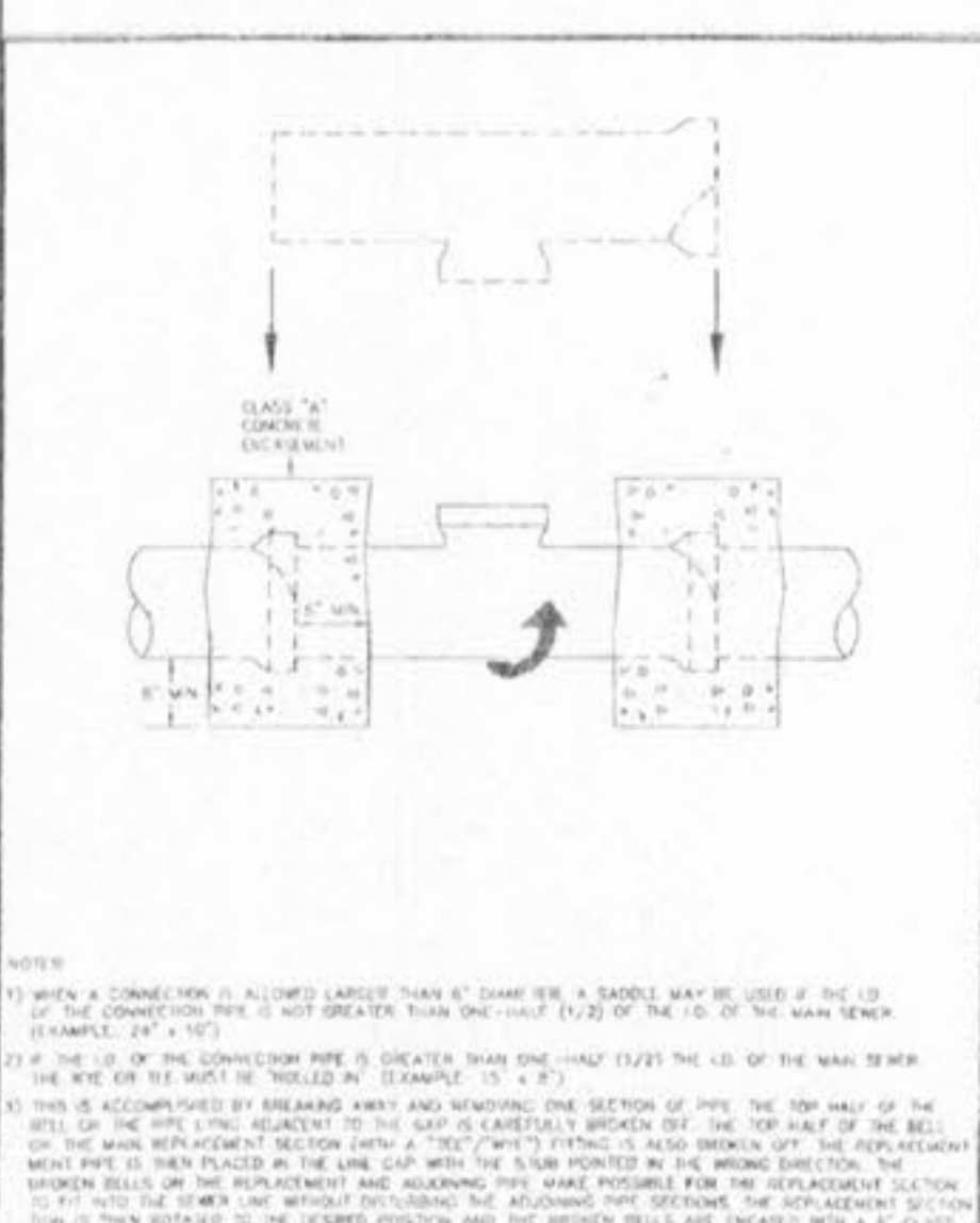
"ROLL-IN" (FOR EXISTING CLAY OR CONCRETE PIPE) METROPOLITAN ST. LOUIS SEWER DISTRICT Standard Details of Sewer Construction D. W. H. / J. C. K. 2000 SHEET 67
