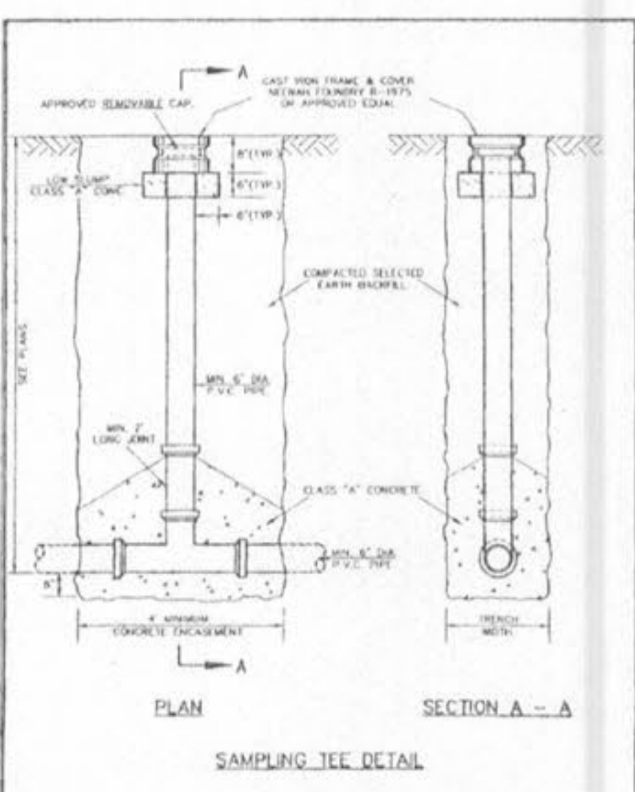
SAMPLING TEE METROPOLITAN ST. LOUIS SEWER DISTRICT Standard Details of Sewer Construction D. W. H. / J. C. K. 2000 SHEET 69
