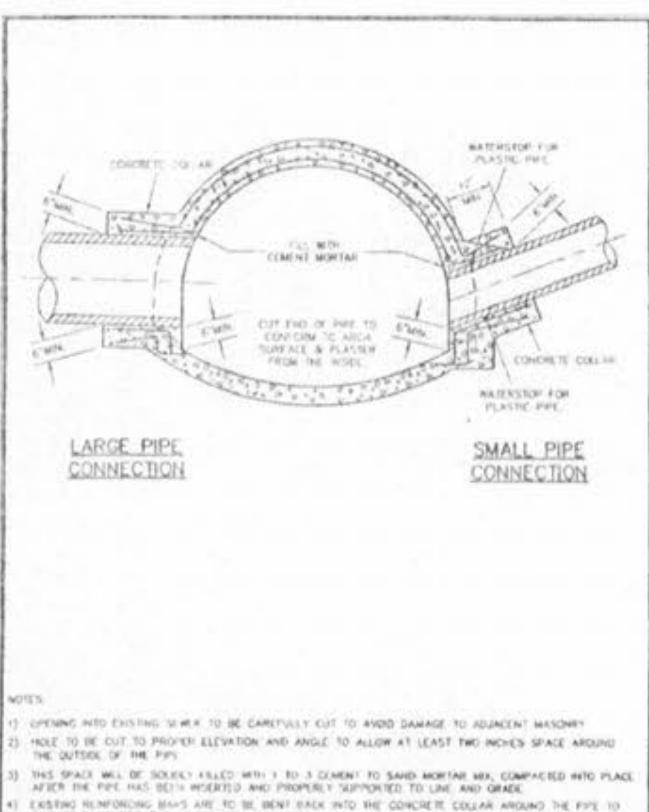
CONNECTIONS TO LARGE SEWERS METROPOLITAN ST. LOUIS SEWER DISTRICT Standard Details of Sewer Construction D. W. H. / J. C. K. 2000 SHEET 68
