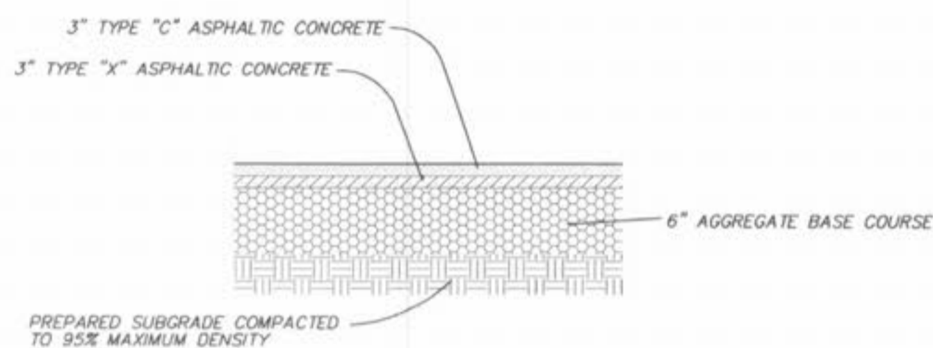
TYPICAL PAVEMENT SECTION N.T.S.
