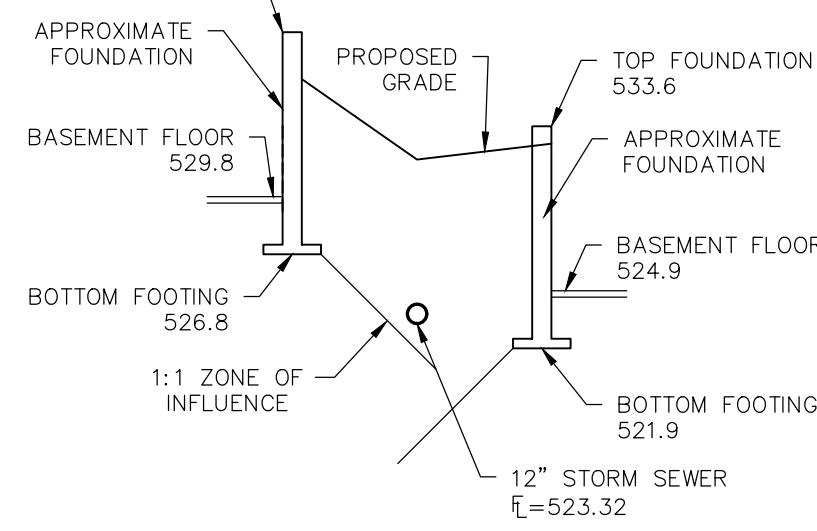
ZONE OF INFLUENCE SECTION 9-9 Scale: 1" = 10'
