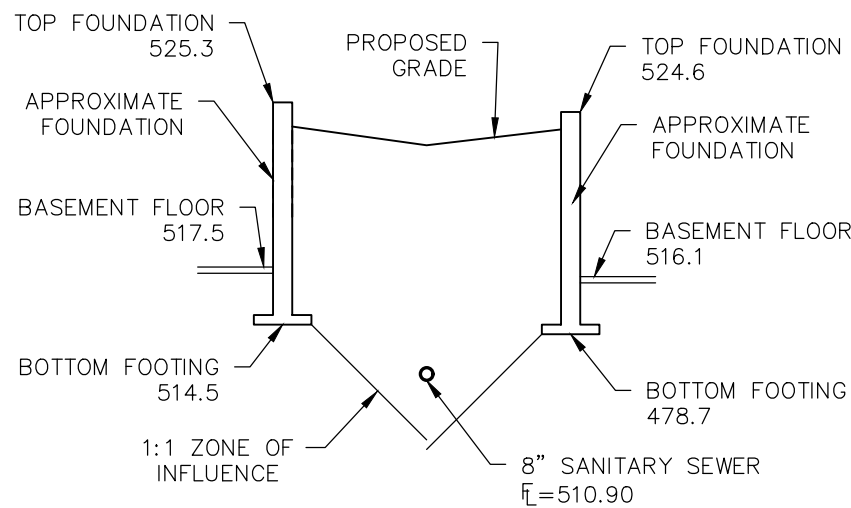
ZONE OF INFLUENCE SECTION 2-2 Scale: 1" = 10'
