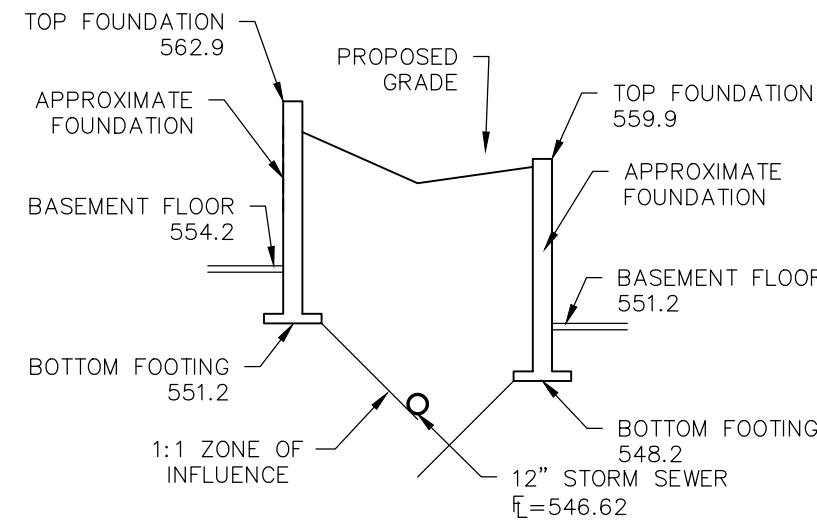
ZONE OF INFLUENCE SECTION 10-10 Scale: 1" = 10'
