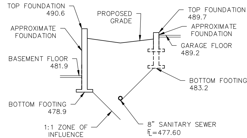
ZONE OF INFLUENCE SECTION 1-1 Scale: 1" = 10'
