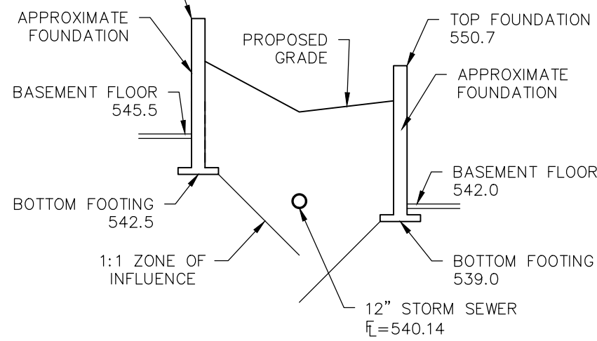
ZONE OF INFLUENCE SECTION 7-7 Scale: 1" = 10'
