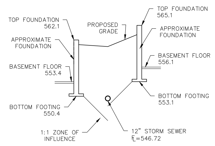
ZONE OF INFLUENCE SECTION 12-12 Scale: 1" = 10'
