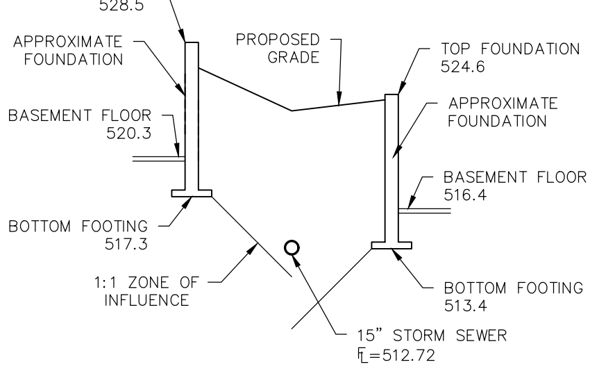
ZONE OF INFLUENCE SECTION 8-8 Scale: 1" = 10'
