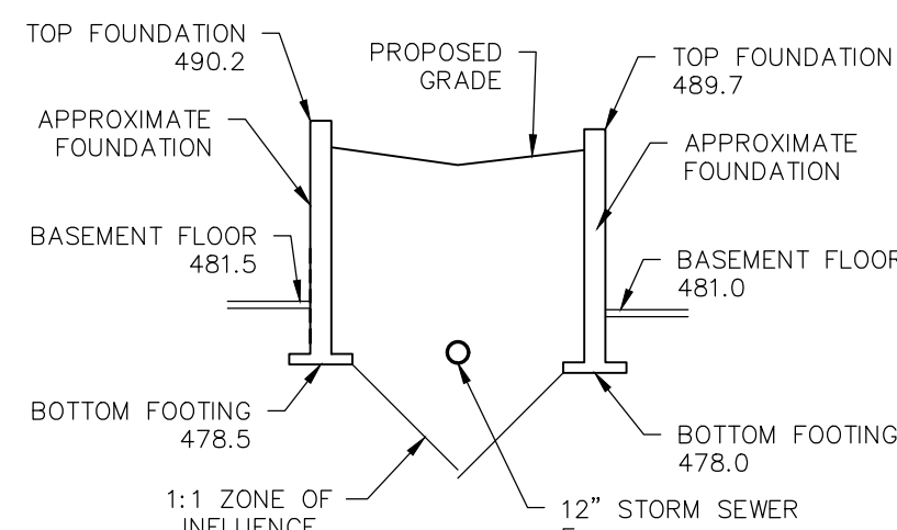
ZONE OF INFLUENCE SECTION 4-4 Scale: 1" = 10'
