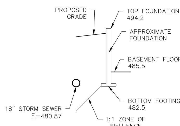
ZONE OF INFLUENCE SECTION 5-5 Scale: 1" = 10'
