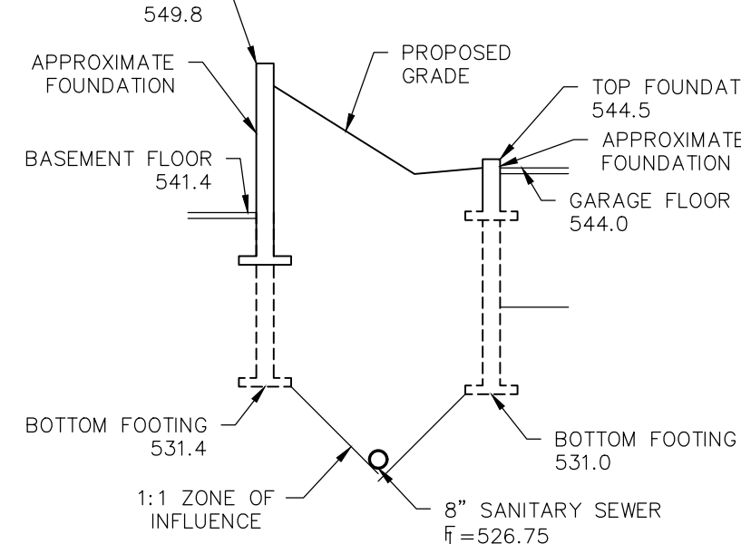
ZONE OF INFLUENCE SECTION 14-14 Scale: 1" = 10'
