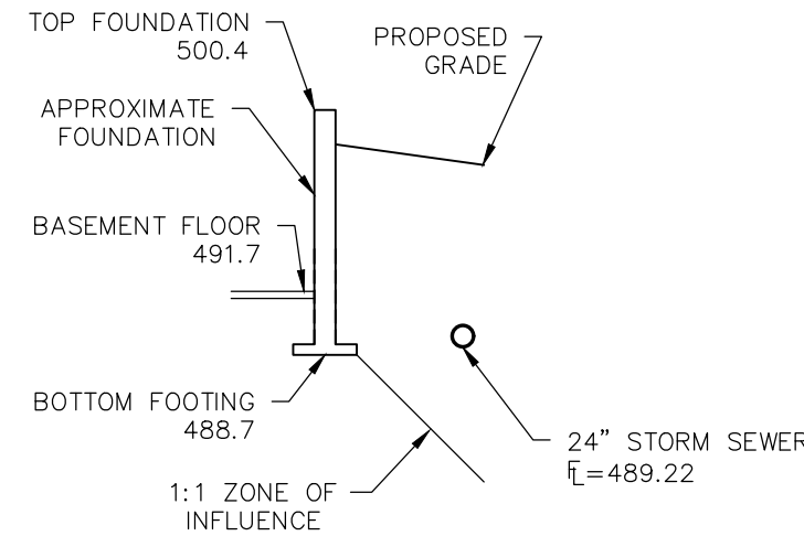
ZONE OF INFLUENCE SECTION 6-6 Scale: 1" = 10'
