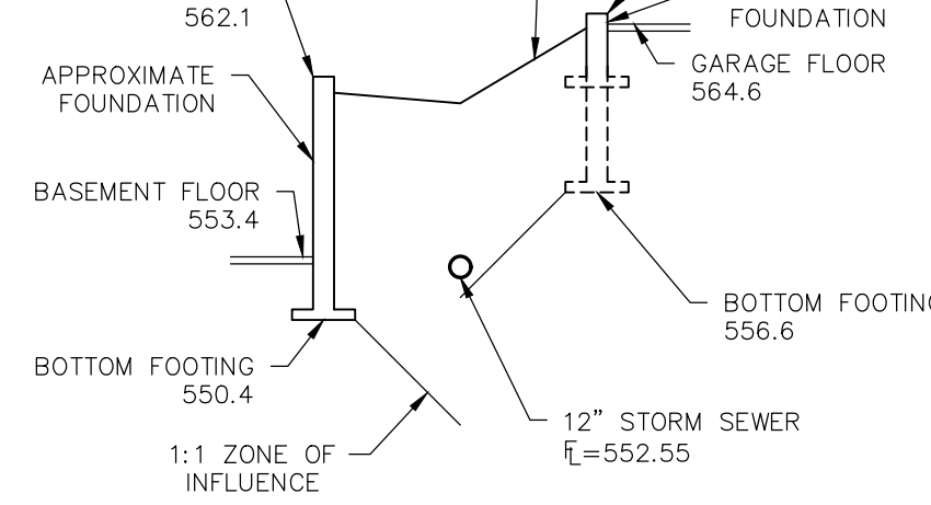
ZONE OF INFLUENCE SECTION 13-13 Scale: 1" = 10'
