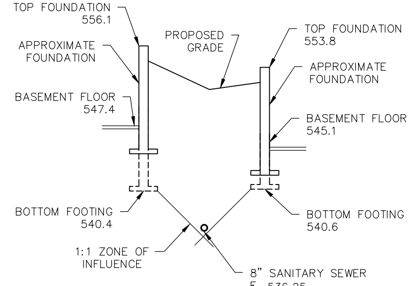
ZONE OF INFLUENCE SECTION 3-3 Scale: 1" = 10'
