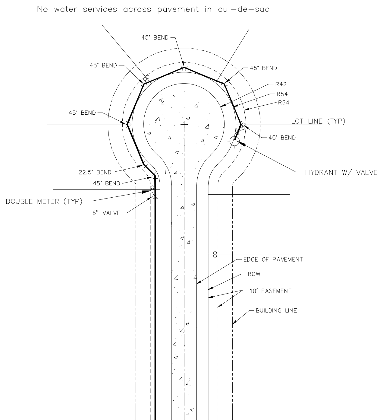
SMALL COURT DETAIL NOT TO SCALE DETAIL "T" PAGE 1 OF 2
