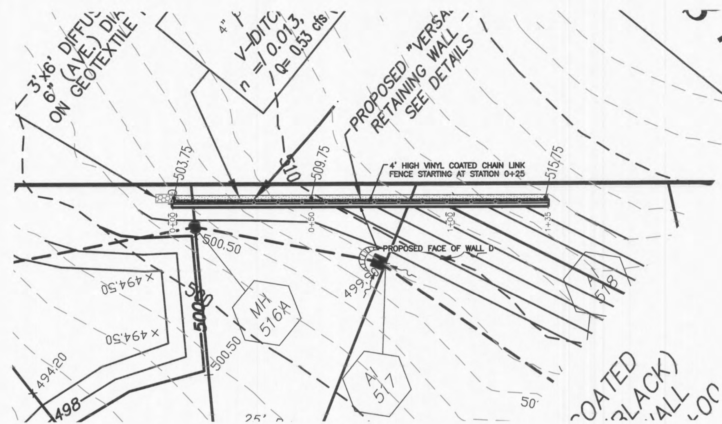
PLAN VIEW - WALL D SCALE 1"=20'
