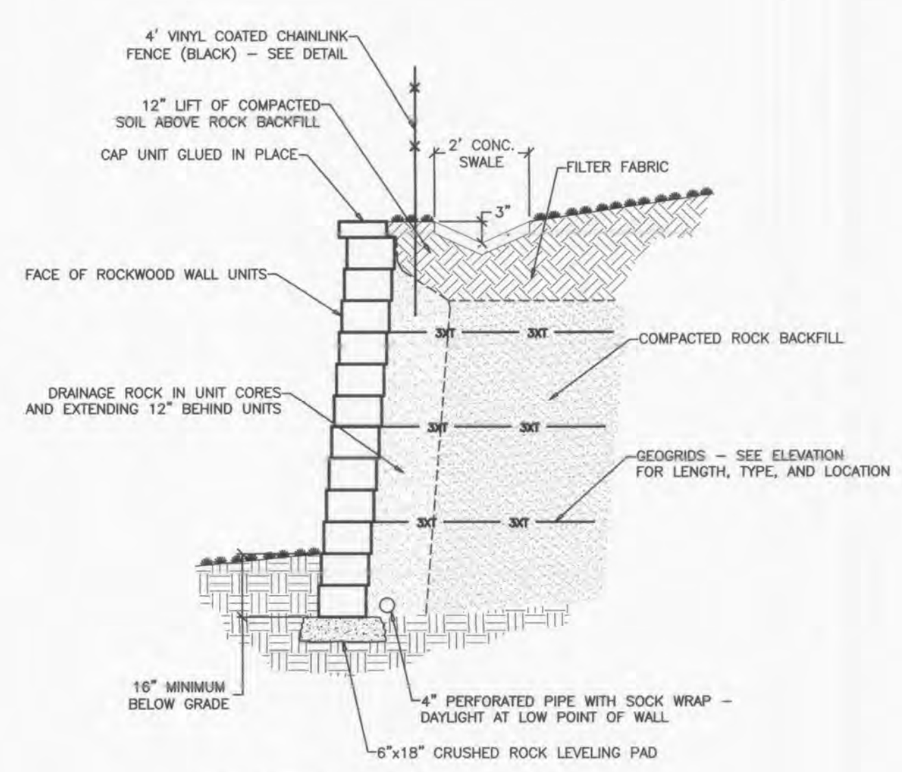
TYPICAL SECTION - WALL D NOT TO SCALE
