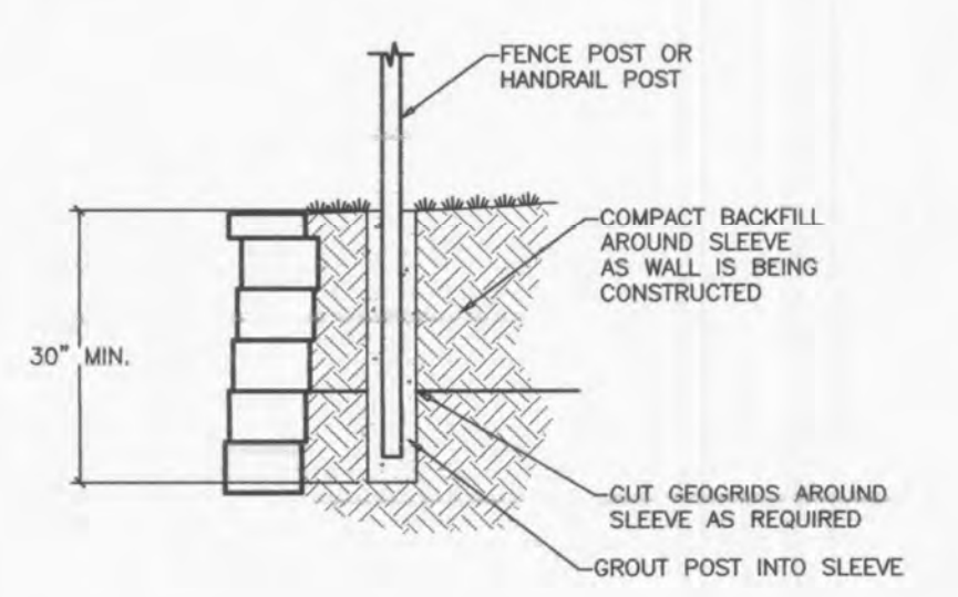
FENCE DETAIL NOT TO SCALE
