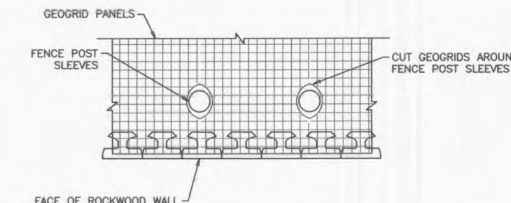
FENCE SLEEVE DETAIL NOT TO SCALE
