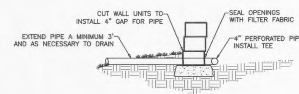
PERFORATED PIPE OUTLET NOT TO SCALE
