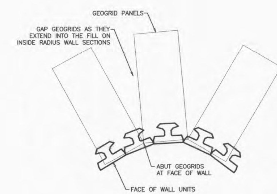
INSIDE RADIUS DETAIL NOT TO SCALE
