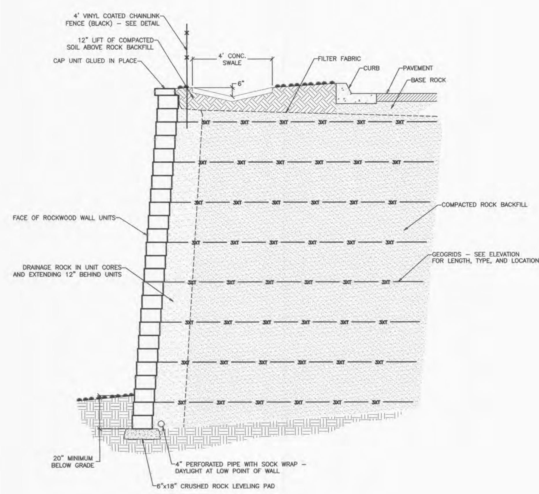
TYPICAL SECTION - WALL C NOT TO SCALE
