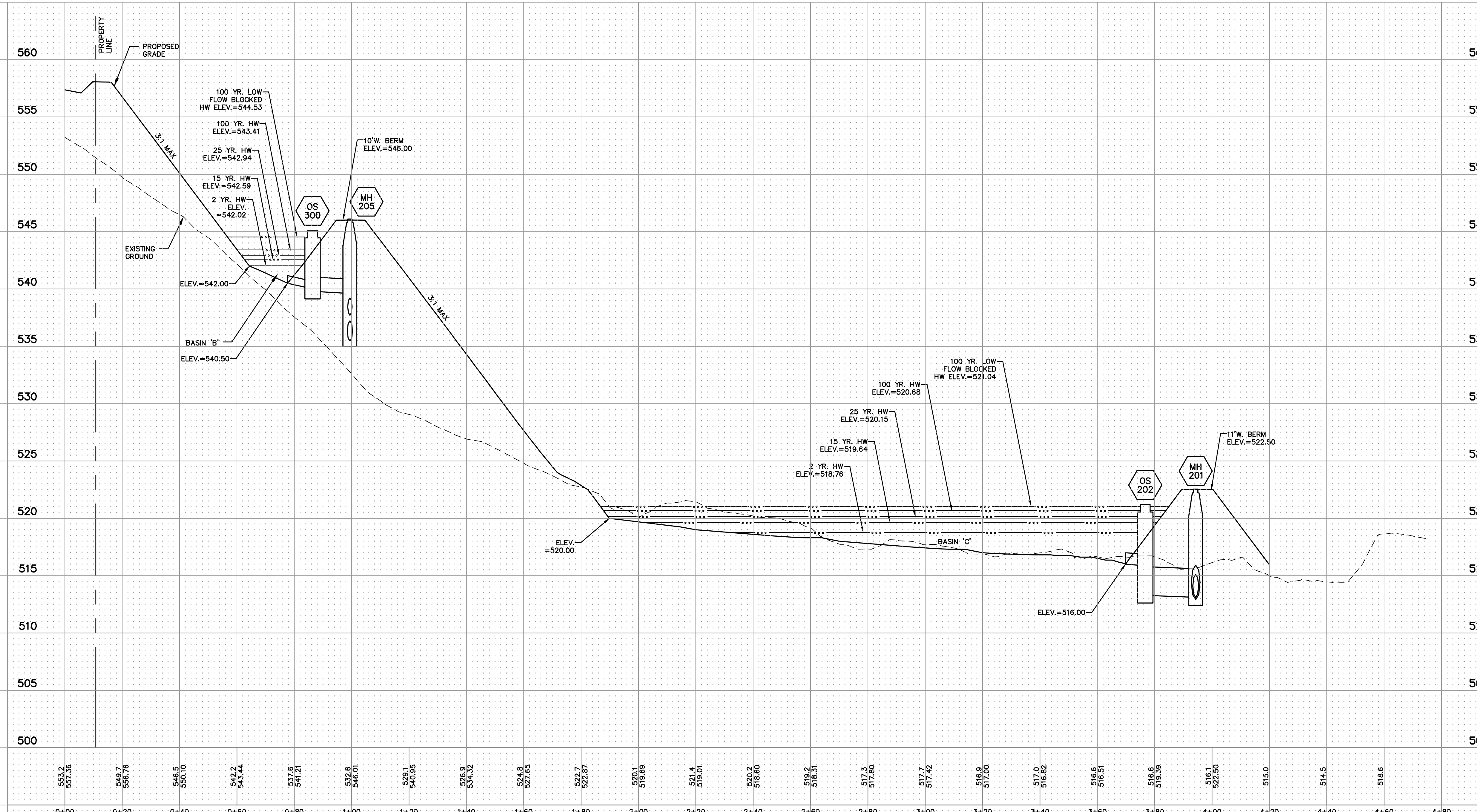
BASIN SECTION 1-1
