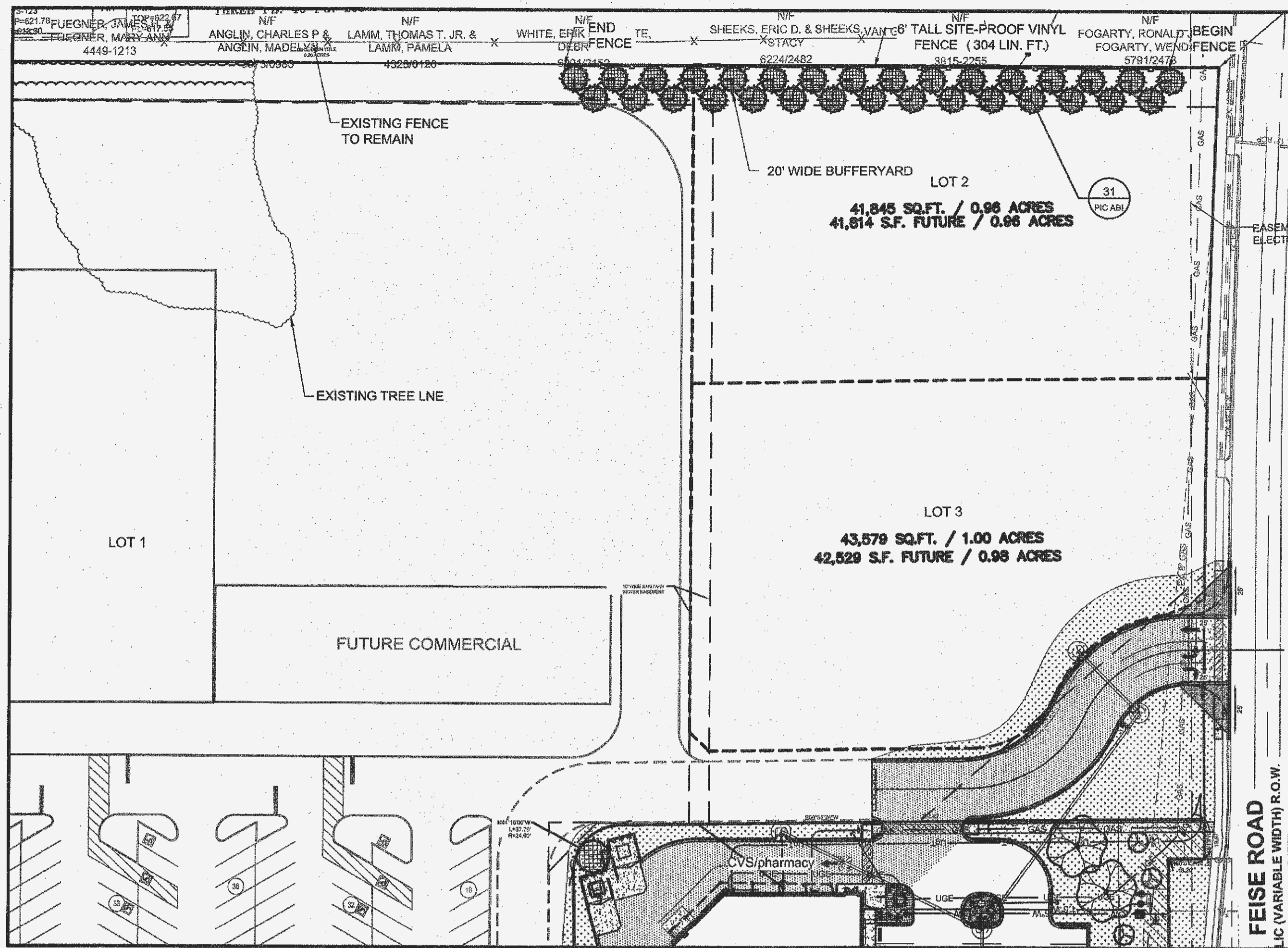
OFFSITE BUFFERYARD PLANTING MAP 1" = 50'
