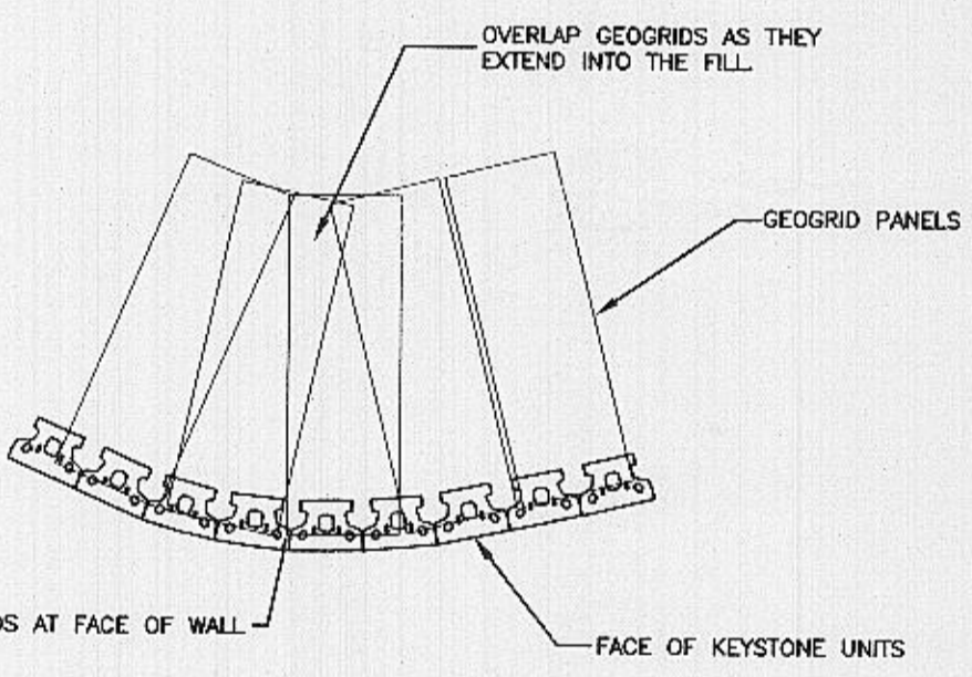
OUTSIDE RADIUS DETAIL NOT TO SCALE
