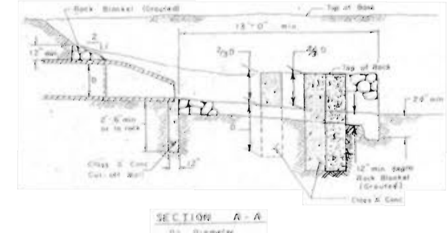
Flared End Section with Energy Dissipator
