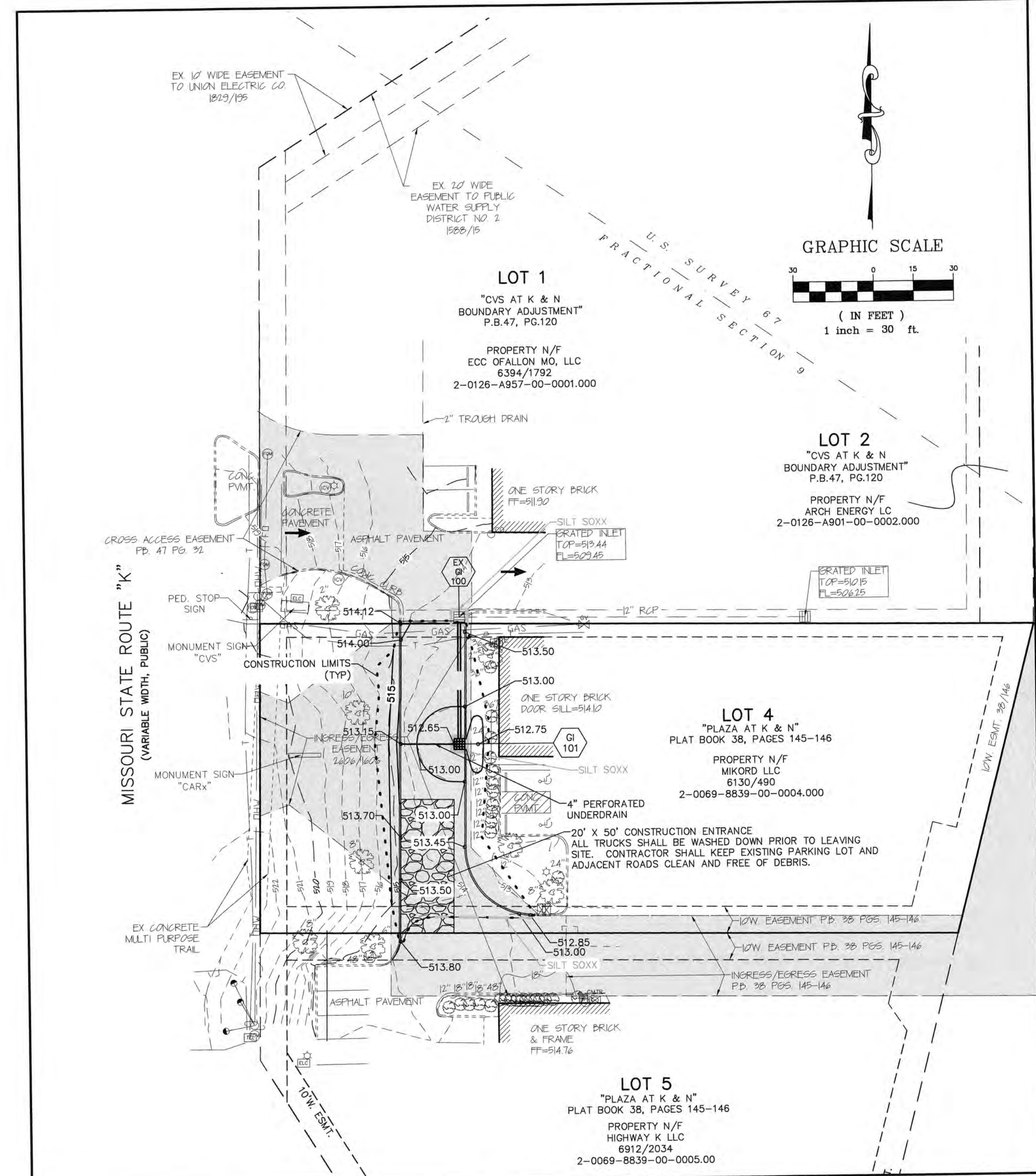
Grading Plan
