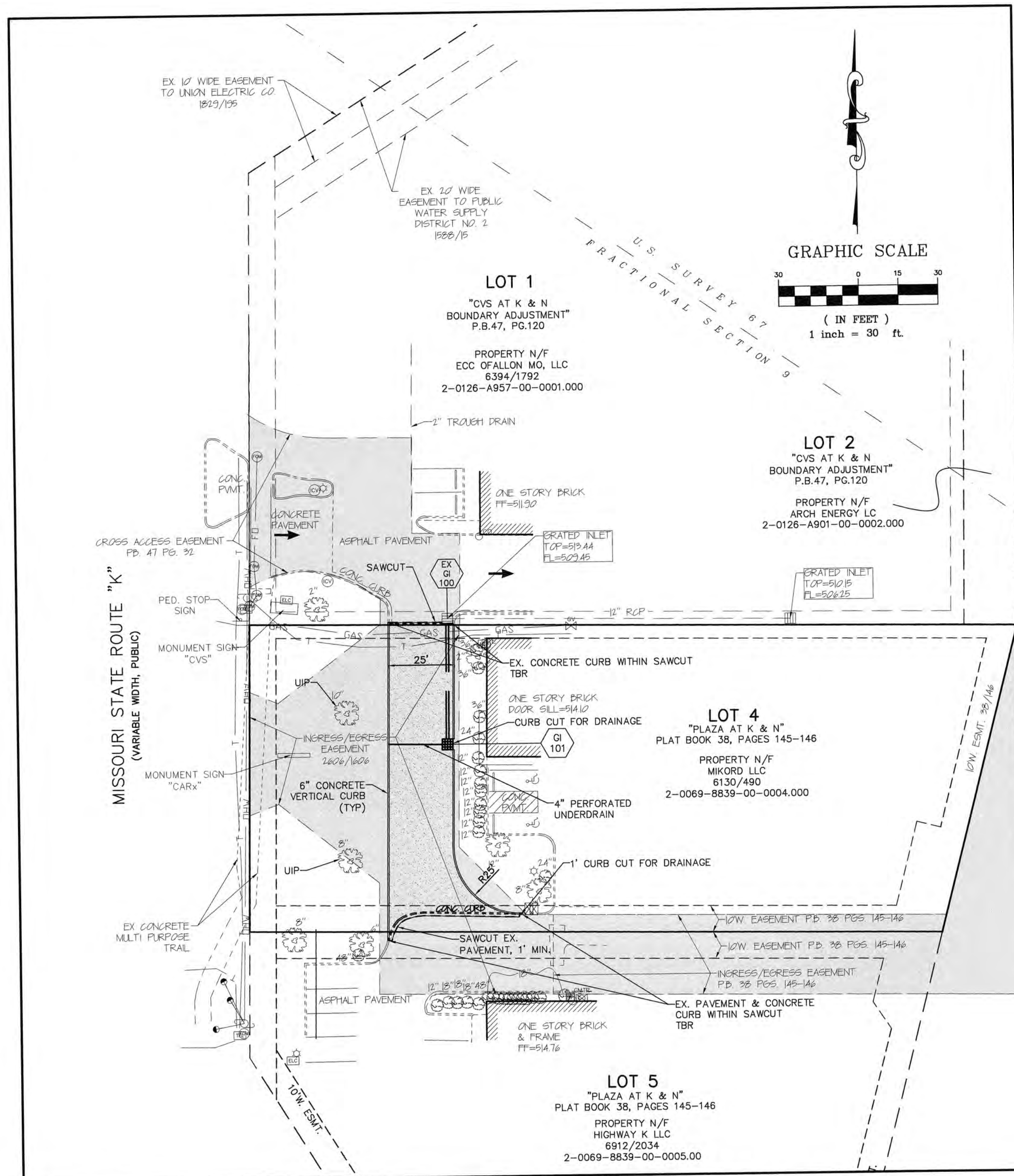
Site Plan
