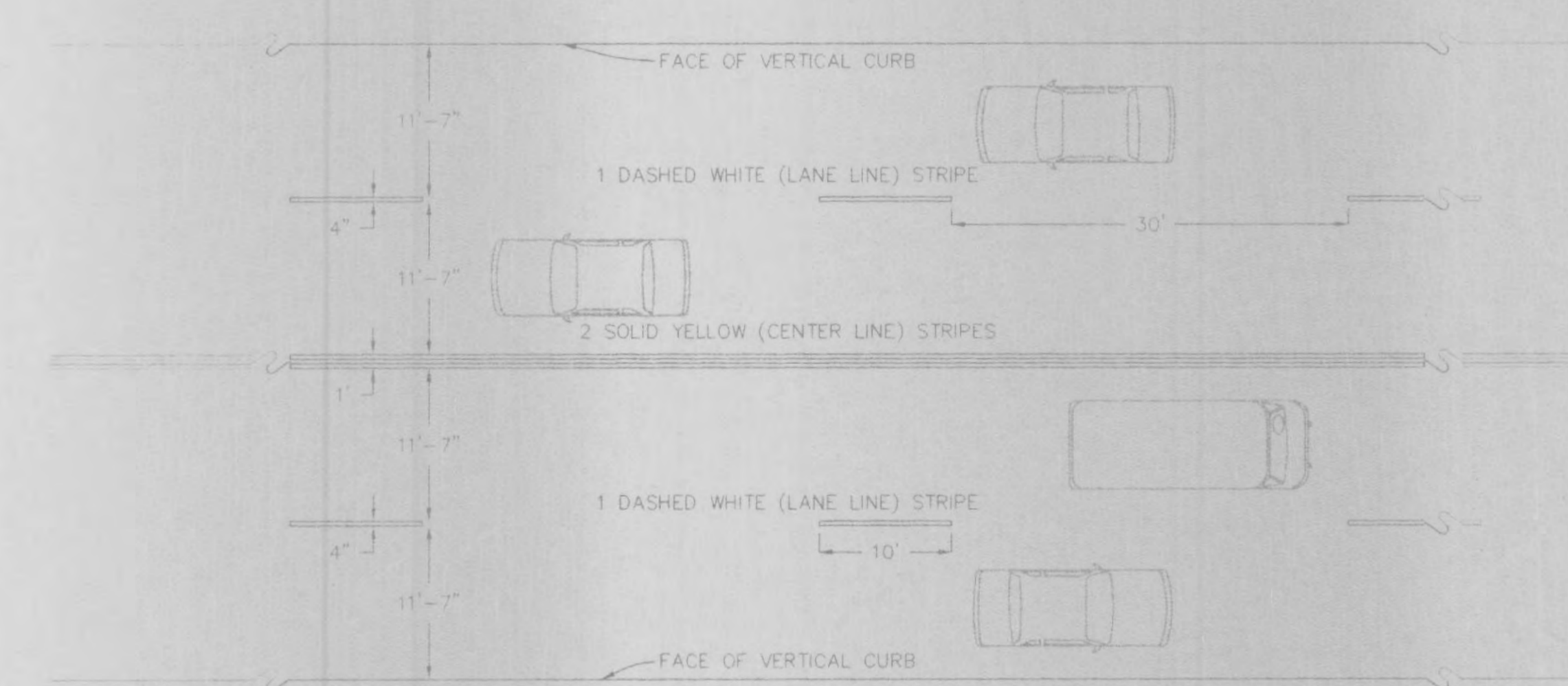
LANE STRIPING DETAIL SCALE: 1" = 10'
