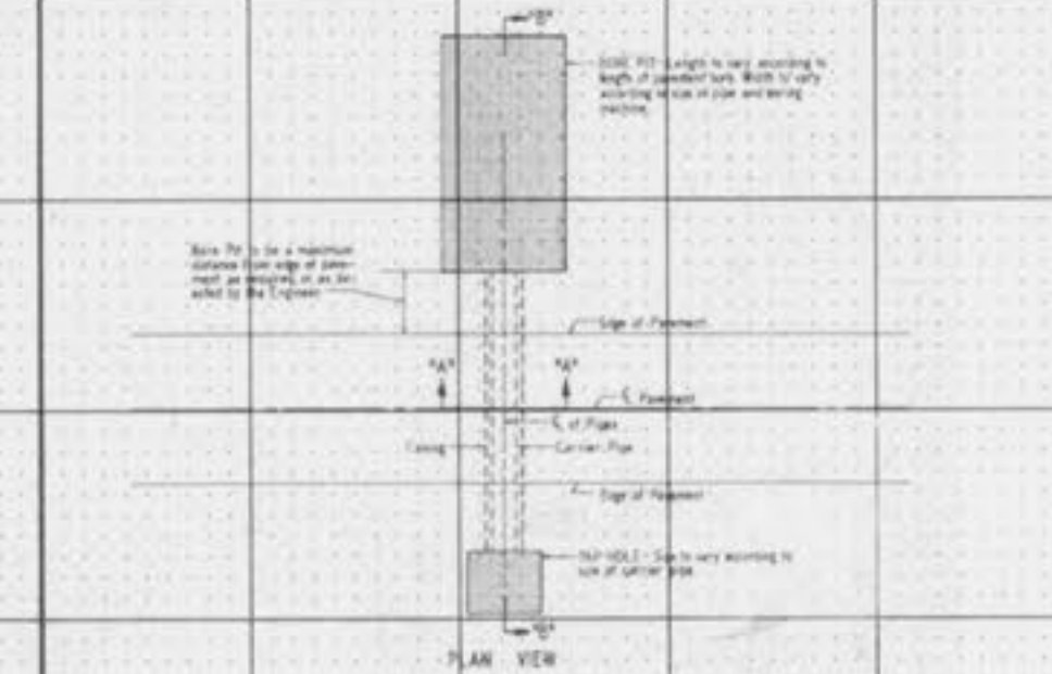
METROPOLITAN ST. LOUIS SEWER DISTRICT Standard Details of Sewer Construction Dr. W.S.H. Ch. J.C.K. 1992 SHEET 5
