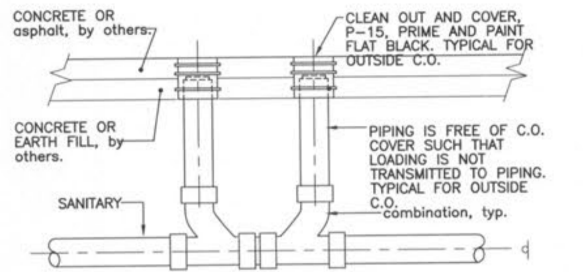
26 DOUBLE SANITARY CLEANOUT SCALE: NONE
